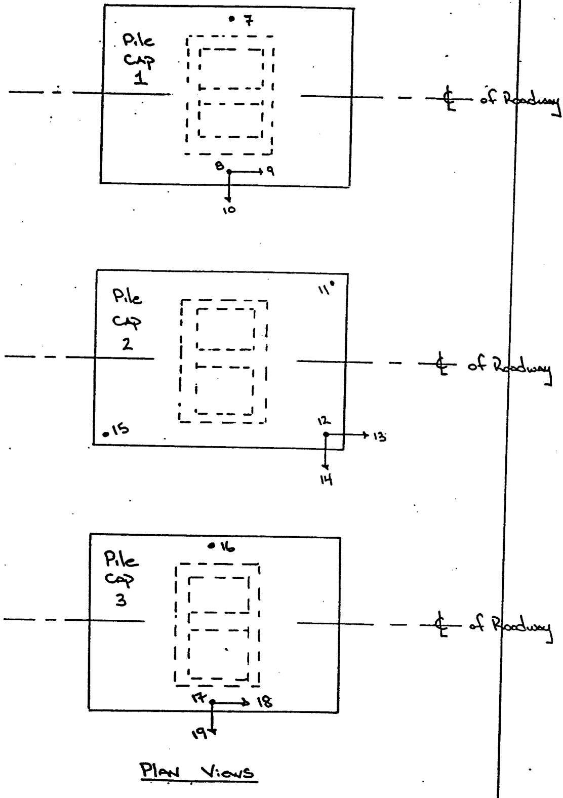
Figure 22. Kealakaha Bridge Support Seismic Instrument Locations (Plan View).
