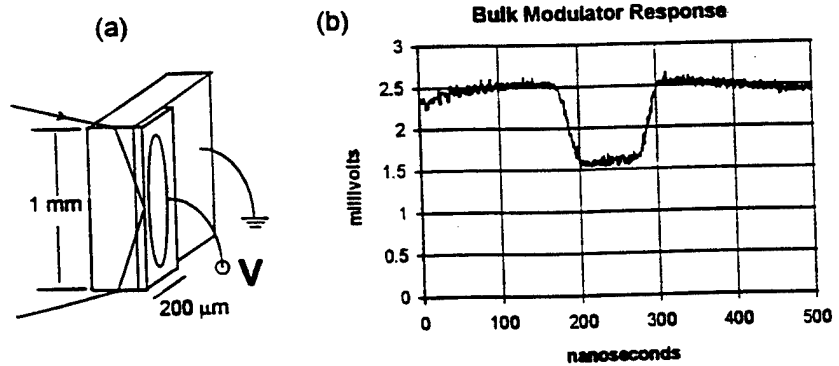
Figure 5. (a) Coupling of laser light into modular at Brewster's angle on the cleaved edge. (b) The modulation response from application of a 20 Volt square wave.
