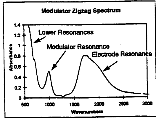
Figure 3. Spectrum of modulator and electrode quantum wells, showing losses from electrodes.
