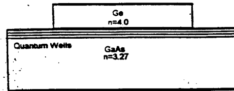
Figure 6. A 2 μm high Ge waveguide confines 10 μm light with evanescent coupling to the active 1 μm thick QWs.
