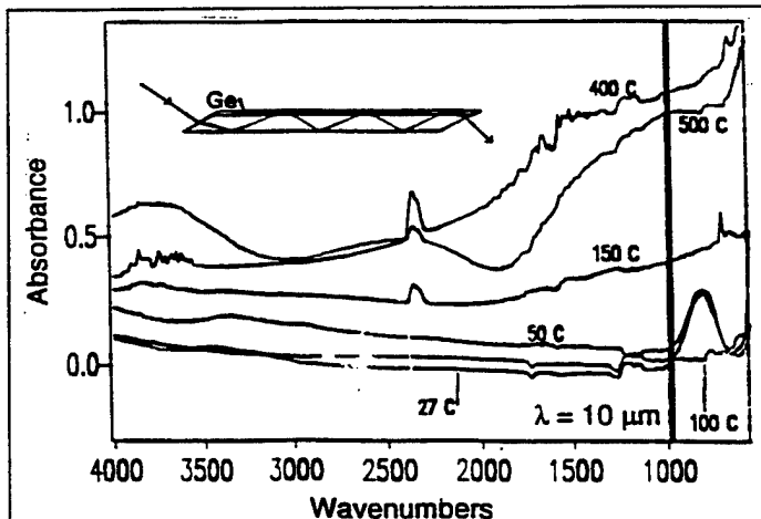
Figure 7. Spectral absorption of 0.5-1.5 μm thick Ge films, showing an optimal growth temperature to be around 100°C. At lower temperatures, an oxide peak forms at 830 cm -1 . At higher growth temperatures, free electron absorption from interface diffusion becomes severe.
