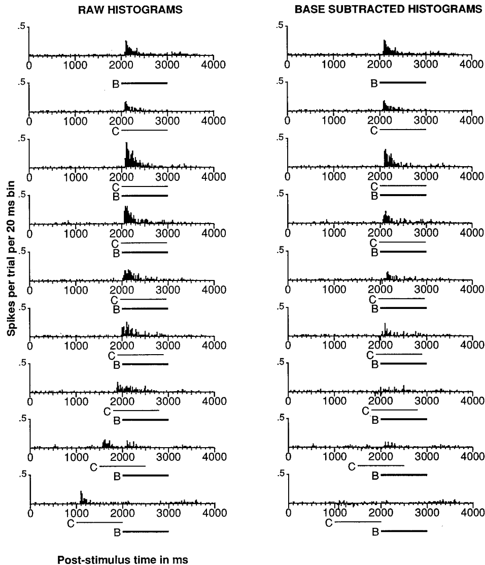
FIG. 2. PST histograms for same cell as in Fig. 1, showing effect of varying delay between 2 slits on resulting responses. Top 2 histograms on left and right: responses obtained when Slit A and Slit B, respectively, were presented by themselves. Below the top 2 histograms, histograms in left column are PST histograms obtained at various delays between Slits C and B. In right column , same data are plotted as on left , but with expected response of 1st slit (C), obtained from average of its PST histogram when presented alone, subtracted bin by bin from histogram when the 2 slits were presented in sequence (base subtraction). This base subtraction (described in METHODS) shows effect of the 1st slit on response to the 2nd slit with expected excitation due to the 1st slit removed.
