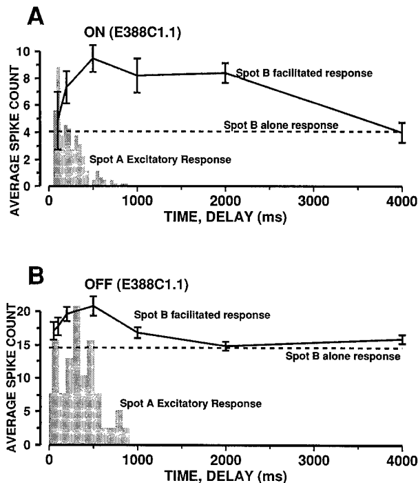
FIG. 4. Facilitation of ON ( A ) and OFF ( B ) responses of a 2nd slit as a function of interslit delays up to 4,000 ms, for cell E388C1.1 . Plots have same scheme as in Fig. 3. Modulation contrast was to 20% above background. Facilitatory process can be seen to be sustained for \geq 2,000 ms for ON response ( top ), and for at least 1,000 ms for OFF response ( bottom ) and clearly lasts much longer than excitatory response of the 1st slit when presented alone, indicated by shaded area.
