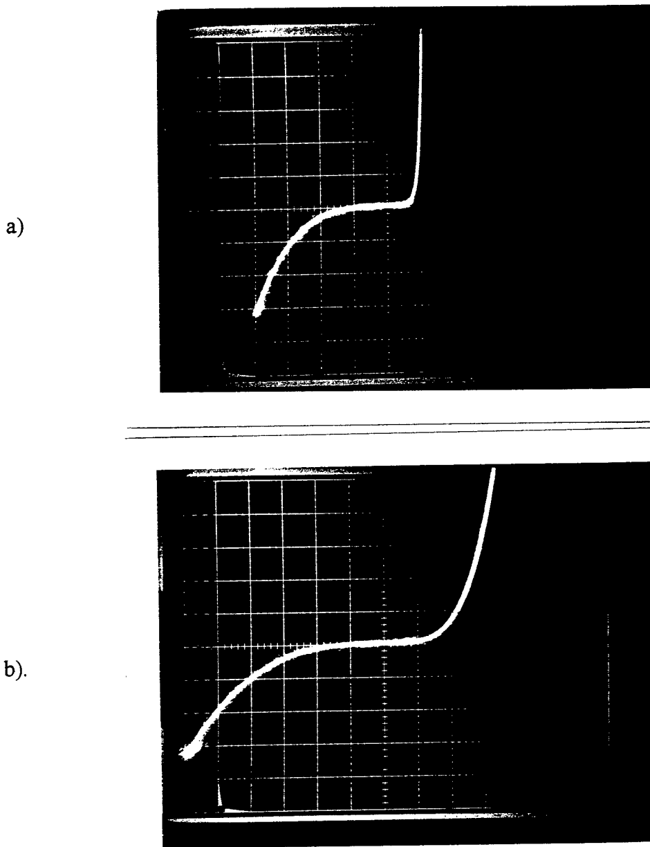
Figure 1. Current voltage curves for GaN PN junctions (350 \mu\text{m} octagons). a) Curve taken from the center of the wafer. The scales are 2V/div. hor. and 50 \mu\text{A}/\text{div} vert., b) Curve from edge of wafer. The scales are 0.5 V/div. hor. and 50 \mu\text{A}/\text{div} vert.
