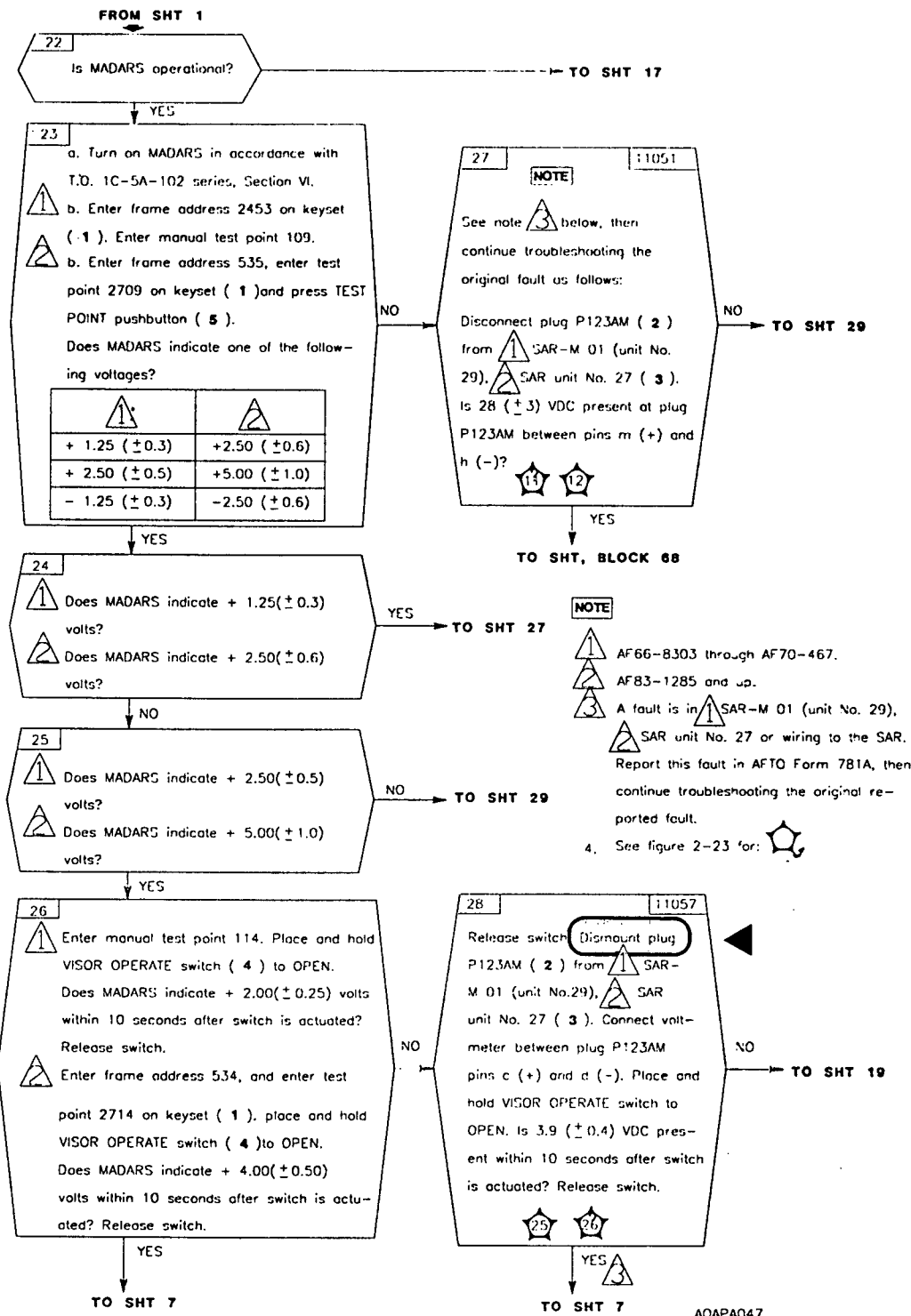
Figure 2-8. Visor Locks Do Not Unlock for Visor Open Sequence (Sheet 1 of 2) (Drawn) (ART017)
