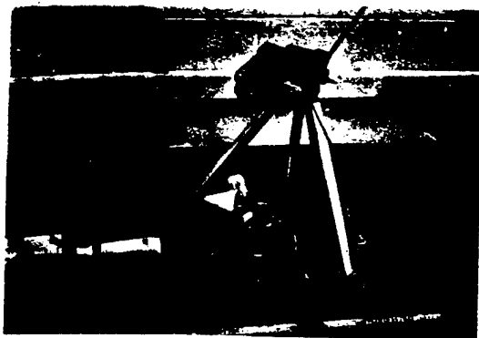
FIG. 1.—Holographic micro-velocimeter setup used to measure the settling velocity of the mica flakes.
