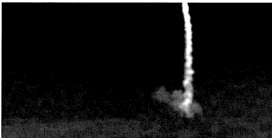
Figure 4. #K19 launch cloud viewed from UCS-07 blockhouse roof at 00:30 (mm:ss after launch). (a) visible imagery and (b) infrared imagery.
