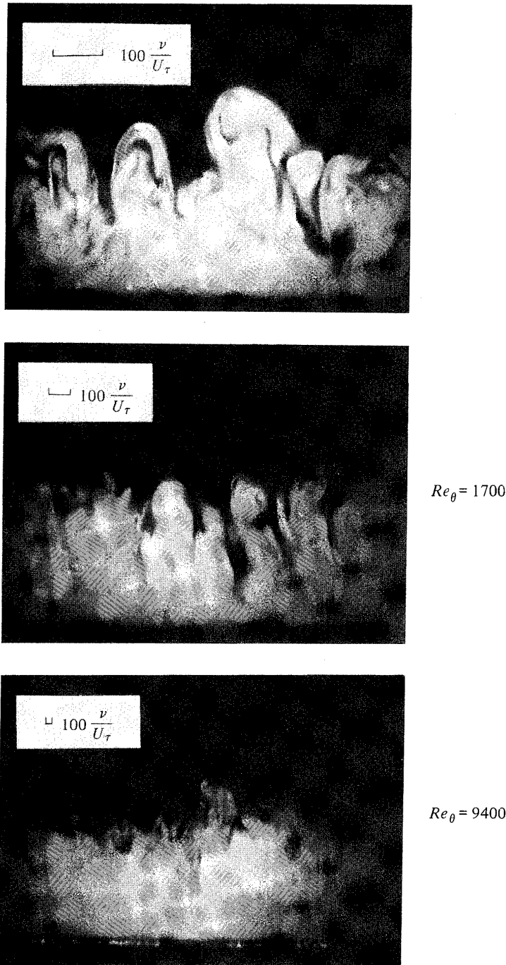
Figure 39: Flow visualizations by Head & Bandyopadhyay (1981), showing the Reynolds number dependence of vortex loop structures in a turbulent boundary layer. The visualizations were obtained by filling the boundary layer with smoke, and illuminating the flow with a laser sheet inclined 45^\circ downstream. a) Re_\theta = 600 ; b) Re_\theta = 1,700 ; c) Re_\theta = 9,400 . Figure from Head & Bandyopadhyay (1981).
