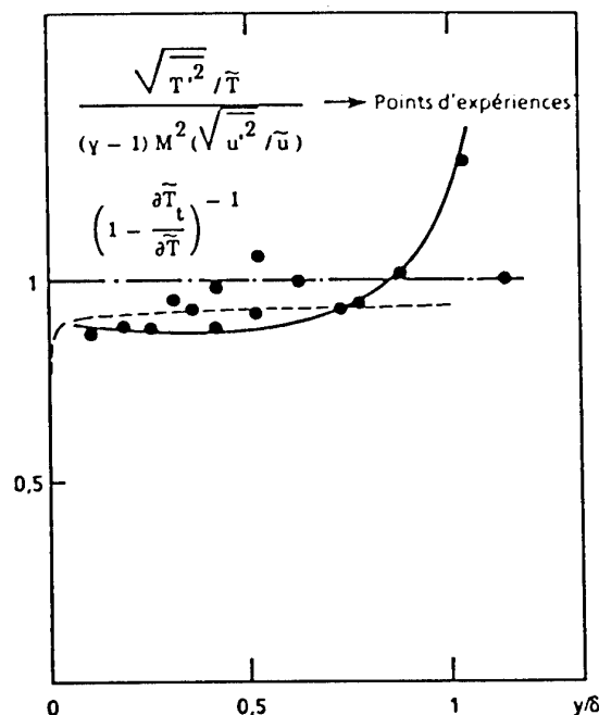
Figure 62: Test of the Strong Reynolds Analogy in a supersonic boundary layer ( M_e = 2.32 , Re_\theta = 5,650 ). Data from Debiève (1983).
