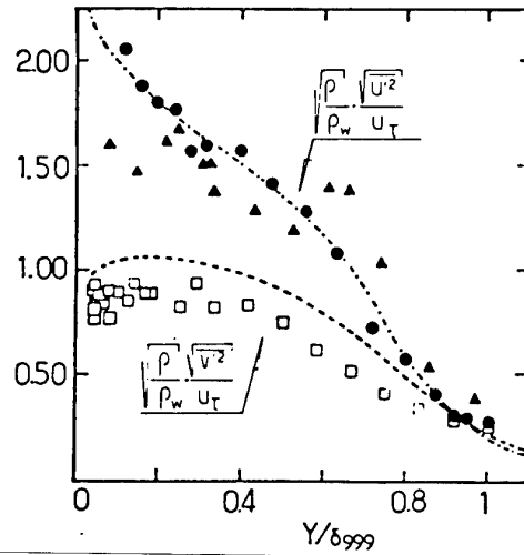
Figure 59: Turbulence distributions in a Mach 2.3 boundary layer, measured using LDV ( Re_\theta = 5,650 ). Figure from Eléna & Lacharme (1988).
