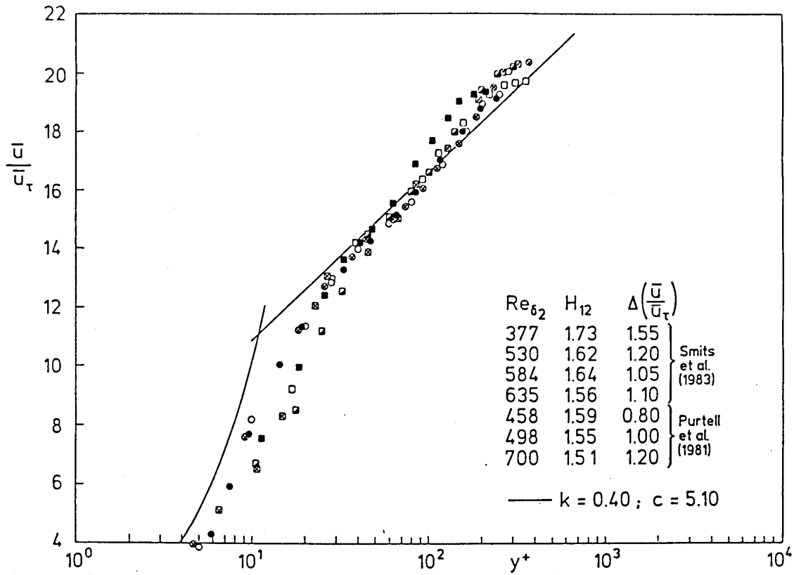
Figure 8: Development of the mean velocity in inner-law scaling in a zero pressure gradient low-Reynolds-number incompressible boundary layer. Figure from Fernholz & Finley (1995).
