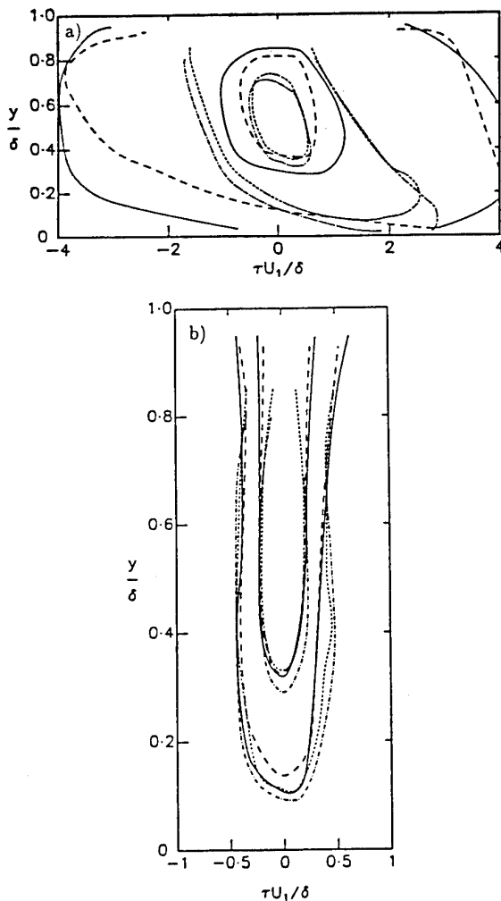
Figure 45: Reynolds number dependence of isocorrelation contours of: a) R_{uu} , b) R_{uv} . Re_\theta = 1,360 —; 2,180 - - -; 6,030 - · - · -; 9,630 — · — · —. One probe was fixed at y/\delta = 0.56 . Two contour levels, 0.05 and 0.2, are shown for each Reynolds number. Figure from Antonia et al. (1990b).
