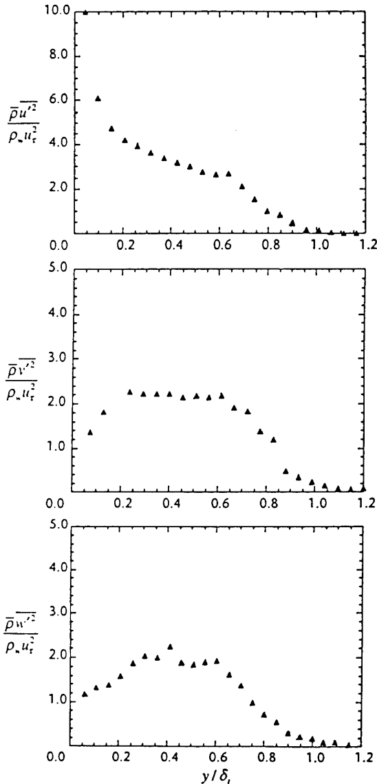
Figure 58: Turbulence distributions in a Mach 2.9 boundary layer, measured using hot-wire probes ( Re_\theta = 65,000 ). Adapted from Konrad (1993).
