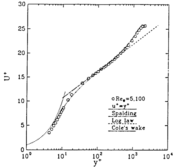
Figure 4: Example of a measured mean velocity profile at Re_\theta = 5,100 from Purtell et al. (1981) scaled on inner variables, and compared to theoretical and empirical scaling-laws: \circ data; — the linear sublayer; - - - the buffer region according to Spalding (1961); - · - the logarithmic overlap region (equation 24); - - - Coles' law-of-the-wake (equation 27). Figure from Smith (1994).
