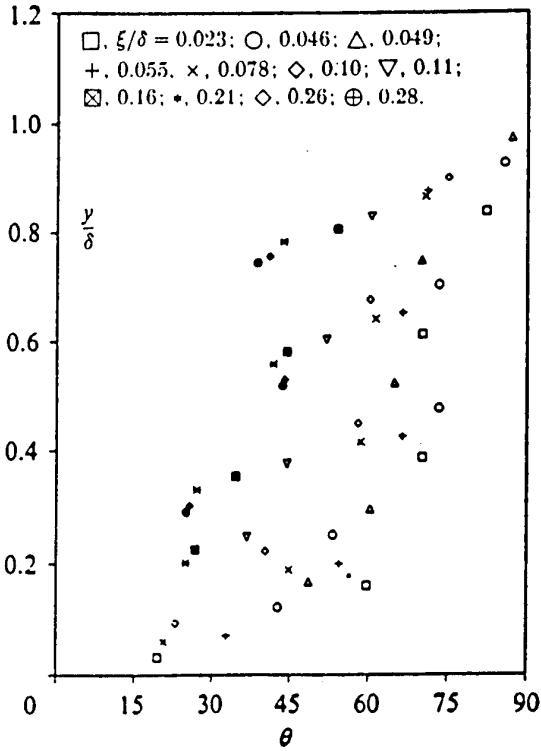
Figure 46: Broadband structure angle in a subsonic boundary layer, as a function of probe-separation distance. Figure from Alving et al. (1990b).
