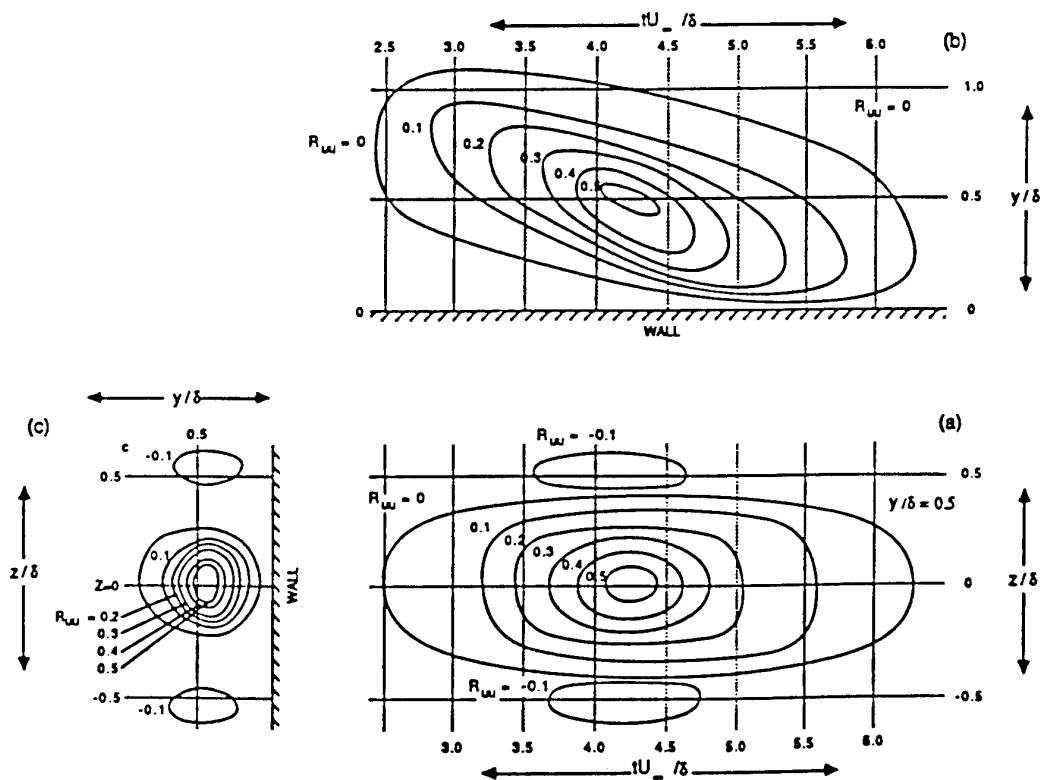
Figure 43: Isocorrelation contours of space-time correlations of the streamwise velocity component measured by Kovaszny et al. (1970). a) x-z plane, b) x-y plane, and c) y-z plane. The position of one probe was fixed at y/\delta = 0.5 . Figure from Smits et al. (1989).
