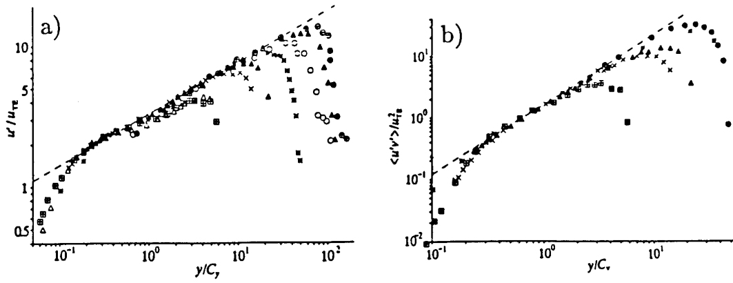
Figure 26: Turbulence stresses scaled on “typical” eddy velocity and length scales, u_{TE} and C_v , respectively: a) u'_{rms} for 1,010 \leq Re_\theta \leq 39,000 . b) -\overline{u'v'} for 1,010 \leq Re_\theta \leq 14,500 . See Falco (1991) for data sources (reproduced from Falco, 1991).
