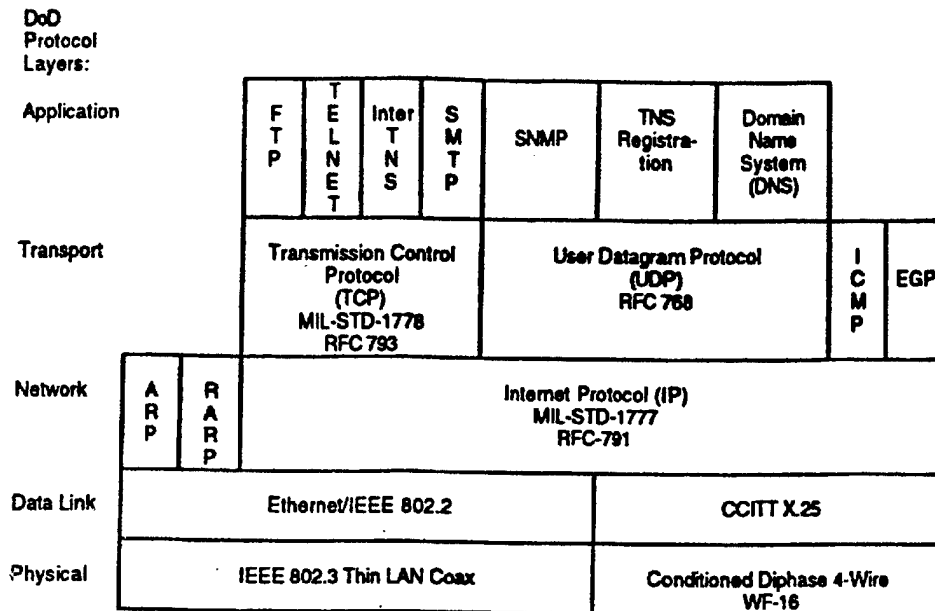
Figure 19. Some Protocols Used Within TPN From [Ref. 10, p. 11]
