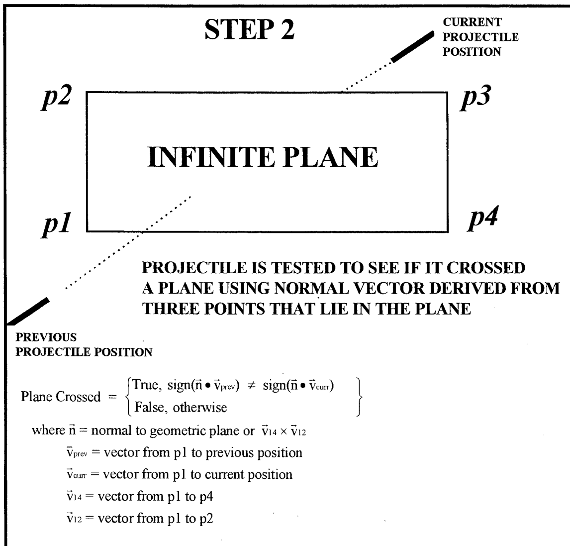
Figure 6: Step 2 of Hit Algorithm
