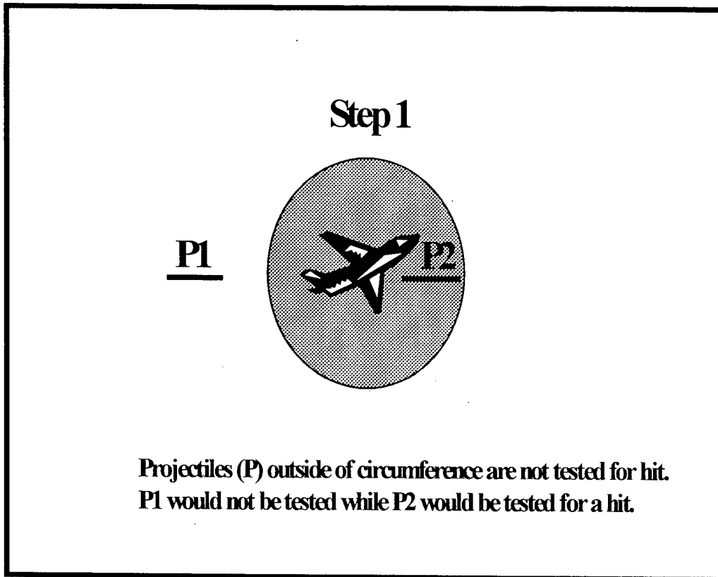
Figure 5: Step 1 of Hit Algorithm
