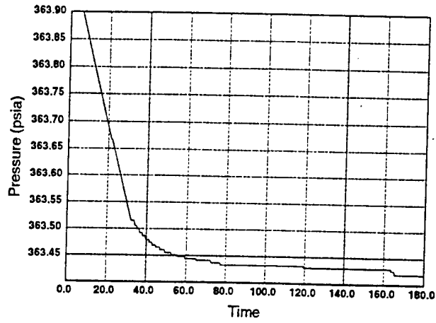
(a) Tank 1 pressure.
