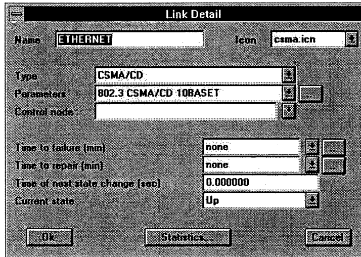
Figure 3.6 Ethernet Link Detail Window
