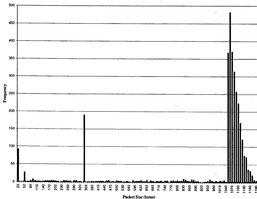
Figure 7.2 Packet Size Histogram
