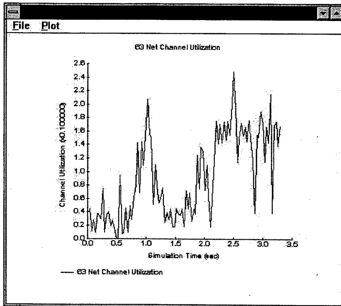
Figure 6.15 Ethernet Utilization
