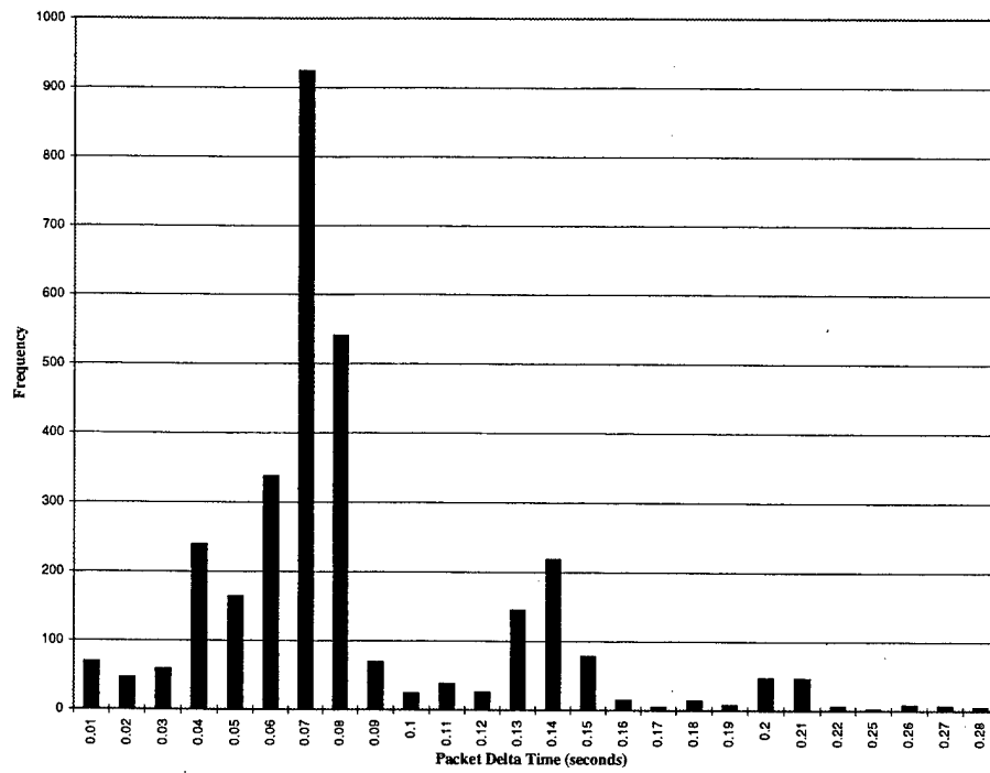
Figure 7.3 Packet Interarrival Time Histogram
