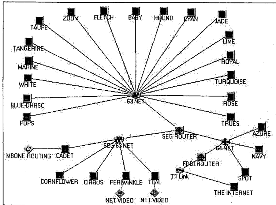
Figure 7.5 Proposed Network Topology
