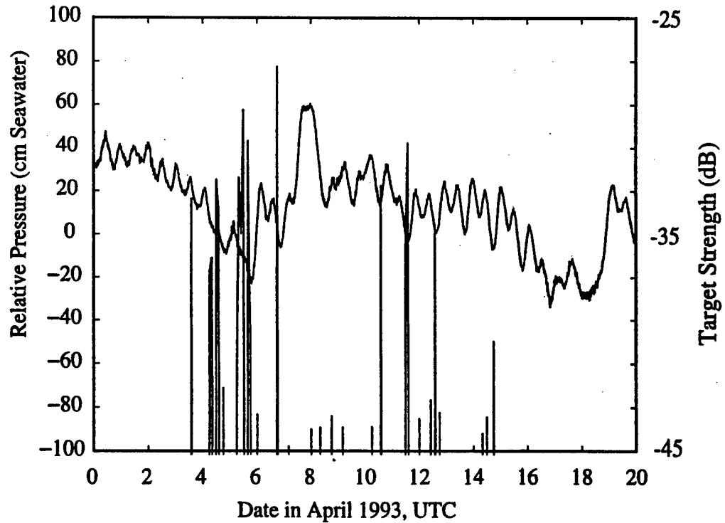
Figure 11. Seafloor Pressure and Target Strength, Eckernfoerde First Deployment
