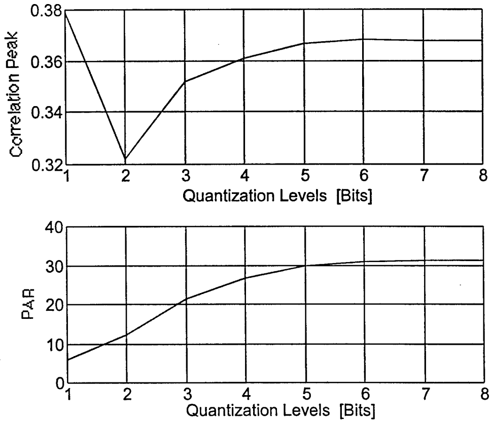
FIGURE 7.11. PERFORMANCE PARAMETERS
