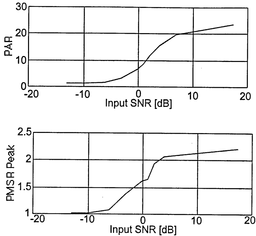
FIGURE 7.14. PERFORMANCE PARAMETERS AS A FUNCTION OF SNR_i (CONTINUED)
