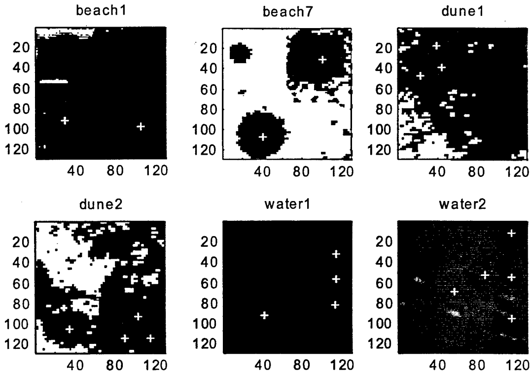
FIGURE 9.5. IMAGES AND TARGET LOCATION AS DETECTED BY CORRELATOR (SPATIAL FILTER USED IS POOF AND PAR_{th}=3 )
