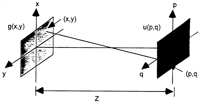
FIGURE 3.1. ELECTRIC FIELD PROPAGATION THROUGH A DISTANCE
