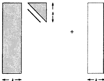
Figure 3: Leading k columns V_kH_k + f_k e_k^T form a length k Arnoldi factorization after discarding the last p columns.
