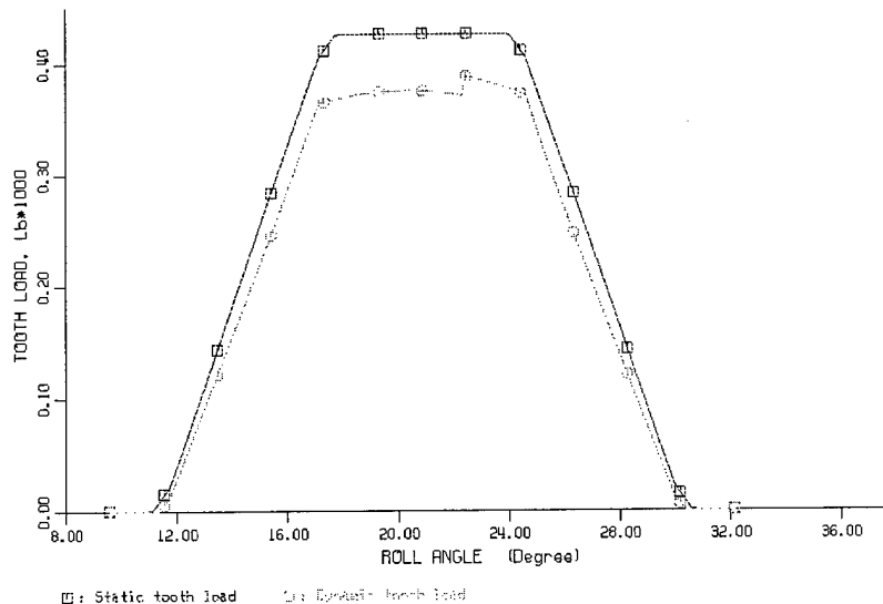
Figure 7—Example of underestimated dynamic load for Test Case I gears, 100 000 rpm, 700 in-lb
