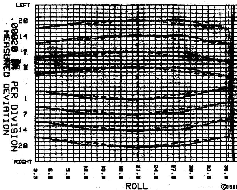
Figure 5--Profile chart for the pinion of test case III
