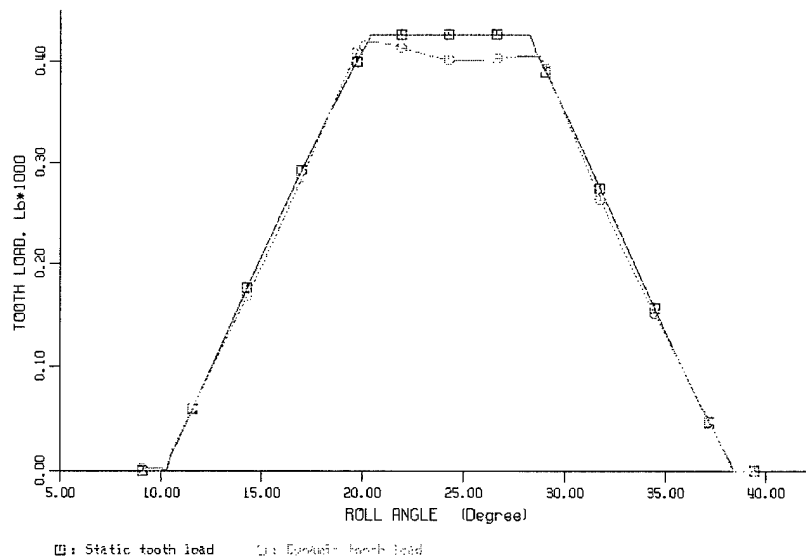
Figure 4—Static and dynamic tooth loads for the gears of test case II
