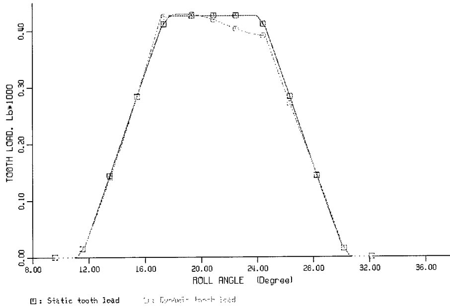
Figure 2--Static and dynamic tooth loads for the gears of test case I
