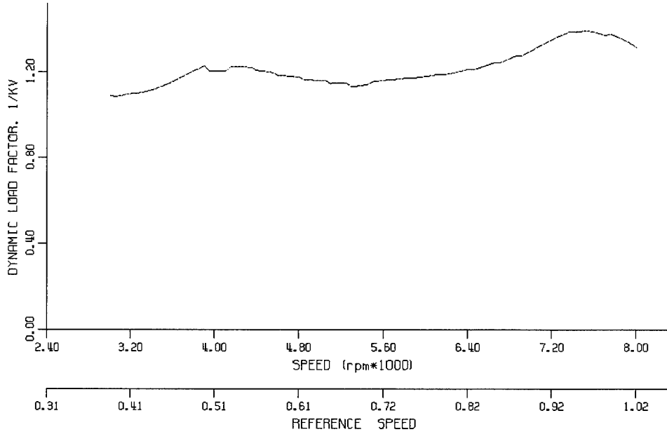
Figure 6--Speed survey of dynamic load factor for the gears of test case III
