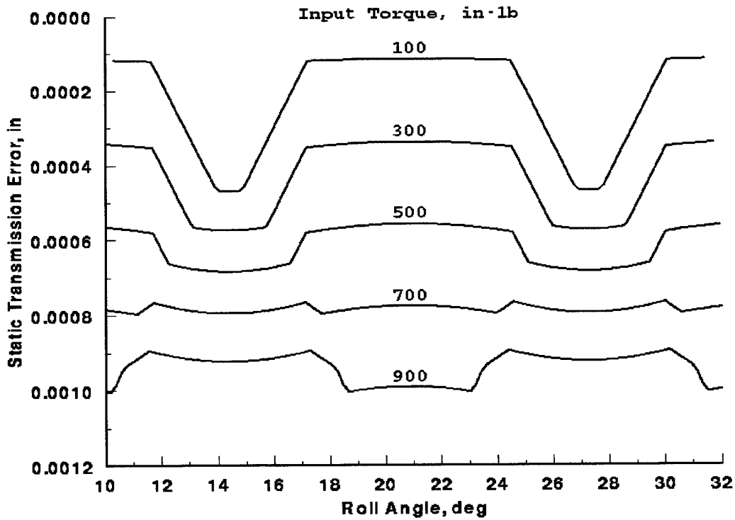
Figure 3--"Harris map" of static transmission error for the gears of test case I
