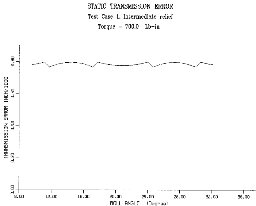
Figure 1--Static transmission error for the gears of test case I
