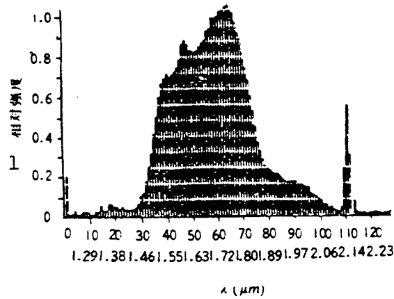
Fig. 4. Typical backward SRS time integral spectrum in blackbody targets Peak with a wavelength 2.14\mu m is dipole spectrum of light with a wavelength 1.06\mu m
