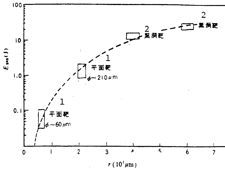
Fig. 3. Interdependent relations between SRS energy ( E_{SRS} ) and plasma radial scale r ( 10^2\mu m )
