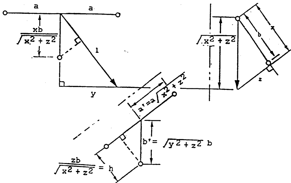
Fig. 6. Front Projection for Determining a' , b' , h
