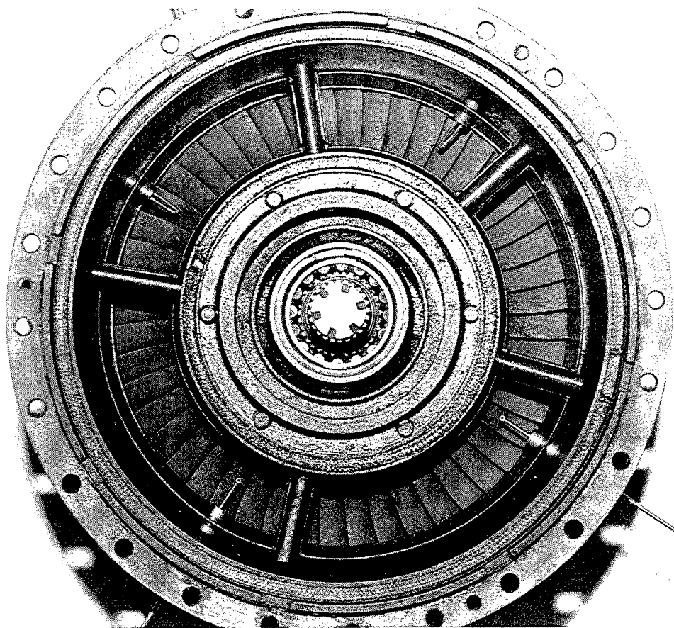
Figure 4.10. Installed view of both Kiel probes and thermocouples for the power turbine inlet conditions.
