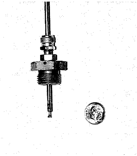
Figure 4.5. 1/8" combination Kiel - thermocouple probe used for compressor discharge measurements.
