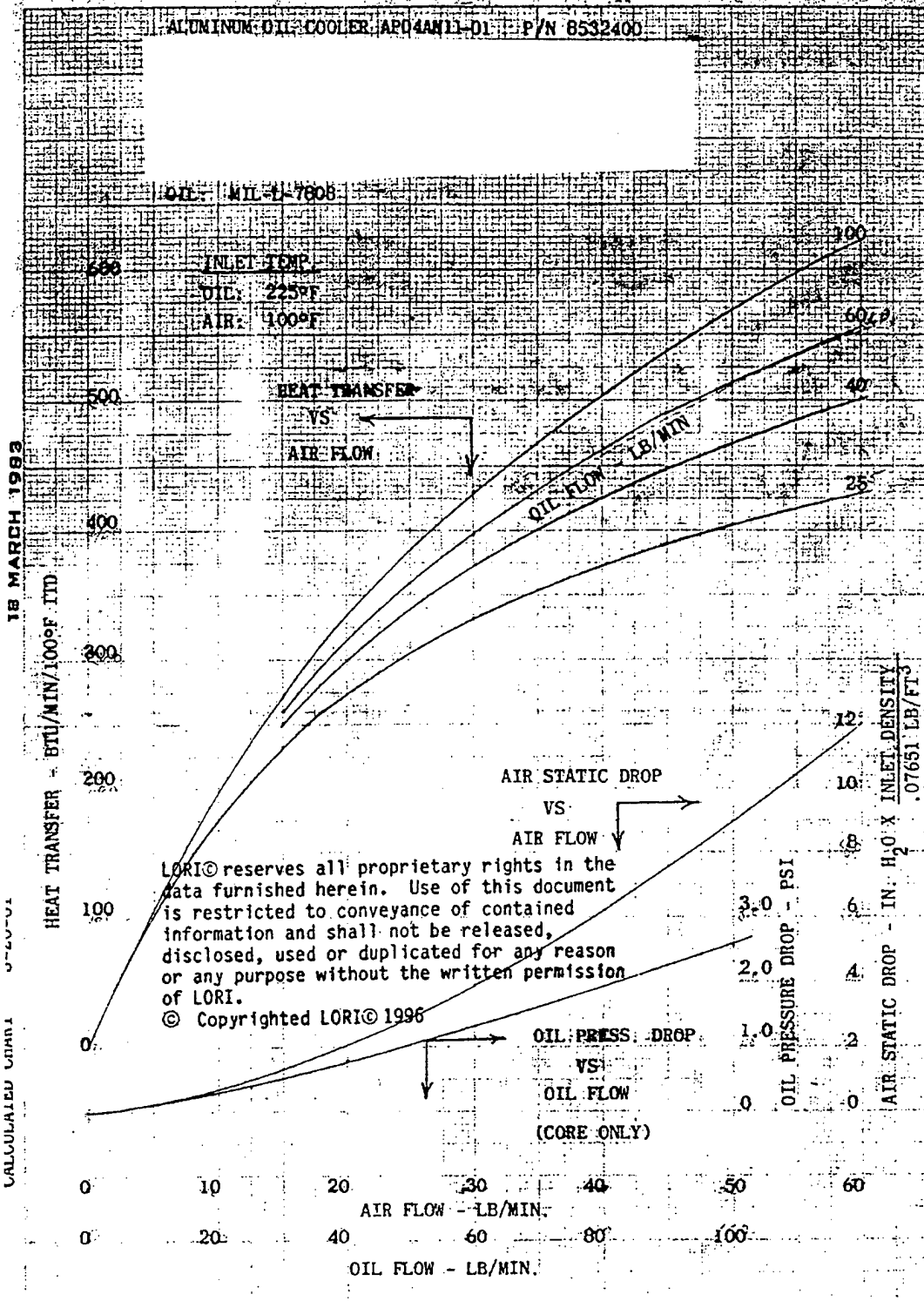
Figure 5.7. UH-1 transmission oil cooler heat transfer curves. "From Ref. [9]."
