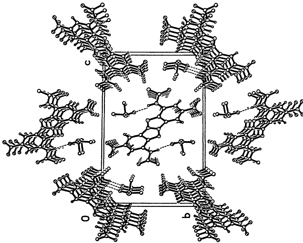
FIGURE A-5. Molecular Assembly of 4,10-Bis(acetamido)-2,8-dinitrobenzo-1,3a,4,6a-tetraazapentalene (13) in the Crystal.
