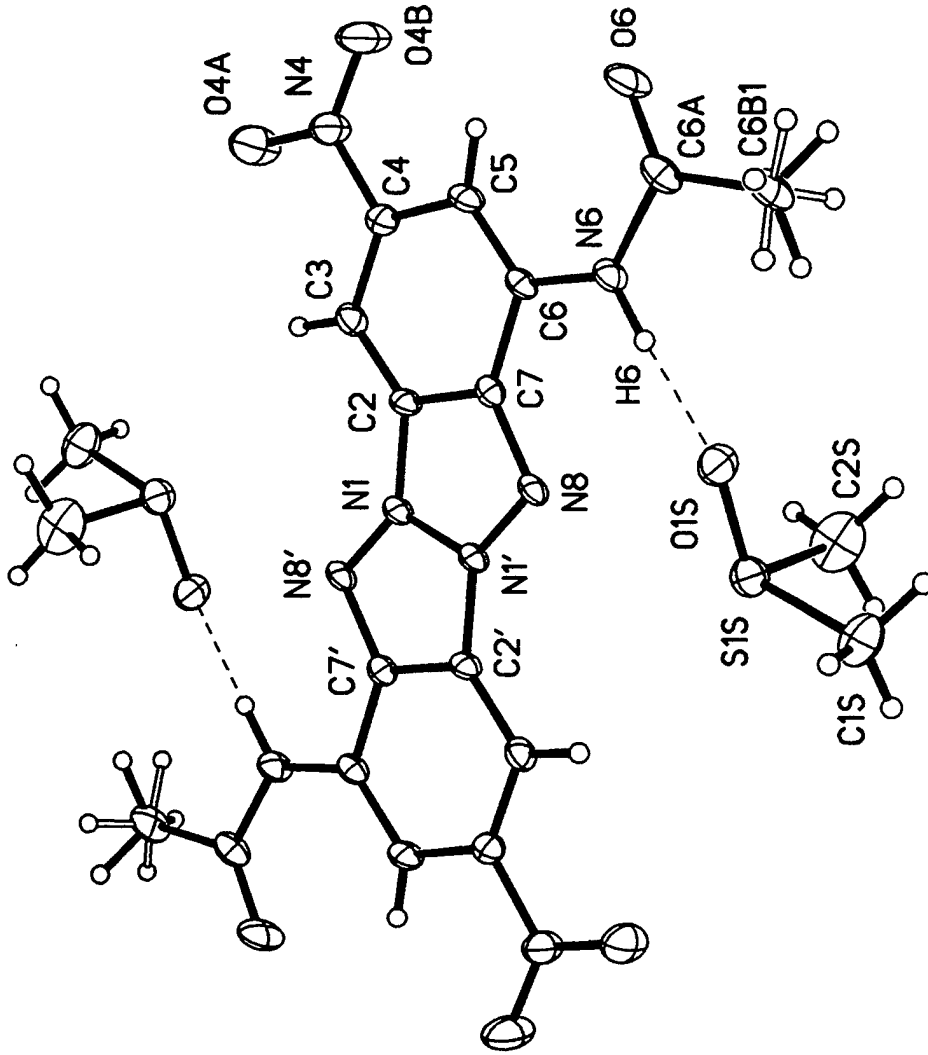
FIGURE A-4. Molecular Structure of 4,10-Bis(acetamido)-2,8-dinitroindobenzene-1,3a,4,6a-tetraazapentalene (13).
