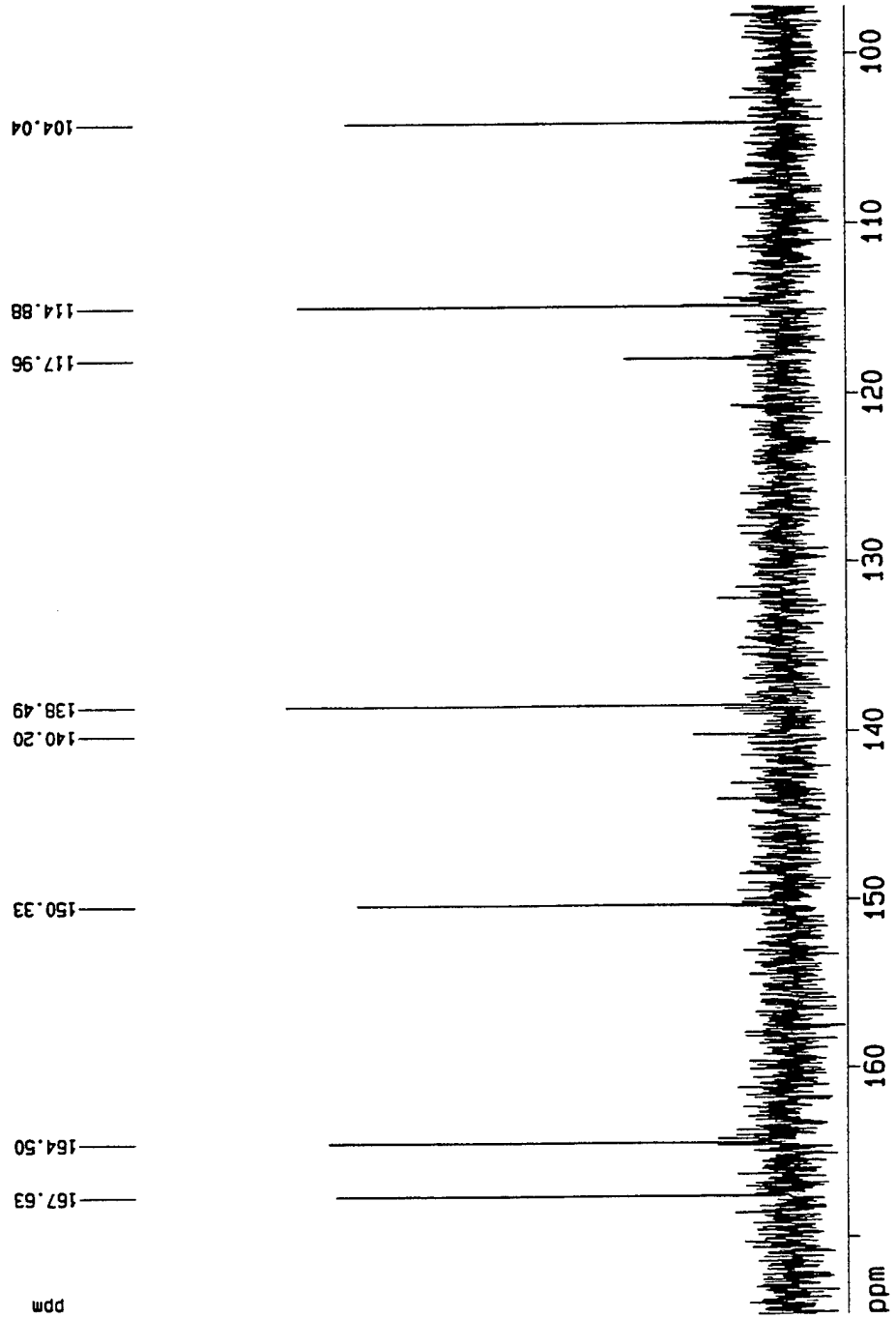
FIGURE 4. Solution ^{13}\text{C} NMR Spectrum of Compound 9 (prepared at China Lake), Run in DMSO at 350 K.
