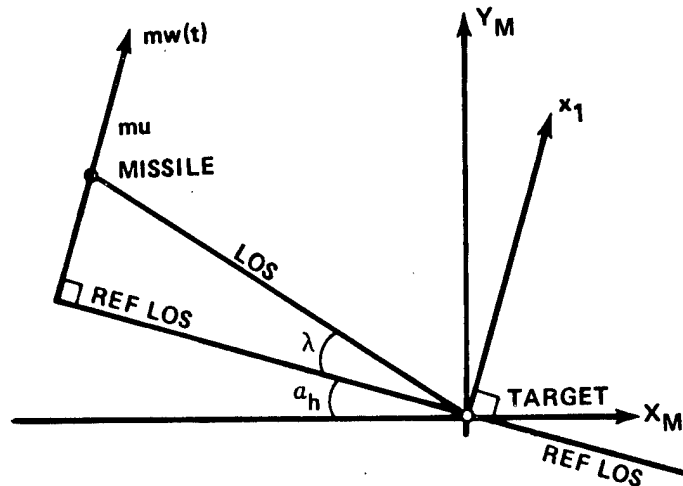
Figure 1. Relative intercept geometry.
