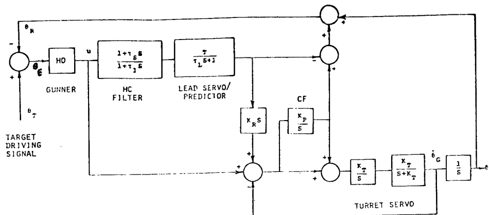
Fig. 3. Disturbed Reticle Design, State Variable Model.
