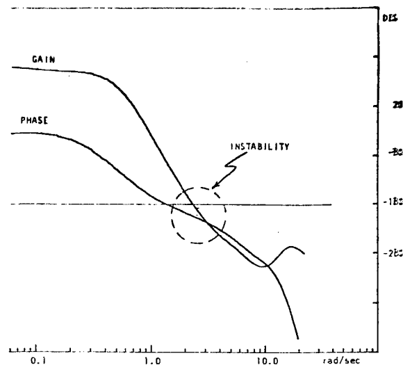
Fig. 11. DR Gunner-Vehicle Open-Loop Transfer Function, K_R=0.5
