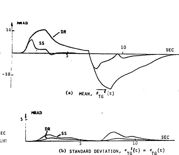
Fig. 15 "First-Order" Gun Pointing Error Statistics
