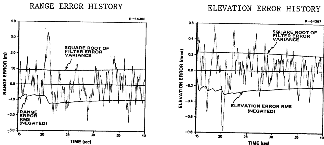
Figure 6 . Anti-Radar Missile Tracking Performance
