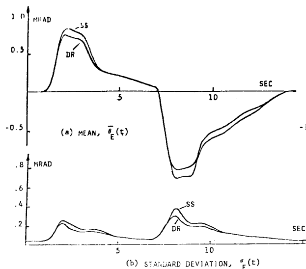
Fig. 14 Tracking Error Ensemble Statistics
