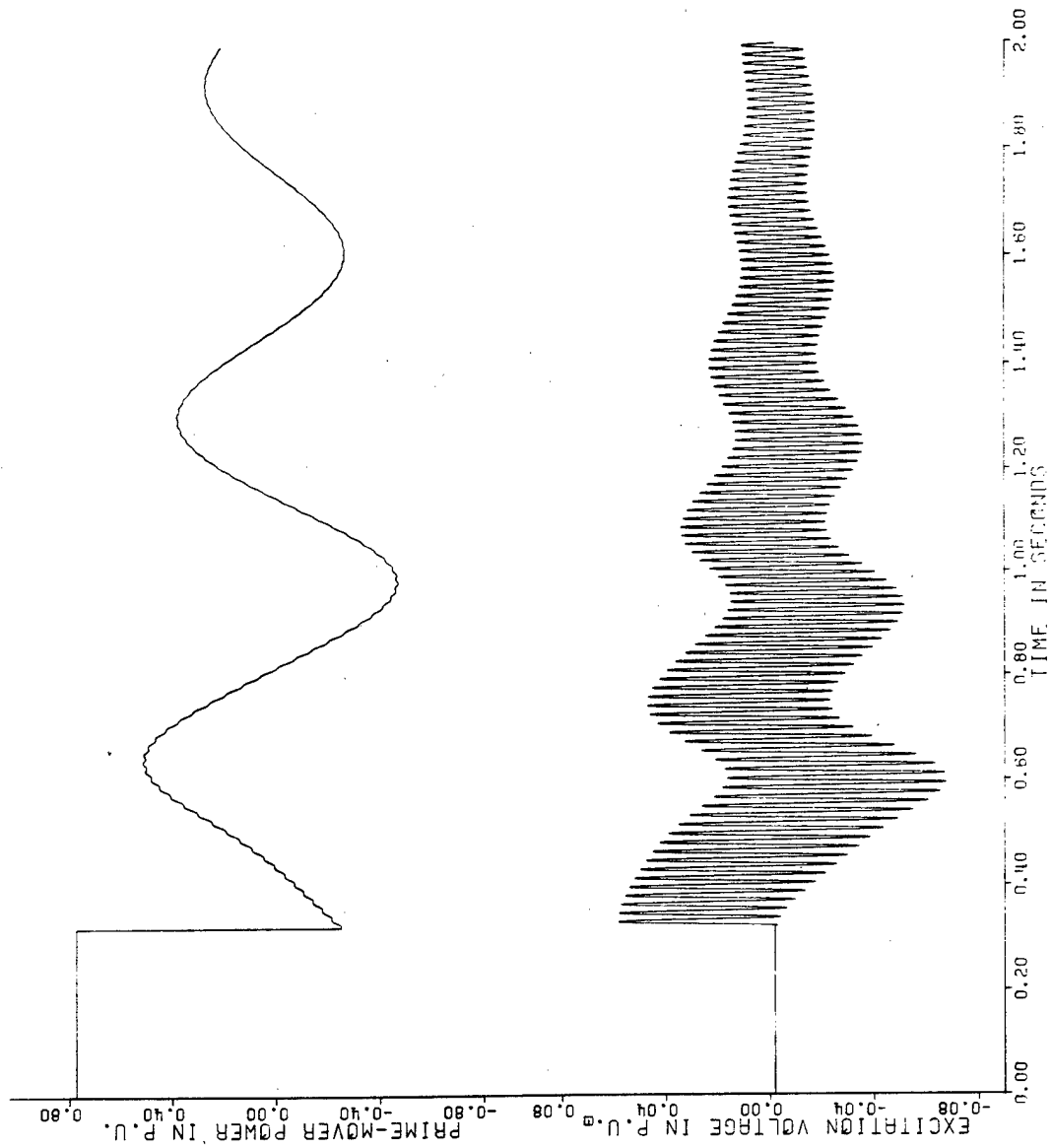
FIGURE 4 CONTROLLER BEHAVIOR
