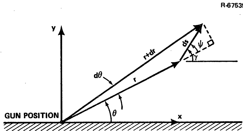
Figure 9 Geometrical Relationships for Prediction Error Analysis
