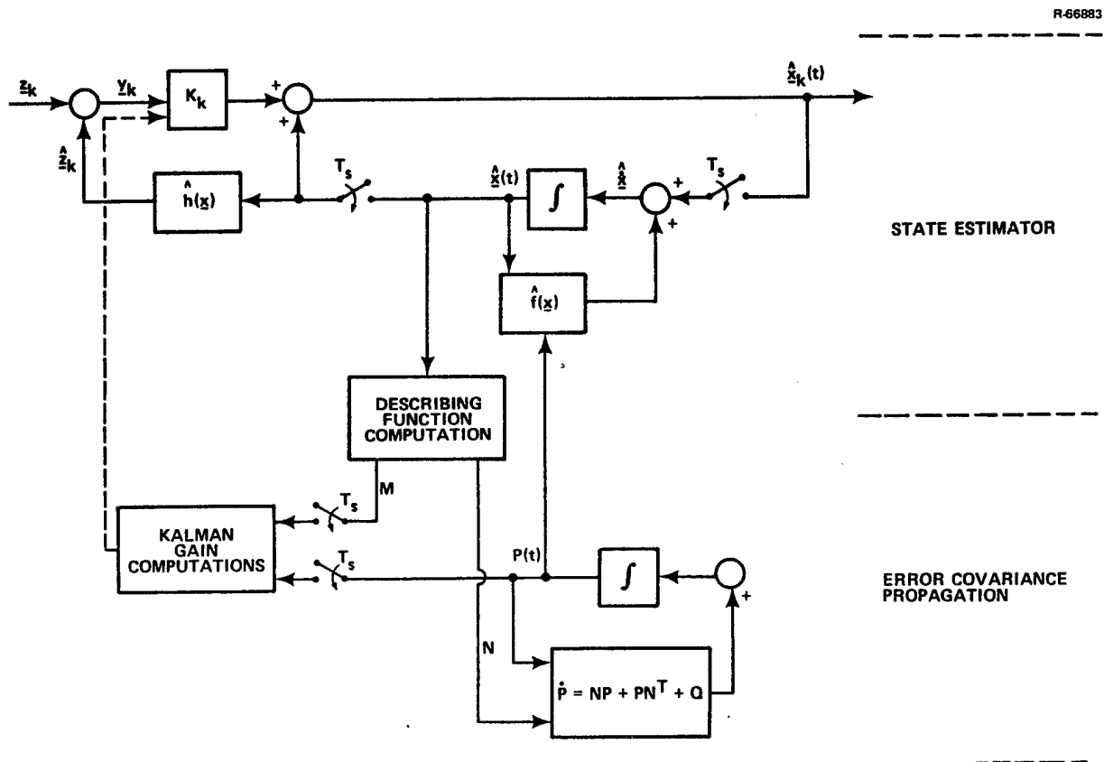
Figure 3 Statistically-Linearized Kalman Filter
