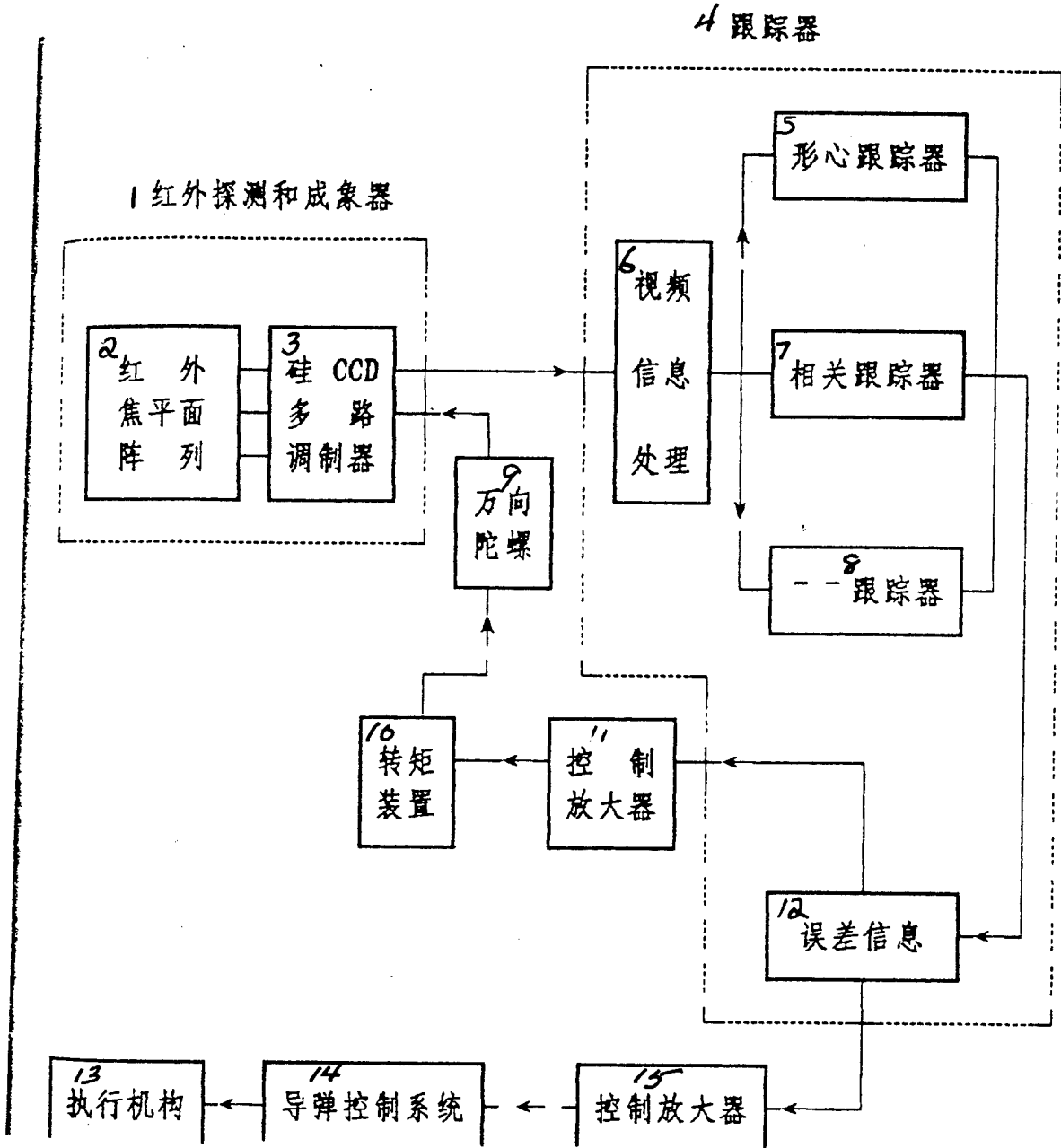
Fig. 1. The principles of infrared imaging guidance
