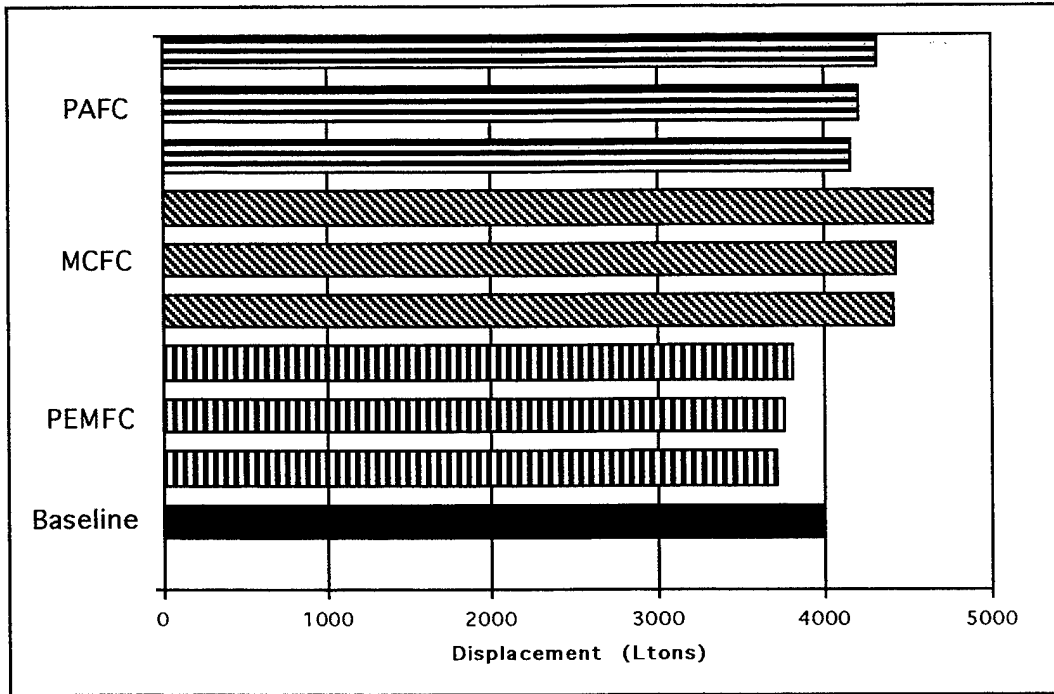
Figure 4-5, Displacement Comparison
