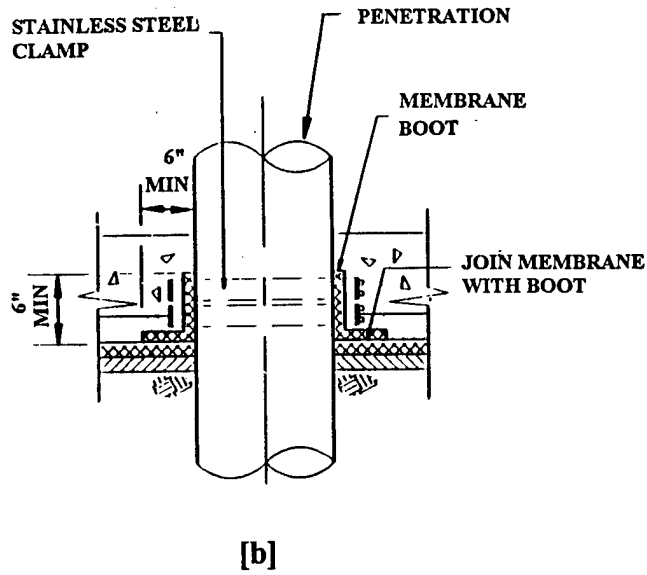
Figure 6.5. [a] Sub-Slab Geotextile Membrane (Source: 28, Exhibit 4-16) [b] Utility Service Penetration Through Slab (Source: 28, Exhibit 4-17)
