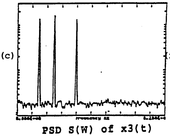
Figure 9(a), 9(b), & 9(c): PSDs for x_1(t) , x_2(t) & x_3(t) . 9(d), 9(e), & 9(f): Auto-Bicoherence for x_1(t) , x_2(t) & x_3(t) .
