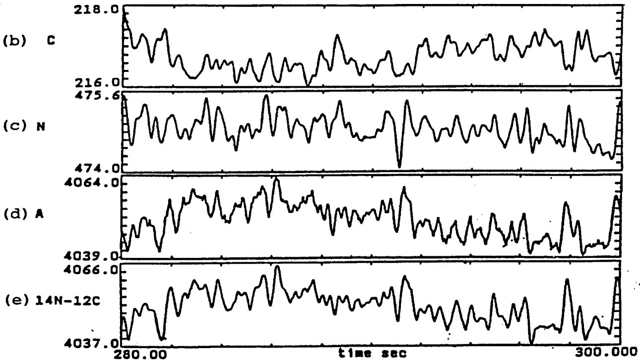
Figure 22 (a) PSD of HPOTP Strain Gauge Measurement. (b) Instantaneous Frequency (IF) of Cage (C). (c) Instantaneous Frequency (IF) of Sync (N). (d) Instantaneous Frequency (IF) of Anomaly (A). (e) 14 times of IF Signal of N (Figure 5-c) minus. 12 times of IF Signal of C (Figure 5-b).
