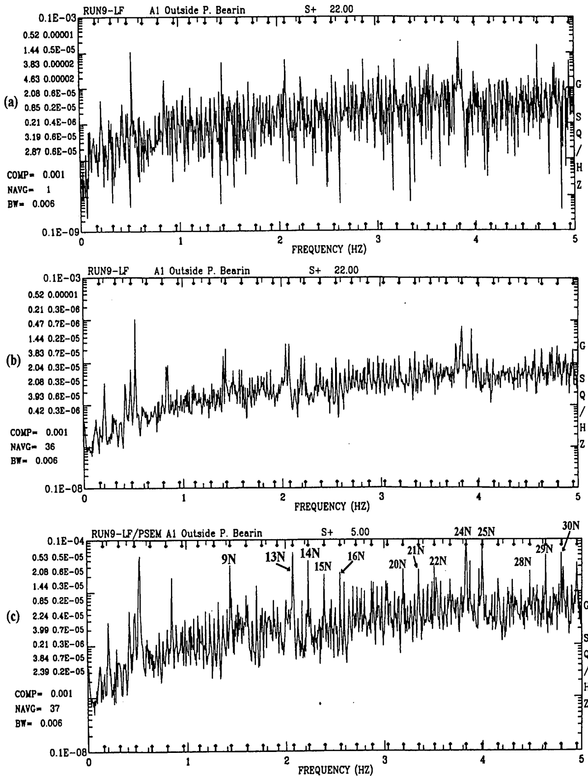
Figure 14: (a) Raw PSD of outer Wheel Bearing measurement over one cycle of antenna excursion (b) Raw PSD Averaging over 22 cycles of antenna excursion (c) PSEM PSD Averaging over 22 cycles of antenna excursion
