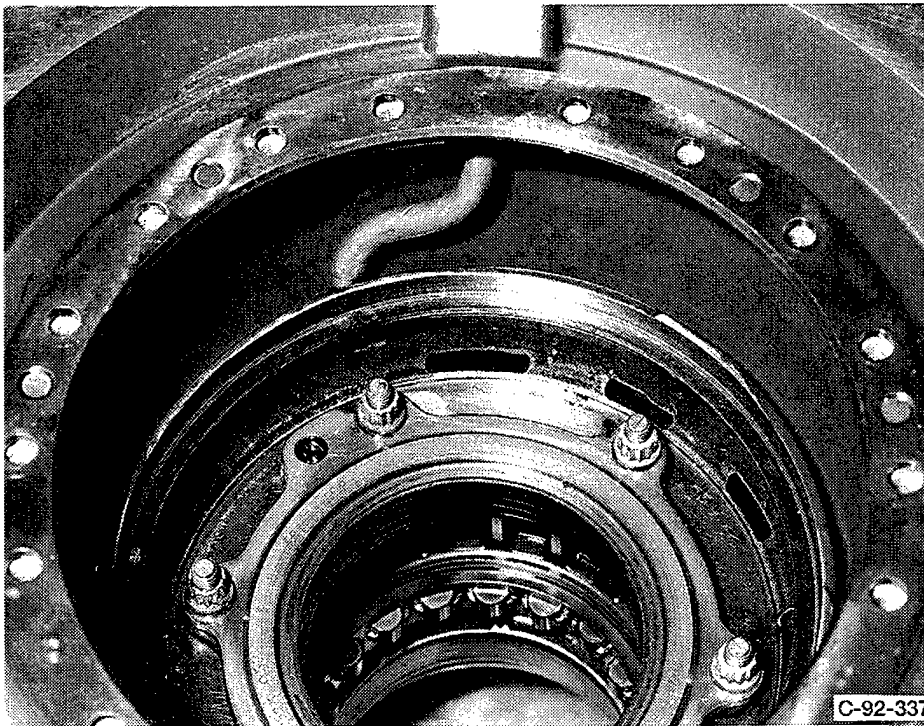
(b) Seal package cavity and housing.
