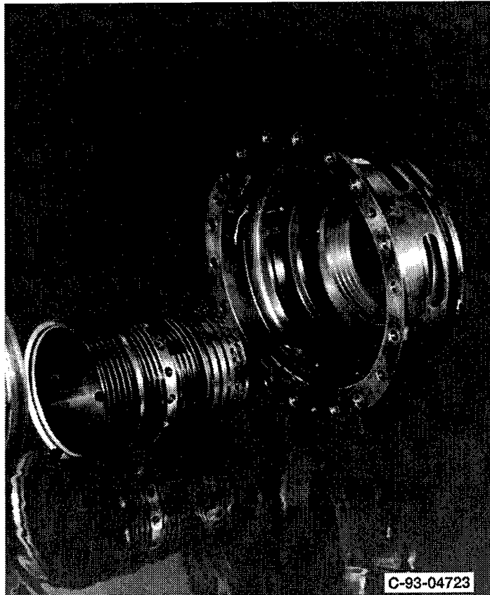
Figure 3.—Simulated exploded view of labyrinth compressor discharge seal system.
