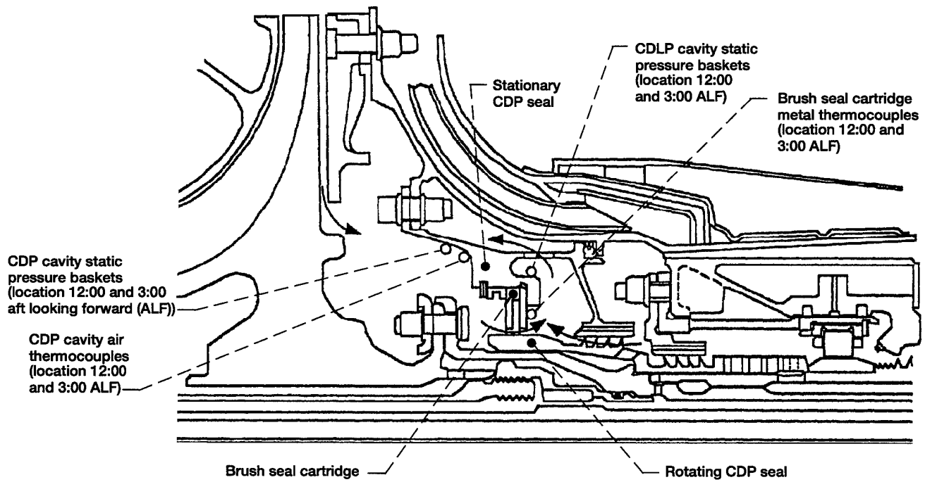
(a) Brush seal package and airflow.
