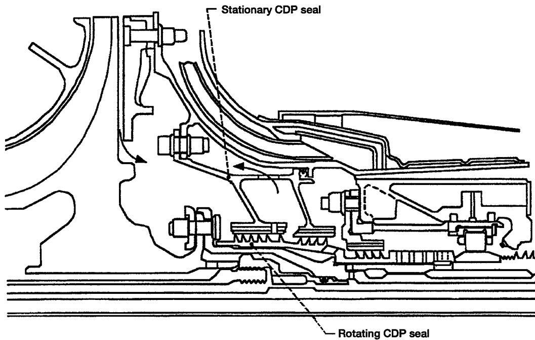
(a) Labyrinth seal package and airflow.
