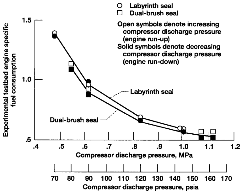
Figure 15.—Experimental testbed engine specific fuel consumption as a function of compressor discharge pressure with labyrinth and dual-brush seals.
