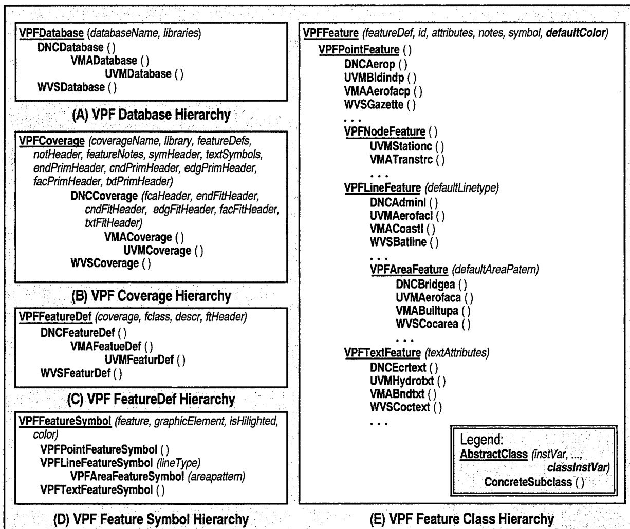
Fig. 1 — Selected OVPF class hierarchies with instance and class-instance variables indicated
