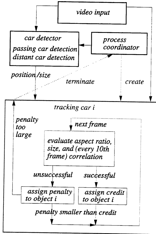
Figure 5: Tracking process i .
