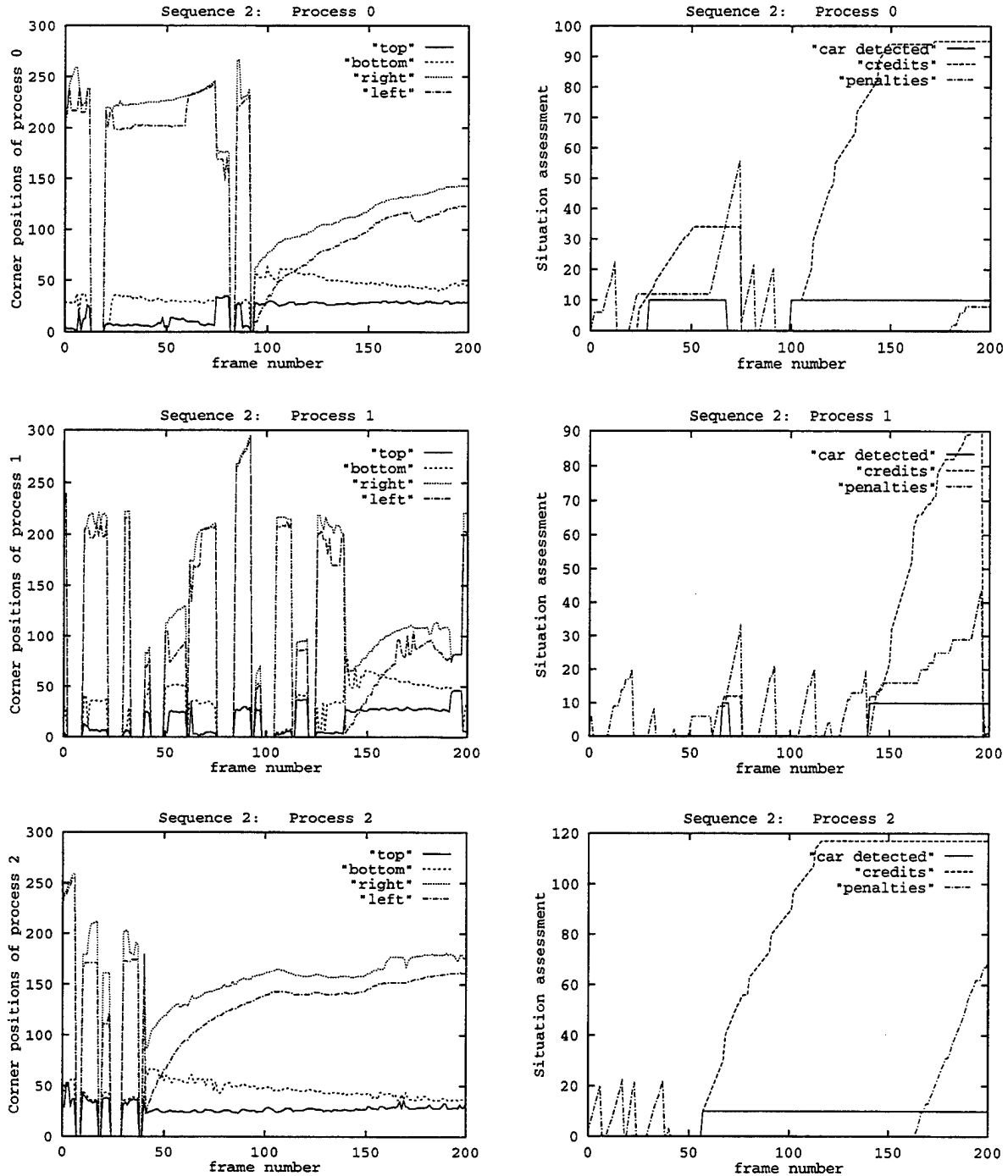
Figure 10: Analysis of Sequence 2 (Fig. 9): The graphs at the left illustrate the y -coordinates of the top and bottom and the x -coordinates of the left and right corners of the tracking windows of processes 0, 1, and 2, respectively. The graphs at the right show the credit and penalty associated with each process and whether the process has detected a car. As seen in the top graphs and in Fig. 9, process 0 tracks a traffic sign that is falsely recognized as the first car in frames 34–66. In frame 200, process 1 terminates tracking the second car, because not enough significant edges are found within window 1 for several antecedent frames (although the credits are much higher than the penalties).
