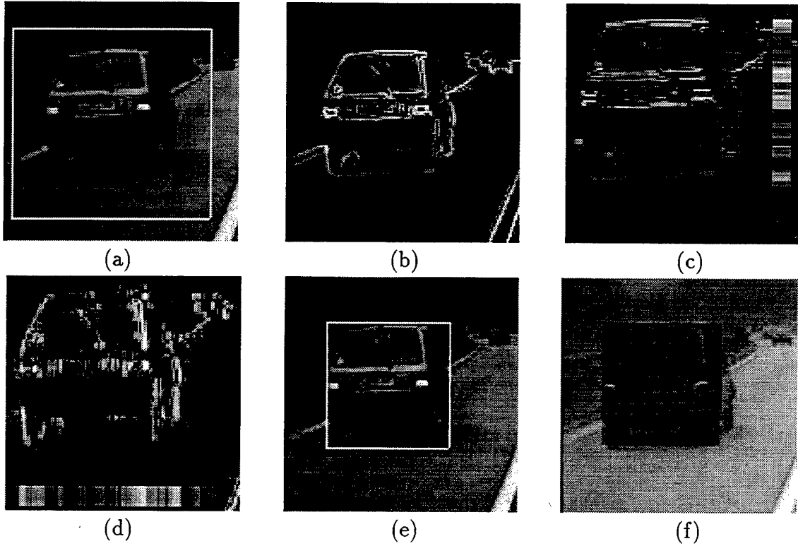
Figure 4: (a) An image with its marked search region. (b) The edge map of the image. (c) The horizontal edge map H of the image (enlarged). The column on the right displays the vertical projection values v of the horizontal edges computed for the search region marked in (a). (d) The vertical edge map V (enlarged). The row on the bottom displays the horizontal projection vector w . (e) Thresholding the projection values yields the outline of the potential car. (f) A car template of the hypothesized size is overlaid on the image region shown in (e); the correlation coefficient is 0.74.
