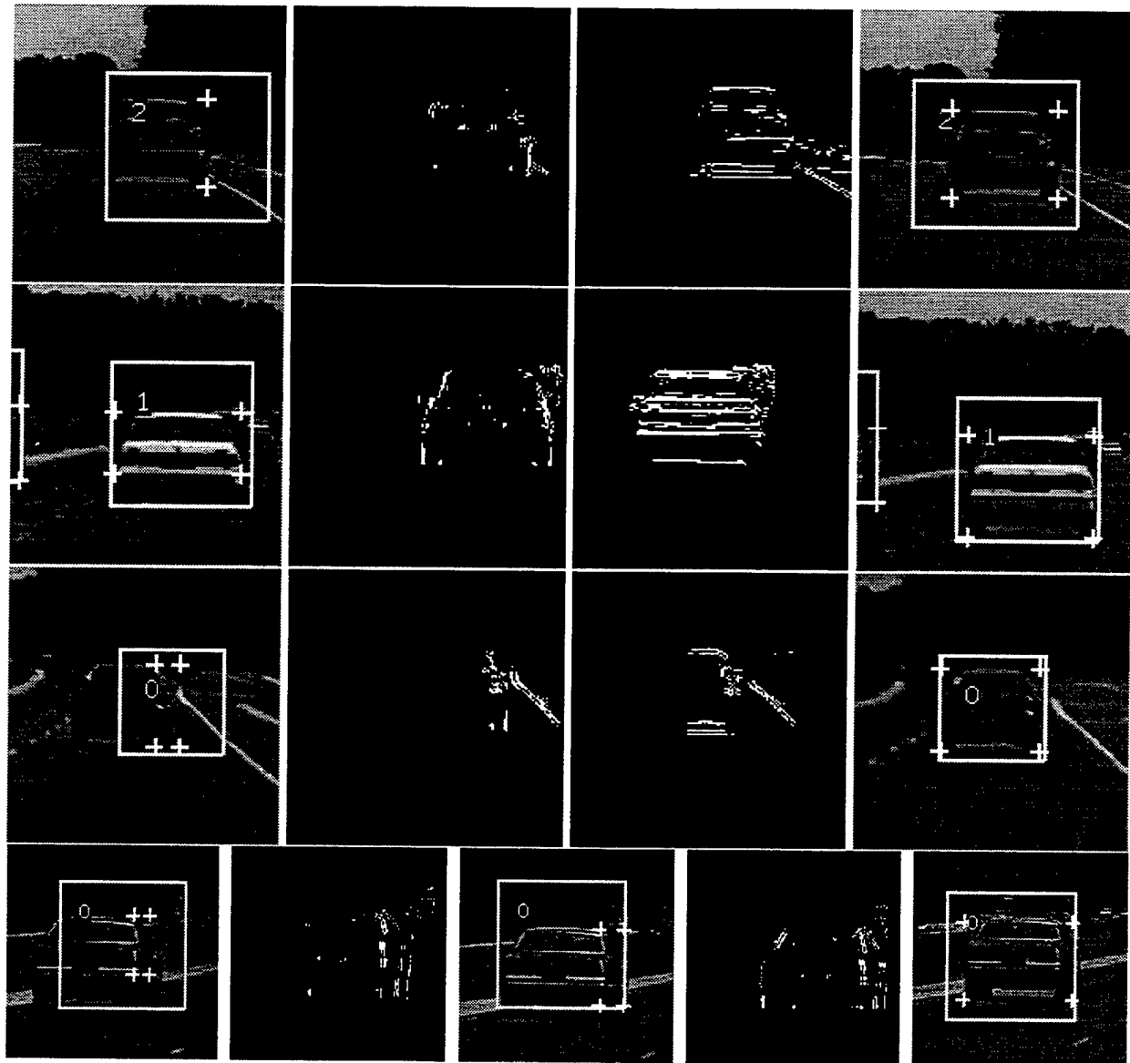
Figure 6: In the first row, the left and right corners of the car are found in the same position due to the low contrast between the sides of the car and background (first image). The vertical edge map resulting from this low contrast is shown in the second image. Significant horizontal edges (the horizontal edge map is shown in third image) are found to the left of the corners and the window is shifted to the left (fourth image).
