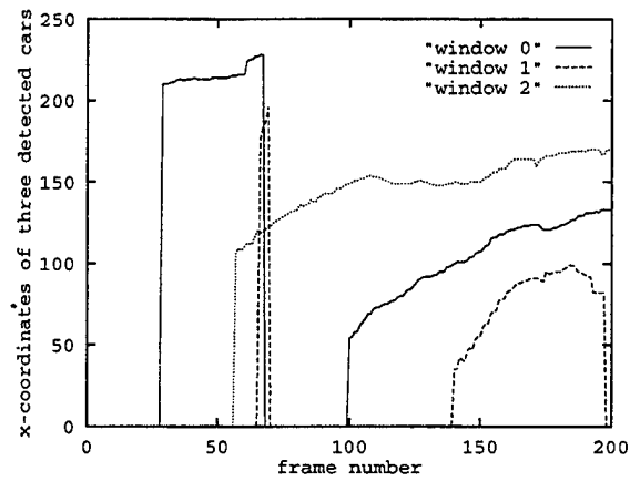
Figure 9: A second image sequence in which three cars are recognized and tracked. On the top, images are shown with their frame numbers in their lower right corners. The rectangles become white when the system recognizes the tracked objects to be cars. A traffic sign causes a false alarm and is tracked by process 0 in frames 34-66. The graph on the bottom shows the x -coordinates of the positions of the three recognized cars and the false alarm.
