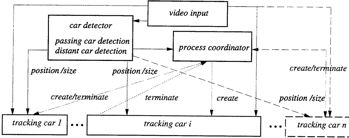
Figure 1: The hard real-time vision system for car detection and tracking.
