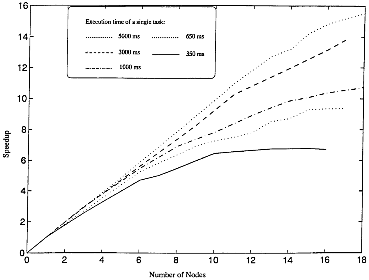
Figure 21: Speed-up factors of ANTS with extended average task execution times.
