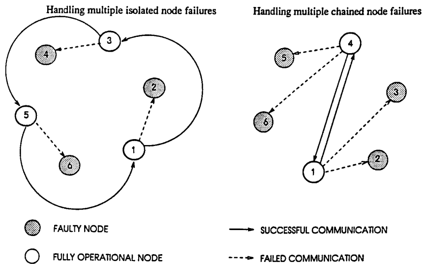
Figure 19: Detection of multiple isolated and multiple chained node failures.
