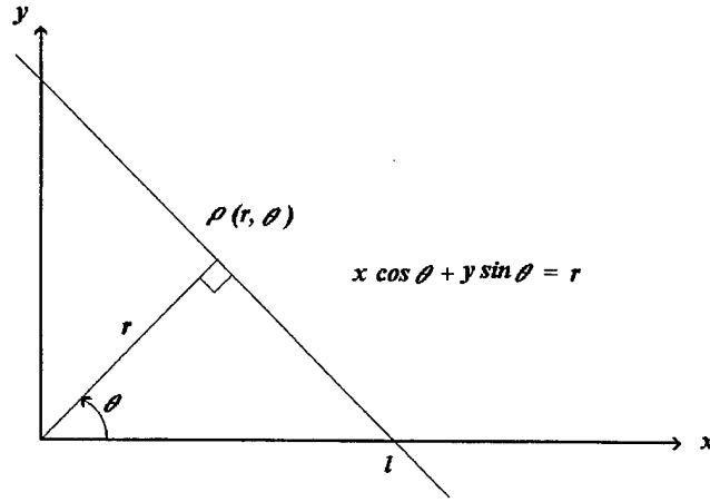
Figure 3. Parametric representation of lines using r and \theta .
