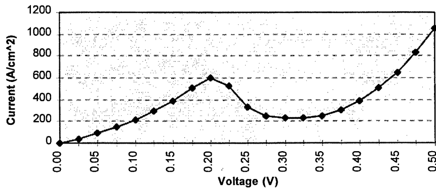
Current-Voltage Response of a DBRTD
