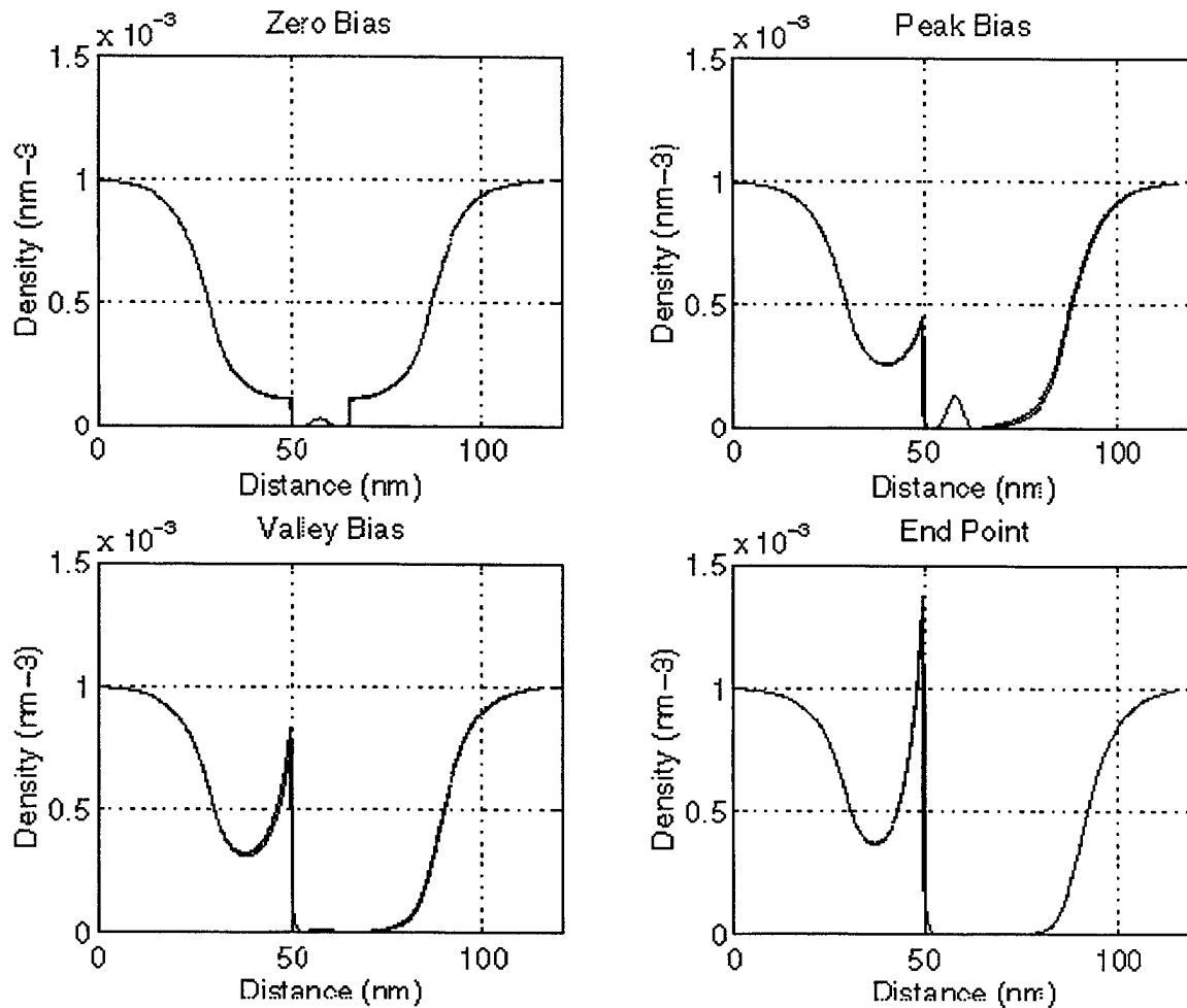
Figure 8 - Electron Density versus Location for the Thomas-Fermi and Poisson-Schrodinger Models.
