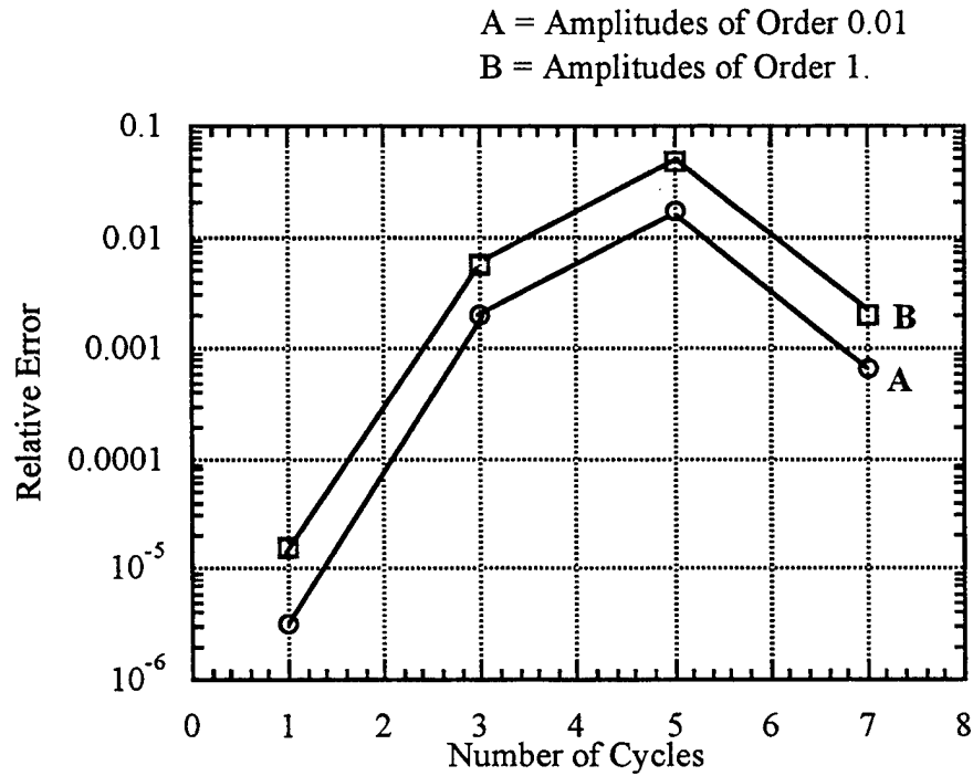
Figure 11-26. Variation of Error for Test Set One Based Upon Function Type for Plates Using the NUBS Method
