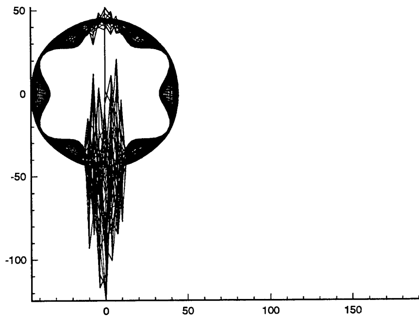
Figure 13-31. Engine Liner Mode Shape 1 Using Multiquadrics Method
