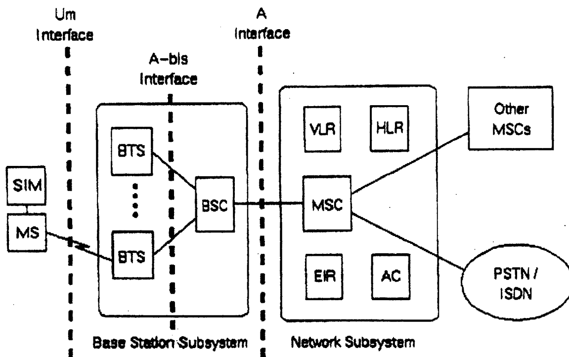
Figure 1. GSM Architecture
