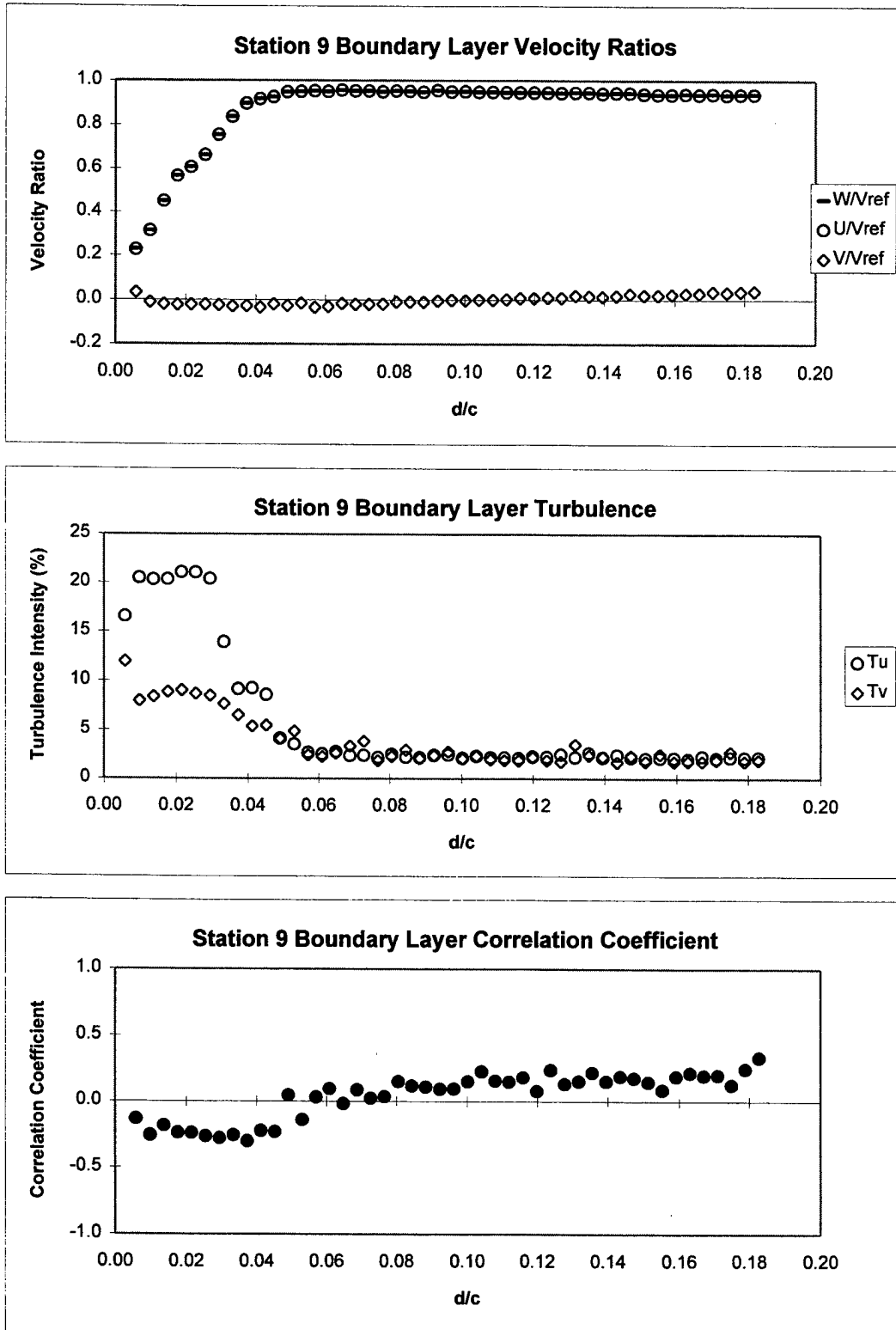
Figure 47. Station 9 Boundary Layer Survey Results at Re=380,000 .
