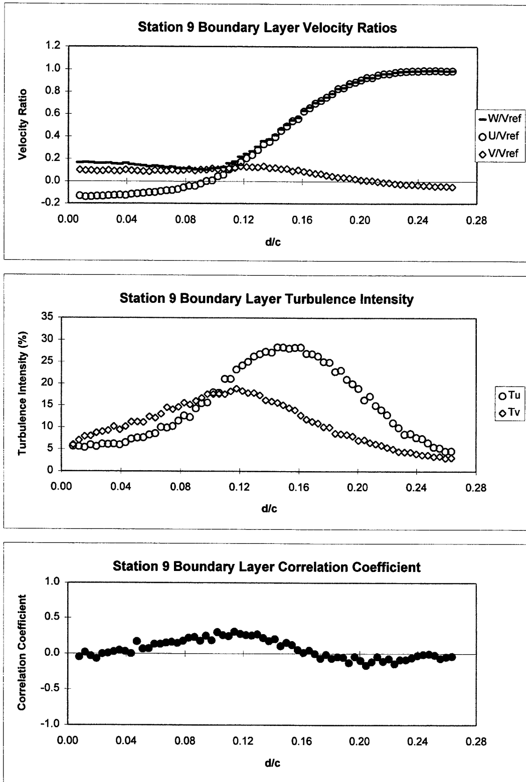
Figure 22. Station 9 Boundary Layer Survey Results at Re=640,000 .
