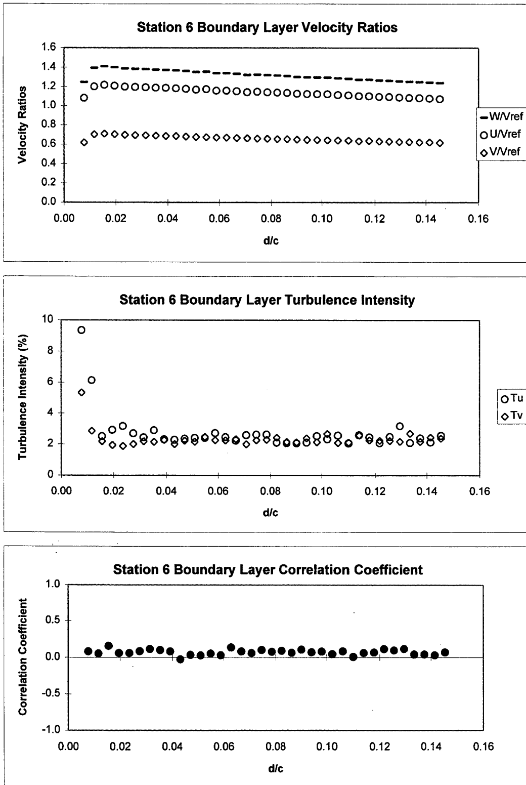
Figure 44. Station 6 Boundary Layer Survey Results at Re=380,000 .
