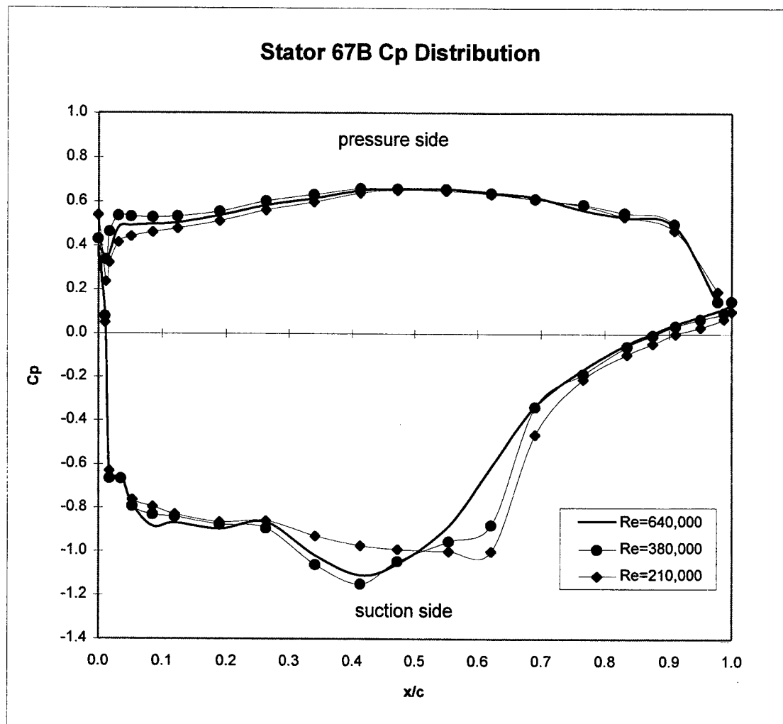
Figure 10. Experimental C_p Distributions.
