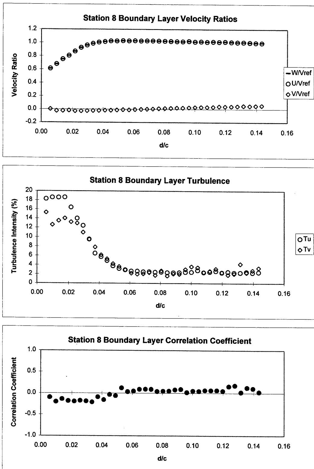
Figure 33. Station 8 Boundary Layer Survey Results at Re=210,000 .
