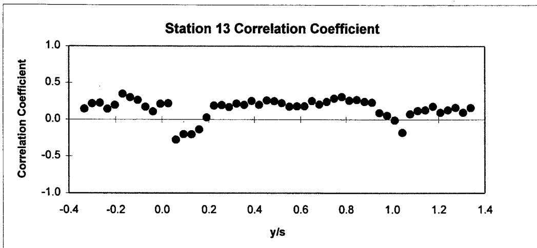
Figure 48. Station 13 Wake Survey Results at Re=380,000 .
