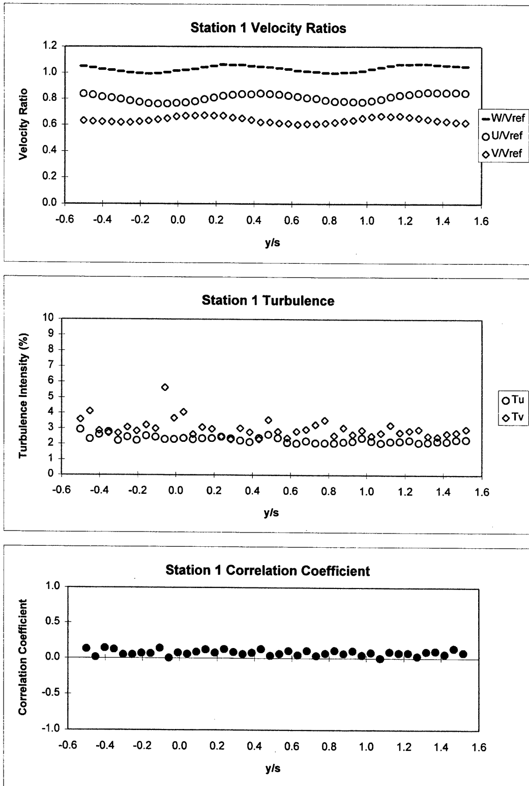
Figure 25. Station 1 Inlet Survey Results at Re=210,000 .
