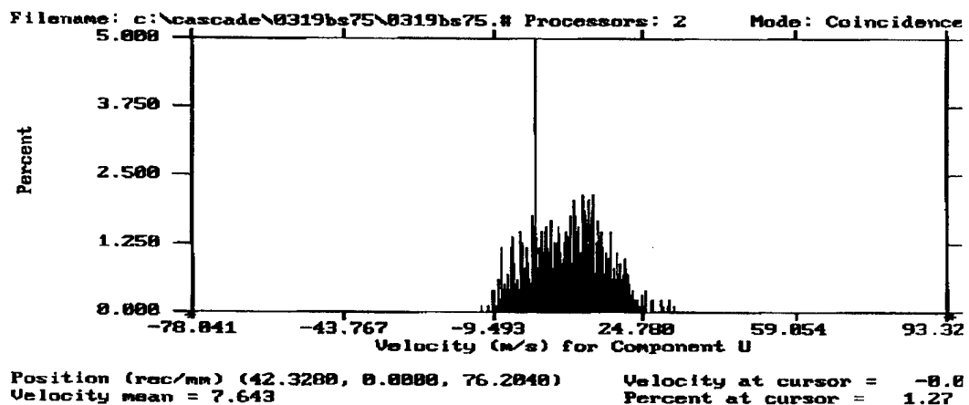
Figure 31b. Station 7.5 Axial Velocity Histograms.
