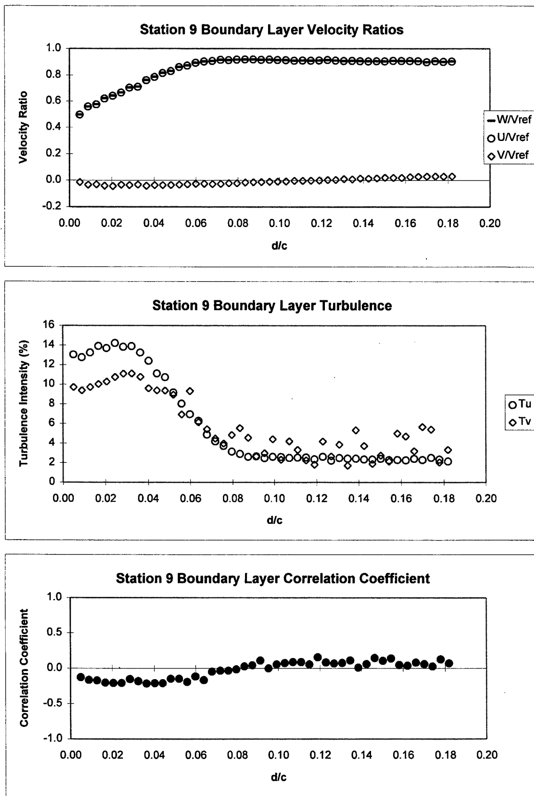
Figure 34. Station 9 Boundary Layer Survey Results at Re=210,000 .
