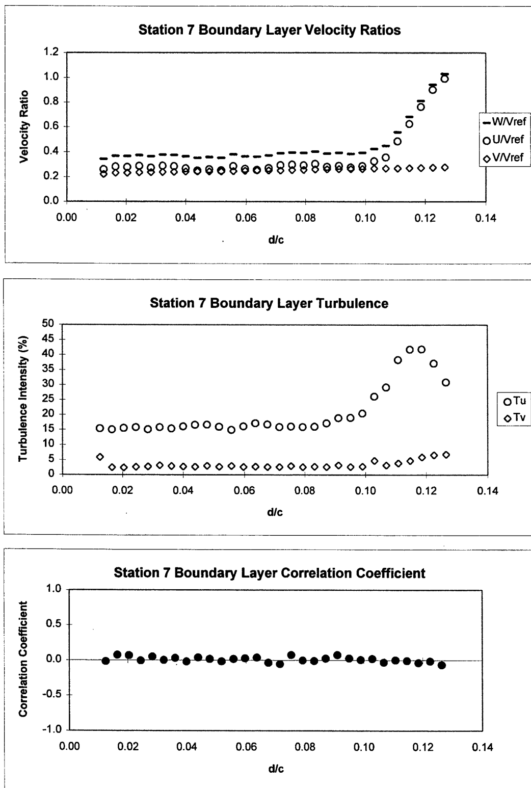
Figure 37a. Station 7 Boundary Layer Survey Results at Design Incidence. (Present Study)
