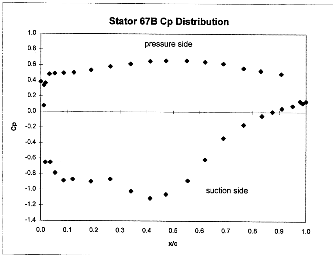
Figure 7. Experimental C_p Distribution at Re=640,000 .
