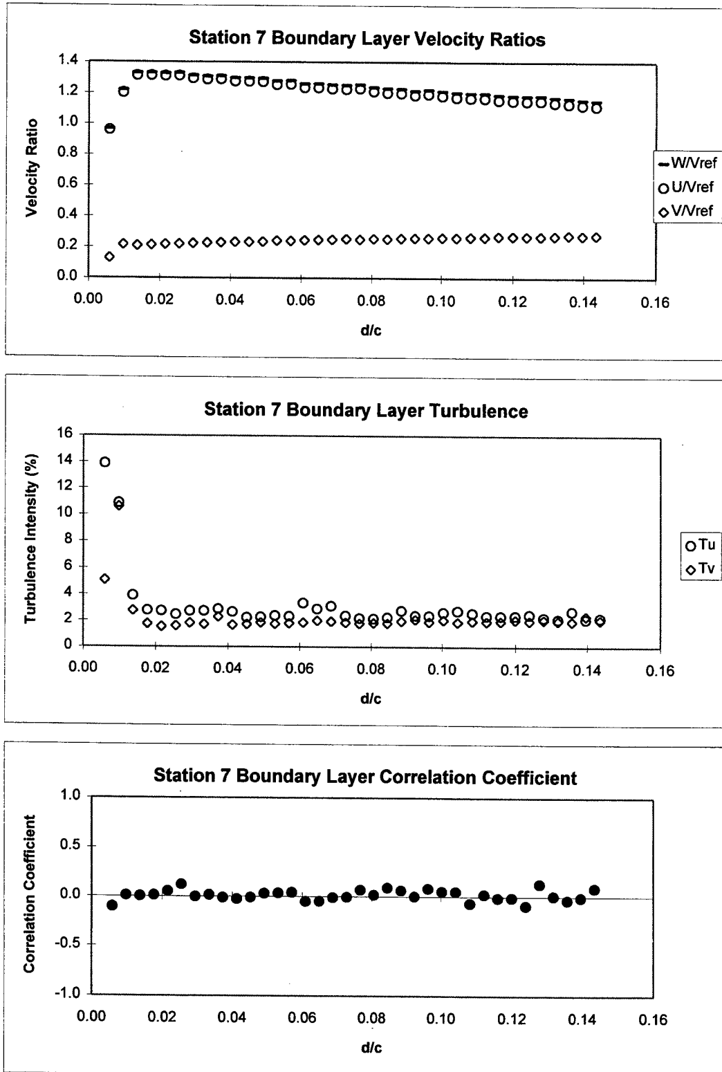
Figure 45. Station 7 Boundary Layer Survey Results at Re=380,000 .
