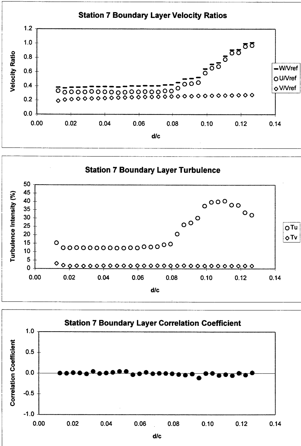
Figure 37b. Station 7 Boundary Layer Survey Results at Design Incidence. (From Ref. 3)
