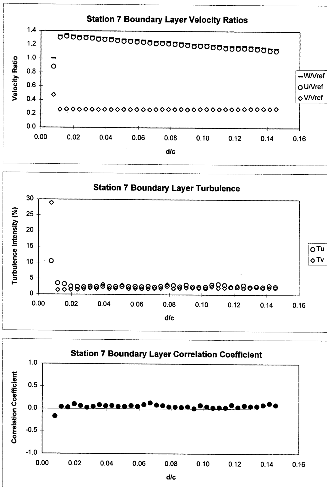
Figure 29a. Station 7 Boundary Layer Survey Results at Re=210,000 .
