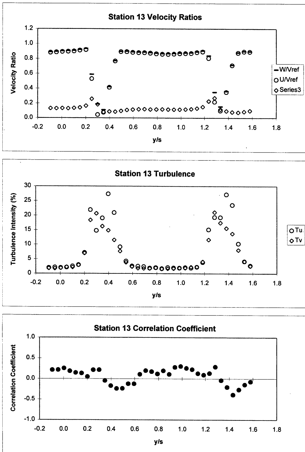
Figure 23. Station 13 Wake Survey Results at Re=640,000 .
