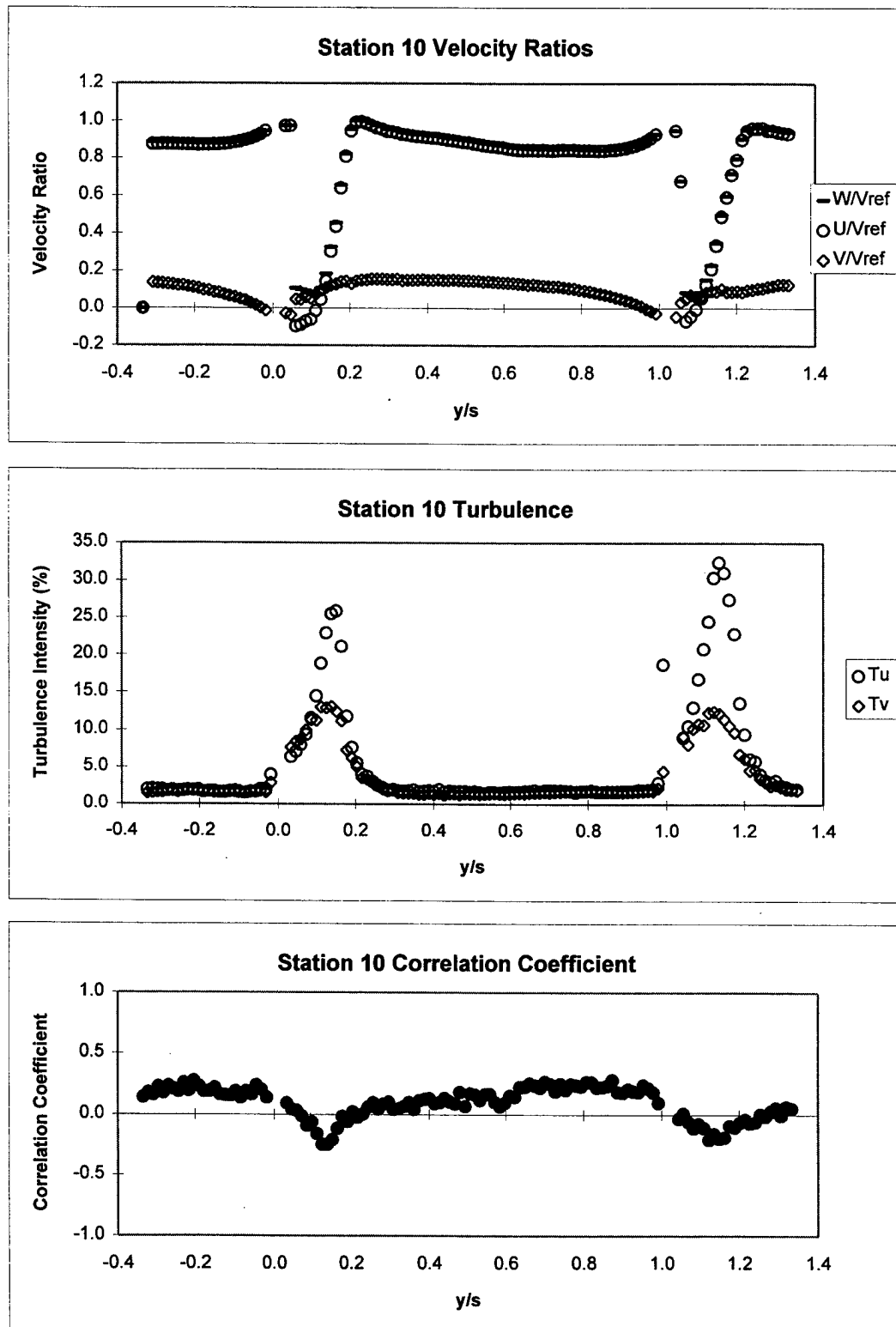
Figure 19. Station 10 Passage Survey Results at Re=640,000 .
