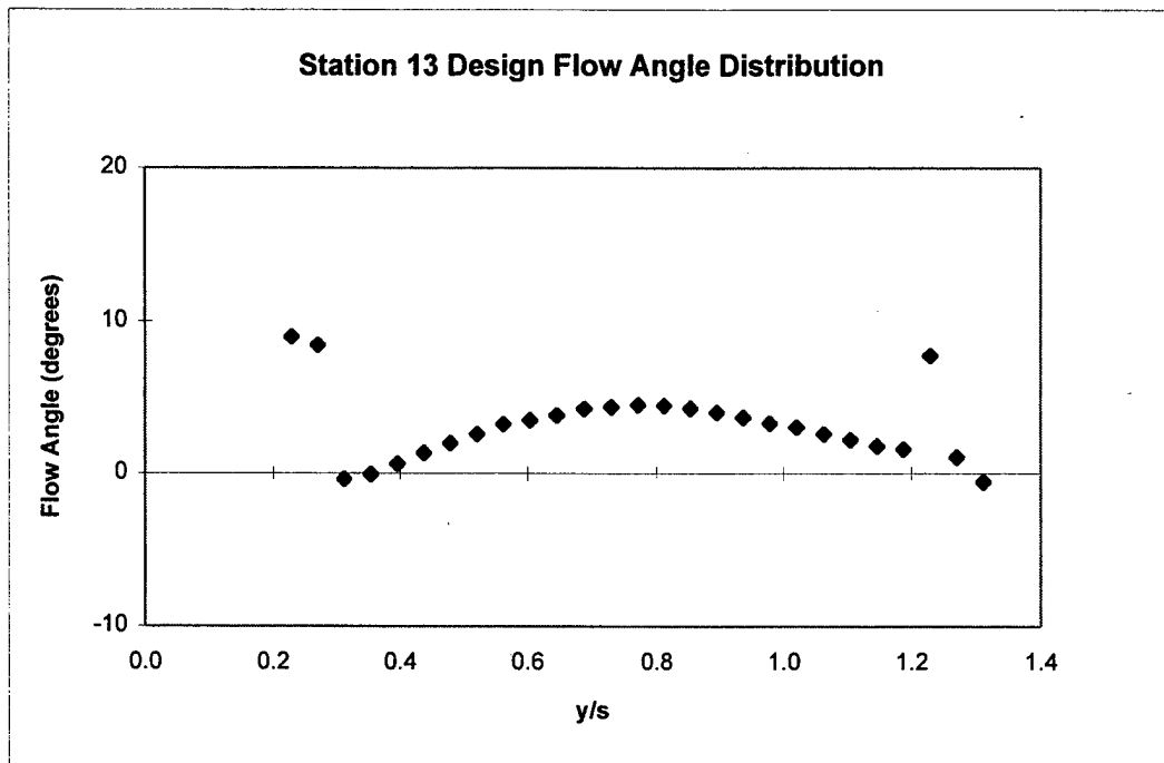
Figure 24a. Station 13 Wake Flow Angle Distribution at Design Incidence.
