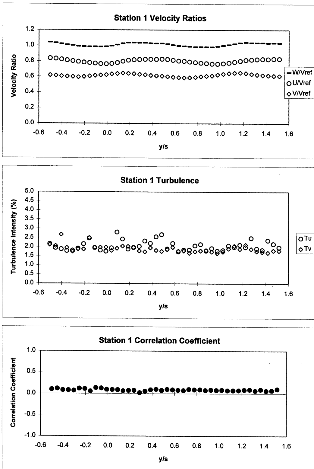
Figure 15. Station 1 Inlet Survey Results at 3000 Data Points.
