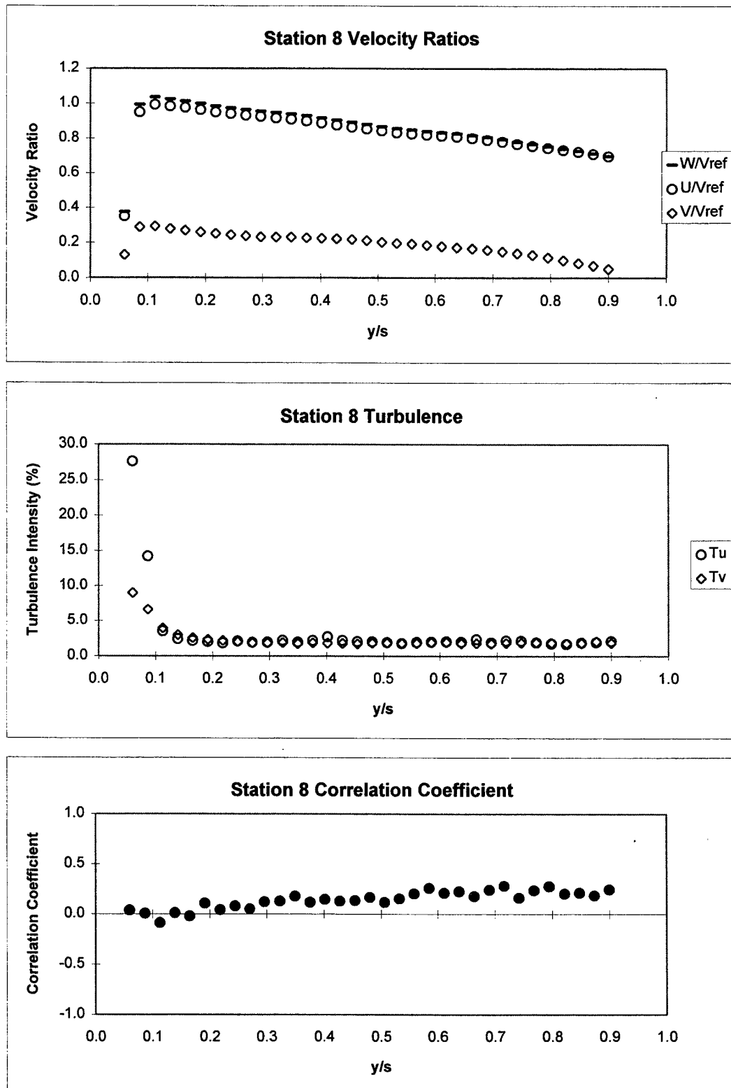
Figure 18. Station 8 Passage Survey Results at Re=640,000 .
