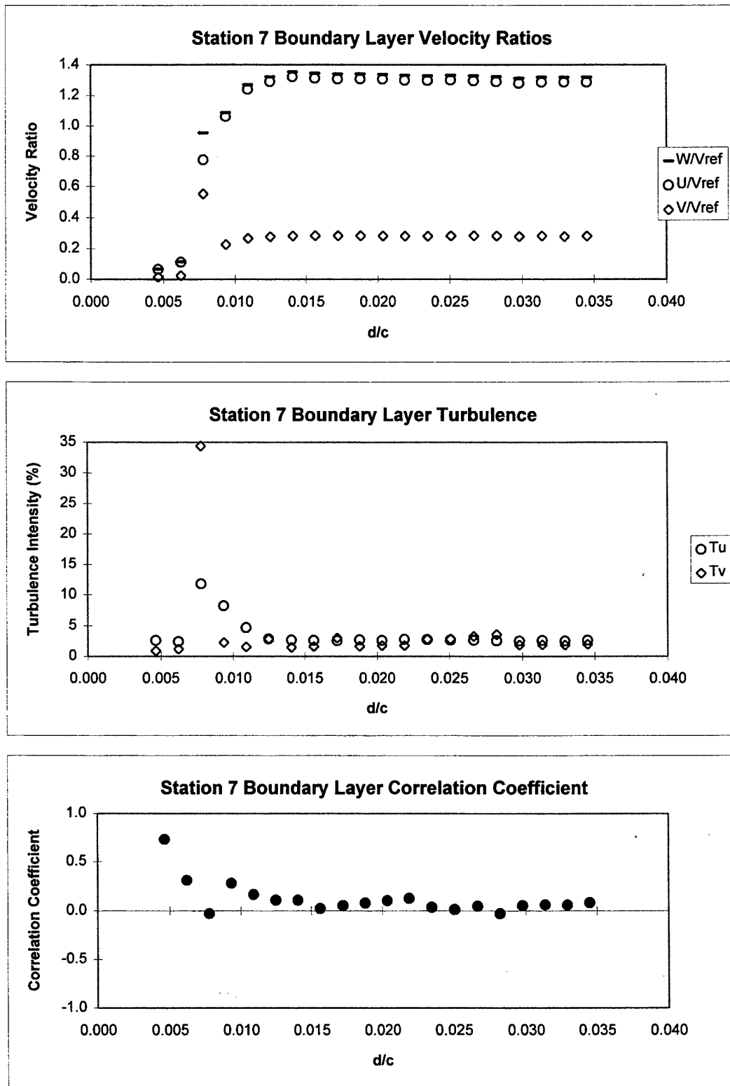
Figure 29b. Station 7 Boundary Layer Survey Results at Re=210,000 .
