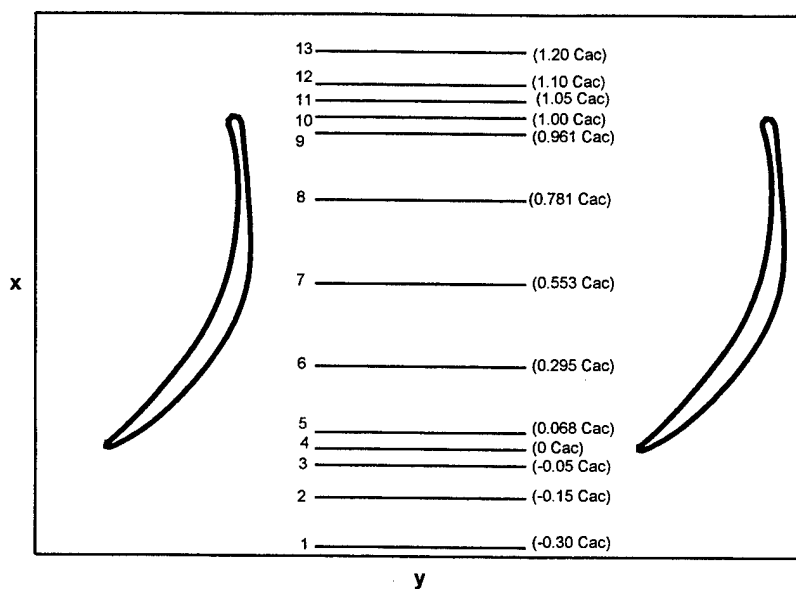
Figure 4. Survey Station Numbering and Position.
