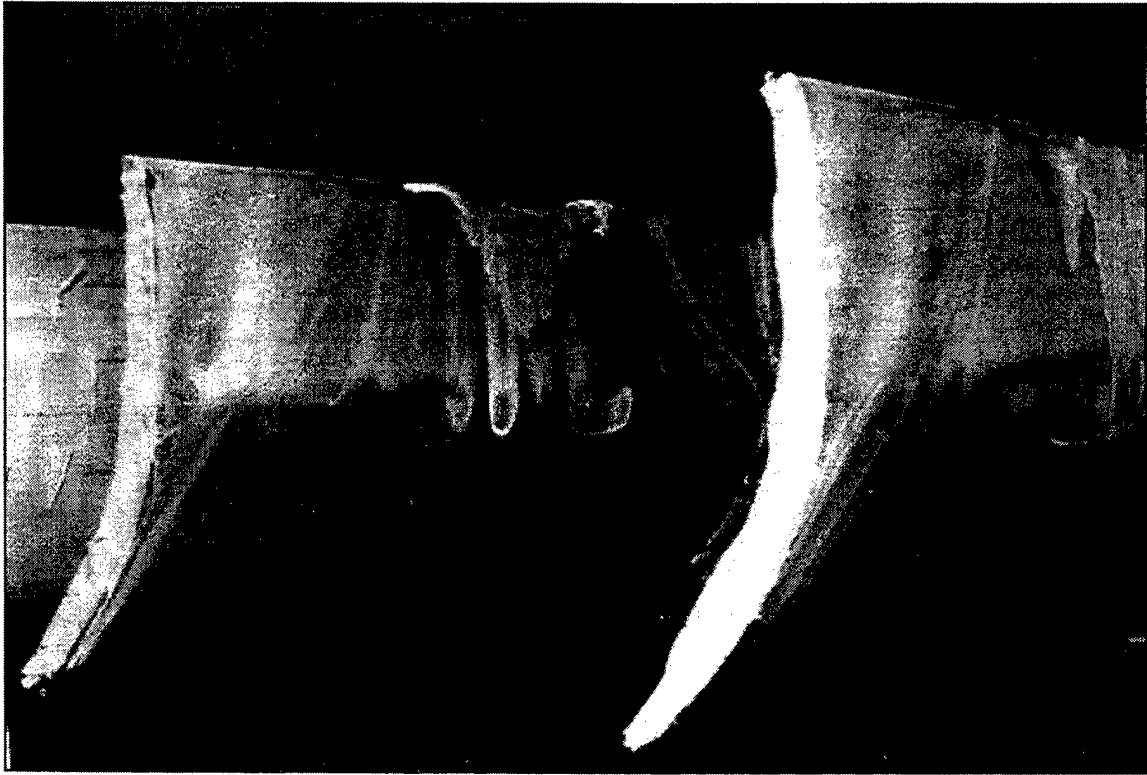
Figure 12. Blade Surface Flow Visualization at Re=380,000 .
