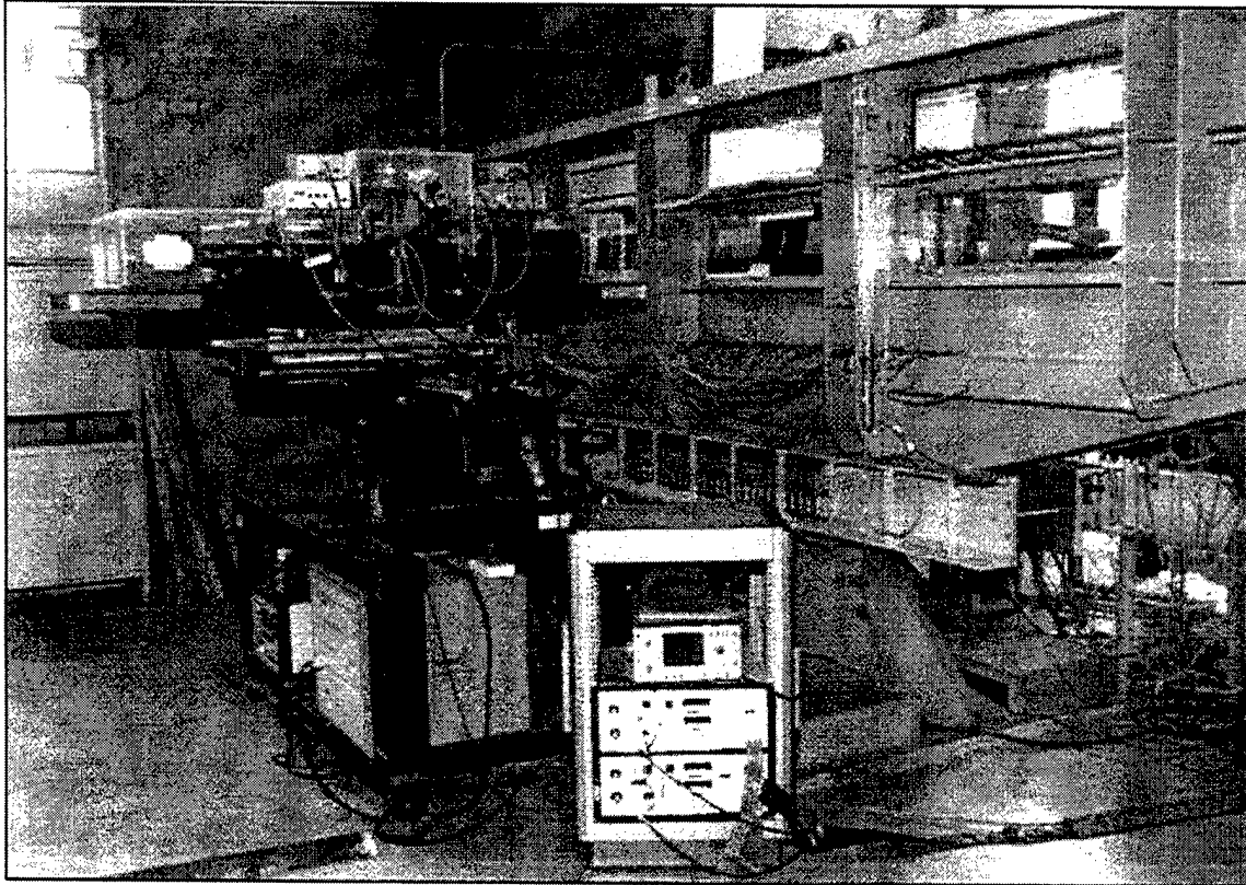
Figure 5. LDV System.
