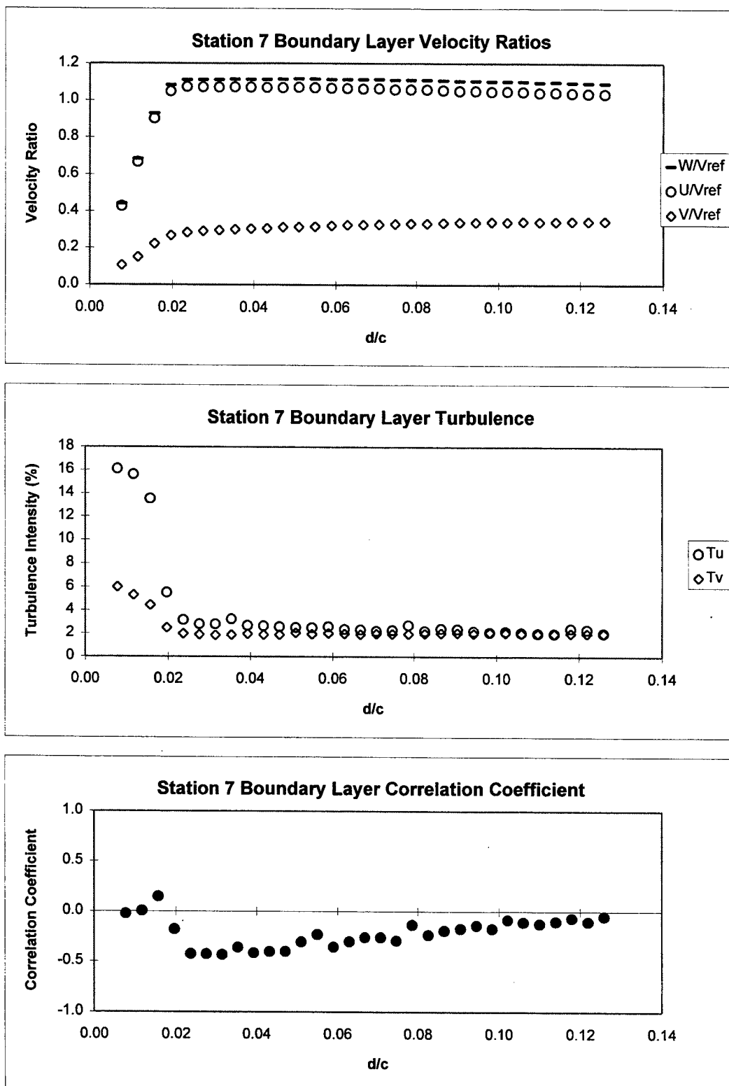
Figure 21. Station 7 Boundary Layer Survey Results at Re=640,000 .
