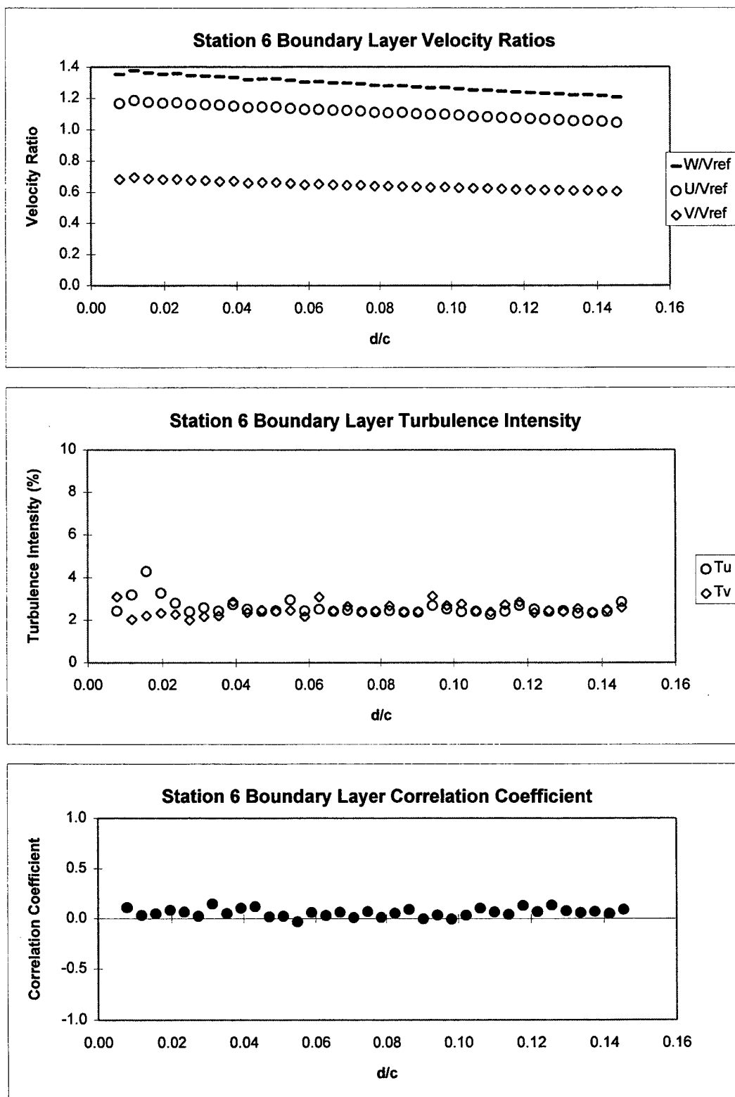
Figure 28. Station 6 Boundary Layer Survey Results at Re=210,000 .
