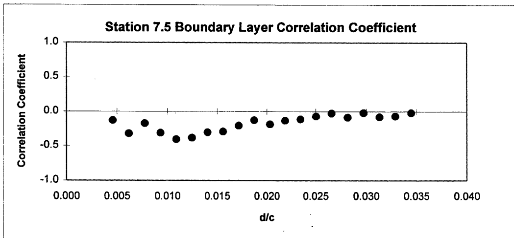
Figure 31a. Station 7.5 Boundary Layer Survey Results at Re=210,000 .
