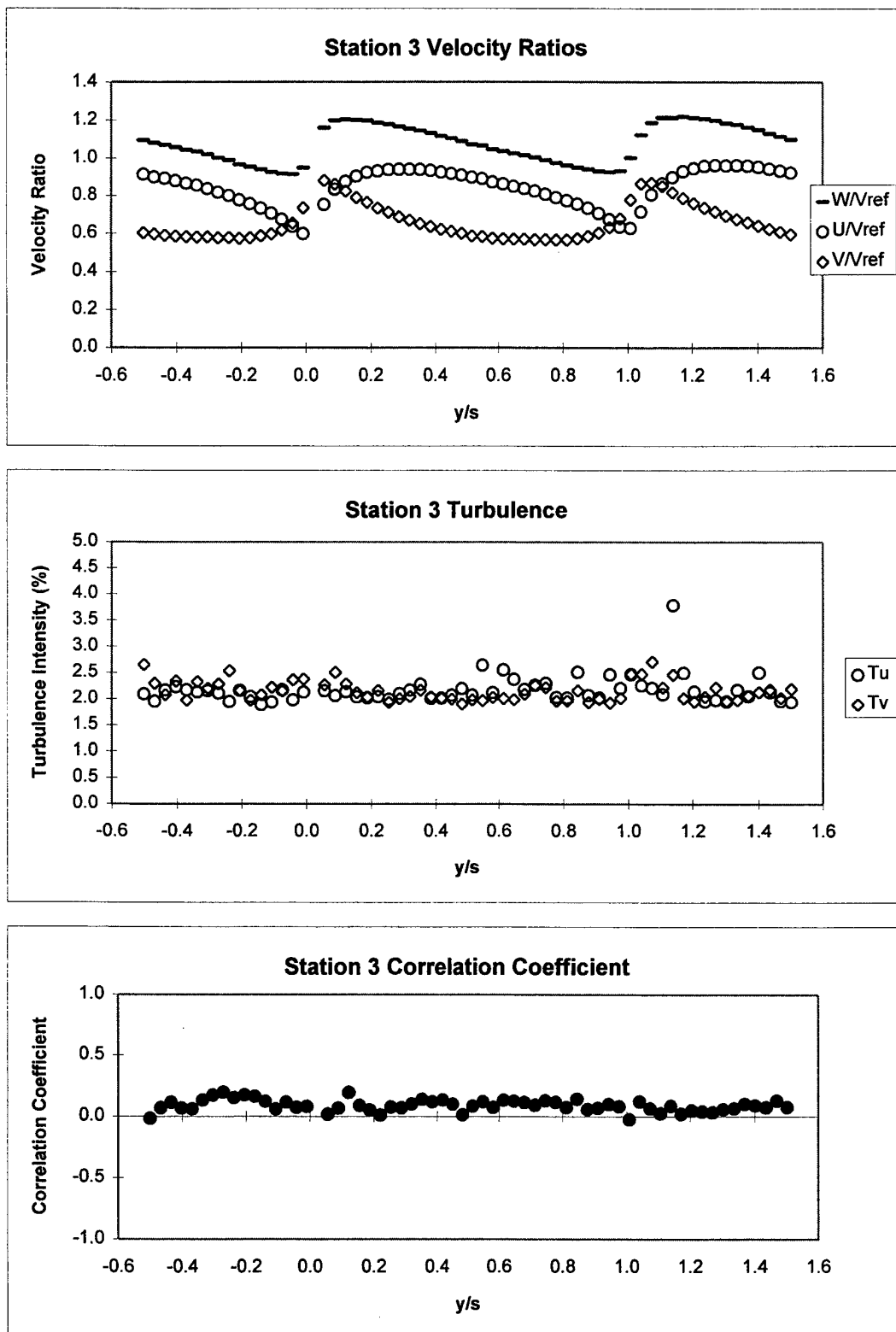
Figure 42. Station 3 Inlet Survey Results at Re=380,000 .
