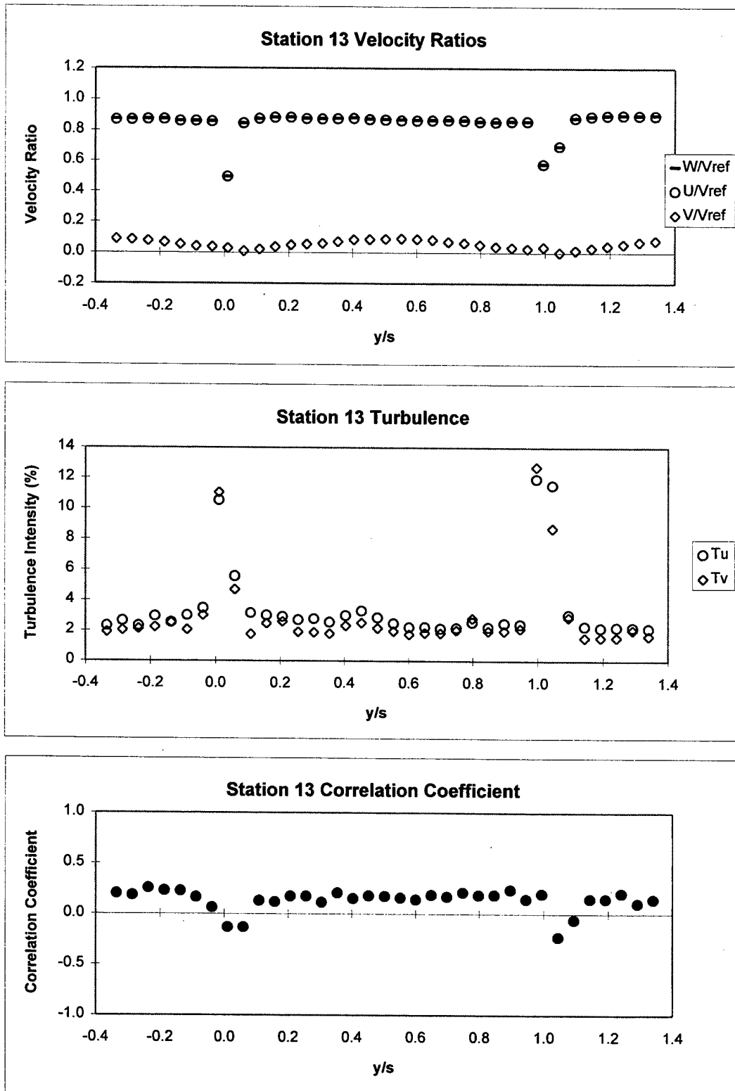
Figure 35. Station 13 Wake Survey Results at Re=210,000 .
