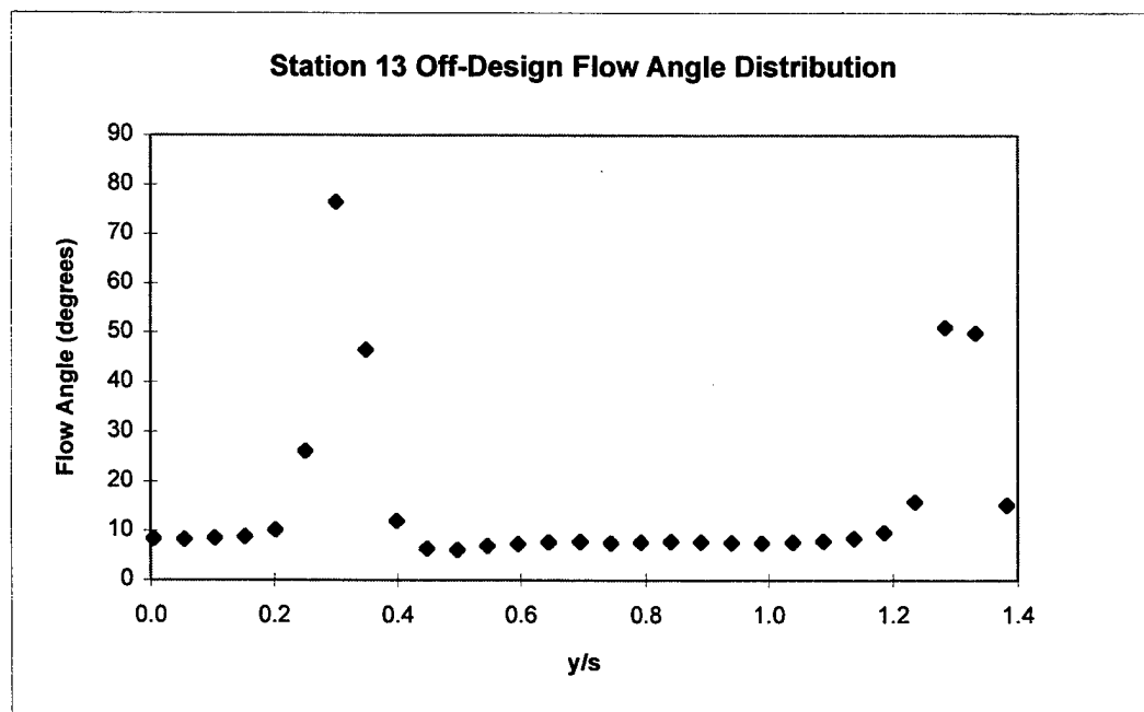
Figure 24b. Station 13 Wake Flow Angle Distribution at Off-Design Incidence.
