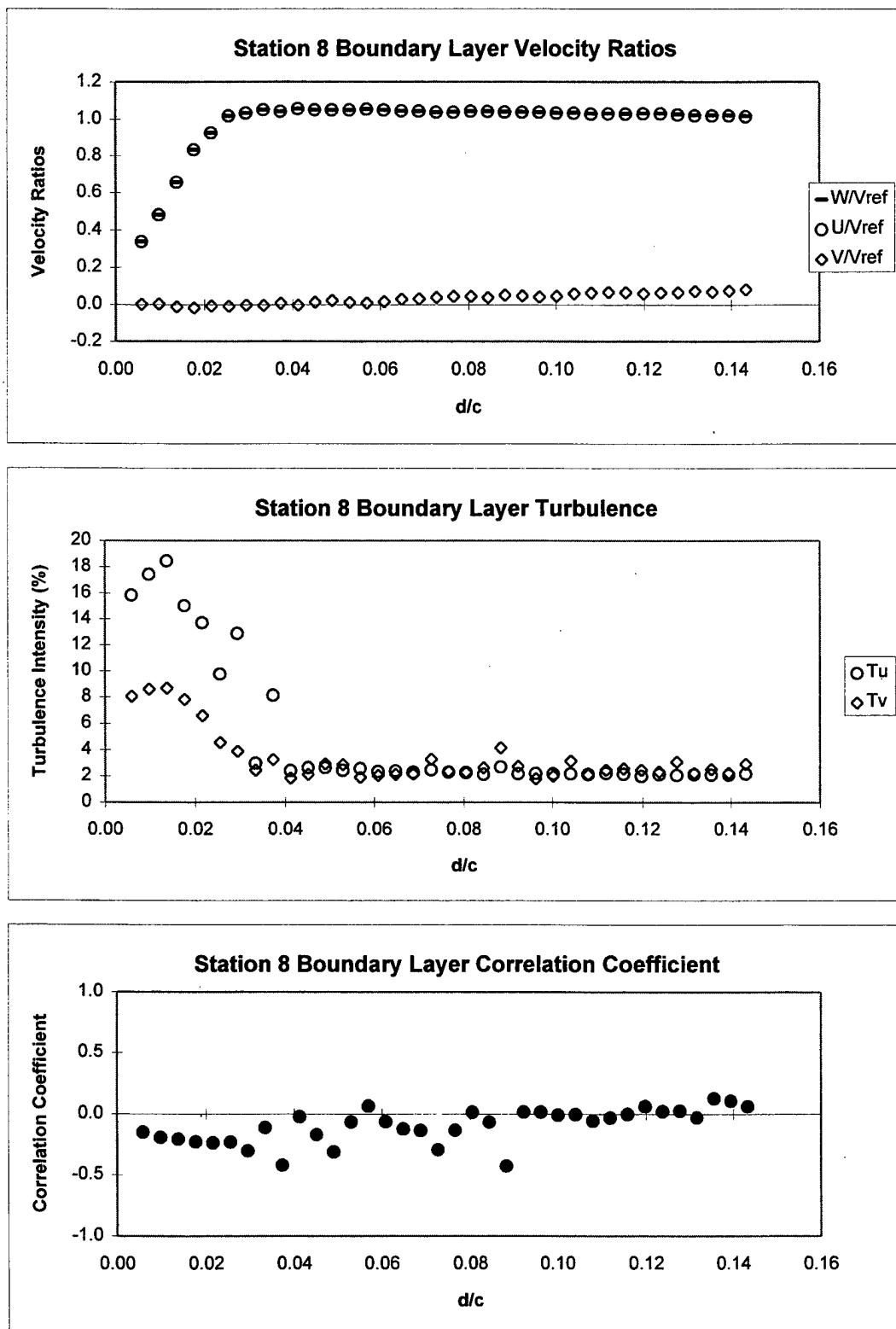
Figure 46. Station 8 Boundary Layer Survey Results at Re=380,000 .
