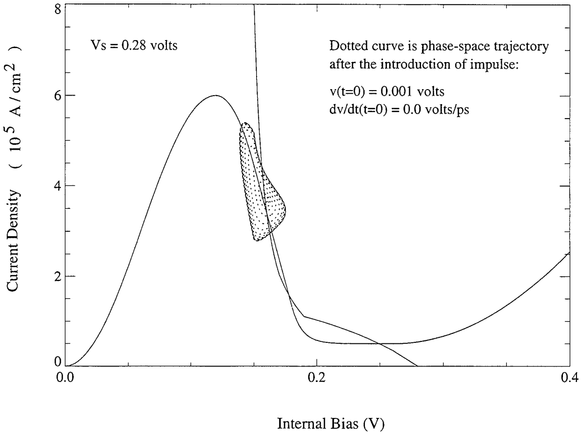
FIG. 13. Forward-sweep current-density phase-space trajectory for V_s = 0.28 V.
