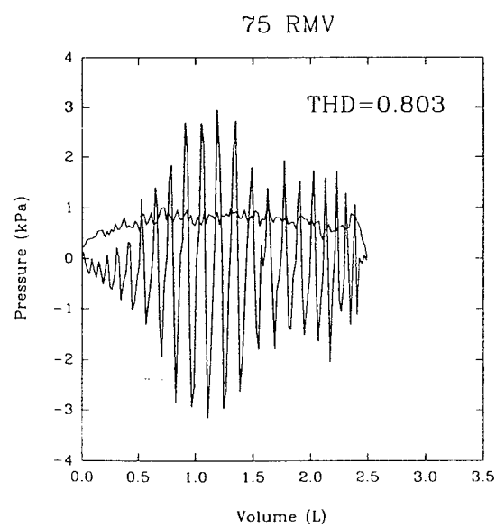
Figure 5-1. Total Harmonic Distortion (THD) and Regulator Chatter
