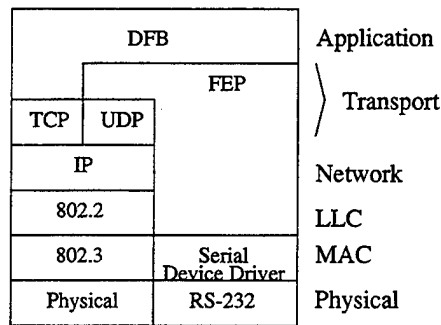
FIGURE 1. Full DFB protocol stack.
