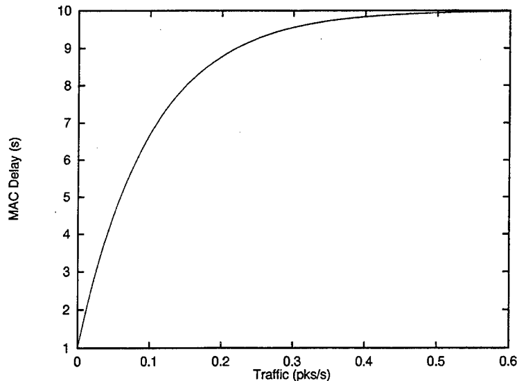
FIGURE 11. Expected MAC Delay for D_{\rho_i} = 10 s vs. traffic rate.
