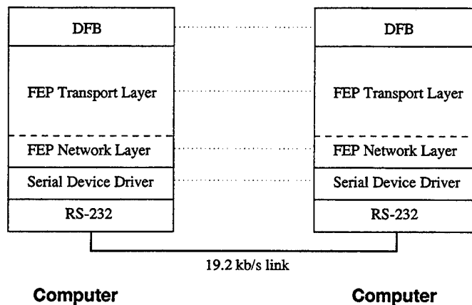
FIGURE 2. Partial DFB protocol stack with RS-232 interconnection.
