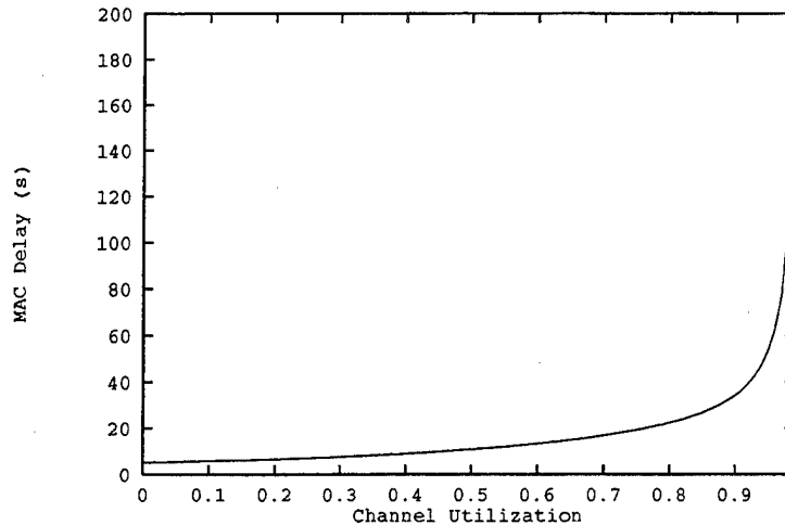
FIGURE 8. MAC delay vs. net utilization
