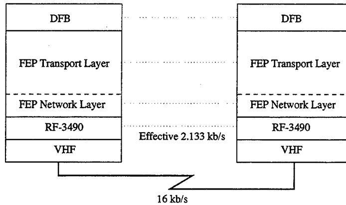
FIGURE 6. Peer-to-peer DFB communication with simplified stacks.
