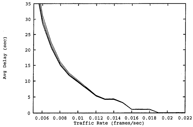
FIGURE 14. Traffic rate vs. average delay, \rho = 0.4 , C = 2133 b/s.
