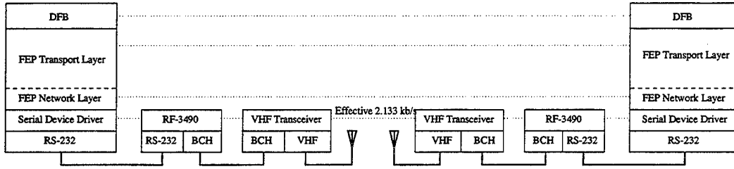
FIGURE 4. Peer-to-peer DFB Communication via Radio Link.
