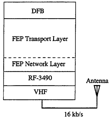
FIGURE 5. Simplified DFB stack.
