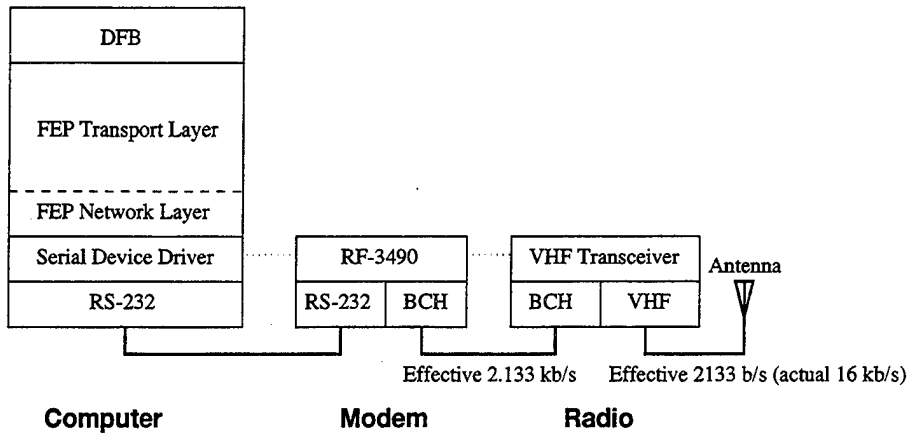
FIGURE 3. Partial DFB protocol stack with radio interconnection.
