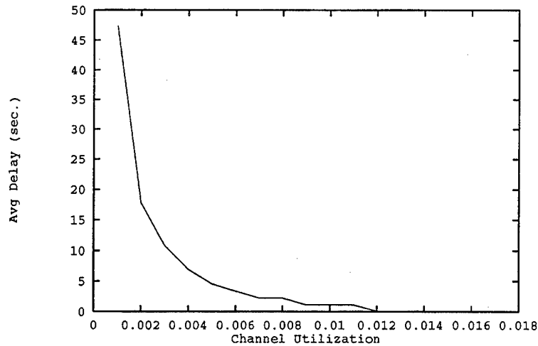
FIGURE 16. Utilization vs. average delay, \lambda = 0.03 , C = 2133 b/s.
