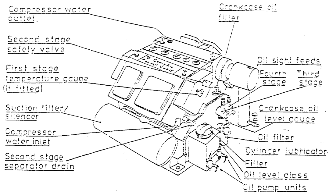
Compressor Description
