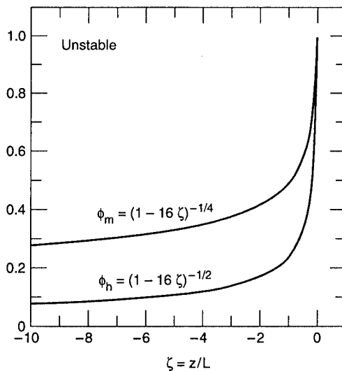
Figure 4. Nondimensional wind speed and scalar gradients, \phi_m and \phi_h , as functions of stability for unstable conditions.
