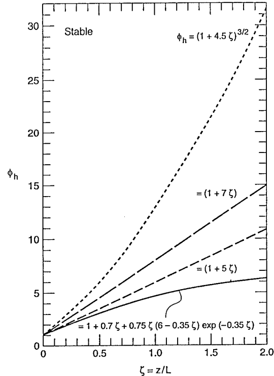
Figure 5. Various suggestions for the functional form of the nondimensional wind speed ( \phi_m ) and scalar ( \phi_h ) gradients for stable conditions.
