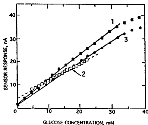
Fig. 7. Calibration curve of glucose biosensor with a PVC coating in phosphate buffer before plasma test (curve 1), calibration curve of the sensor in bovine blood plasma (curve 2) and in phosphate buffer obtained after plasma test (curve 3).
