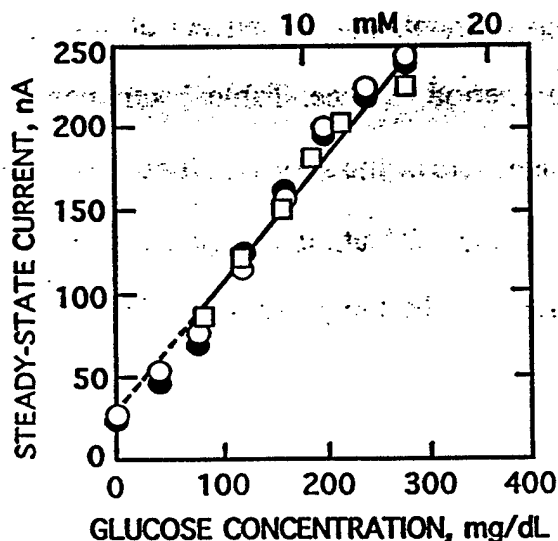
FIG. 5 Calibration curve of glucose biosensor with standard polycarbonate membrane in bovine serum (□) compared with the calibration data obtained before (○) and after (●) serum test.
