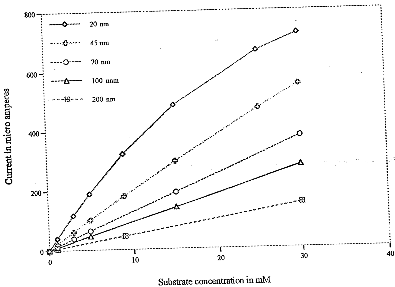
Figure. 3 Calibration plot obtained from numerical solutions for a homogeneous distribution of enzyme [Equation 32].
