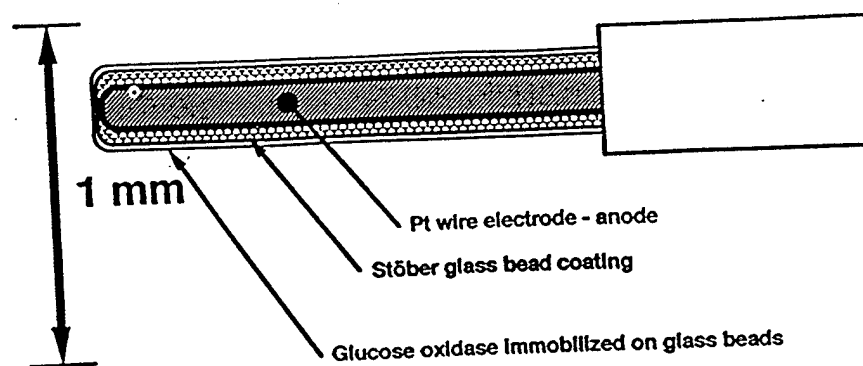
FIG. 2 Schematic of the glass-bead-coated glucose enzyme electrode
