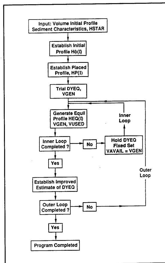
Figure 2. Flow diagram for equilibrium beach profile development
