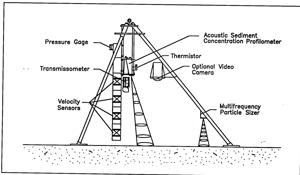
Figure 14. Acoustic resuspension measurement system
