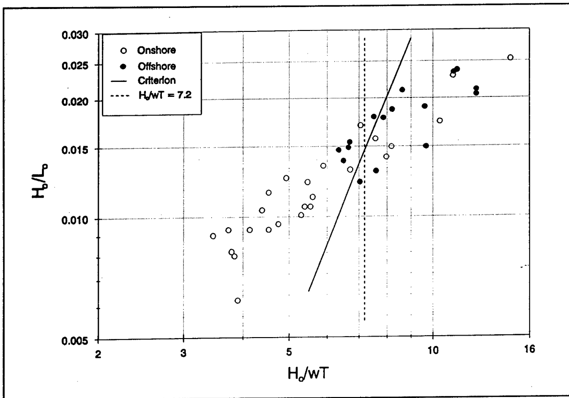
Figure 5. Prediction of cross-shore movement of longshore bar or nearshore berm
