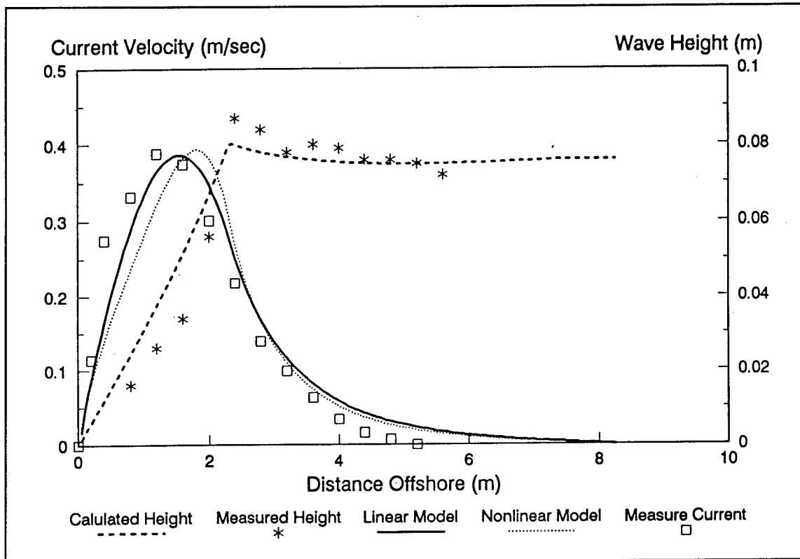
Figure 4. NMLONG longshore current and wave distributions across the surf zone
