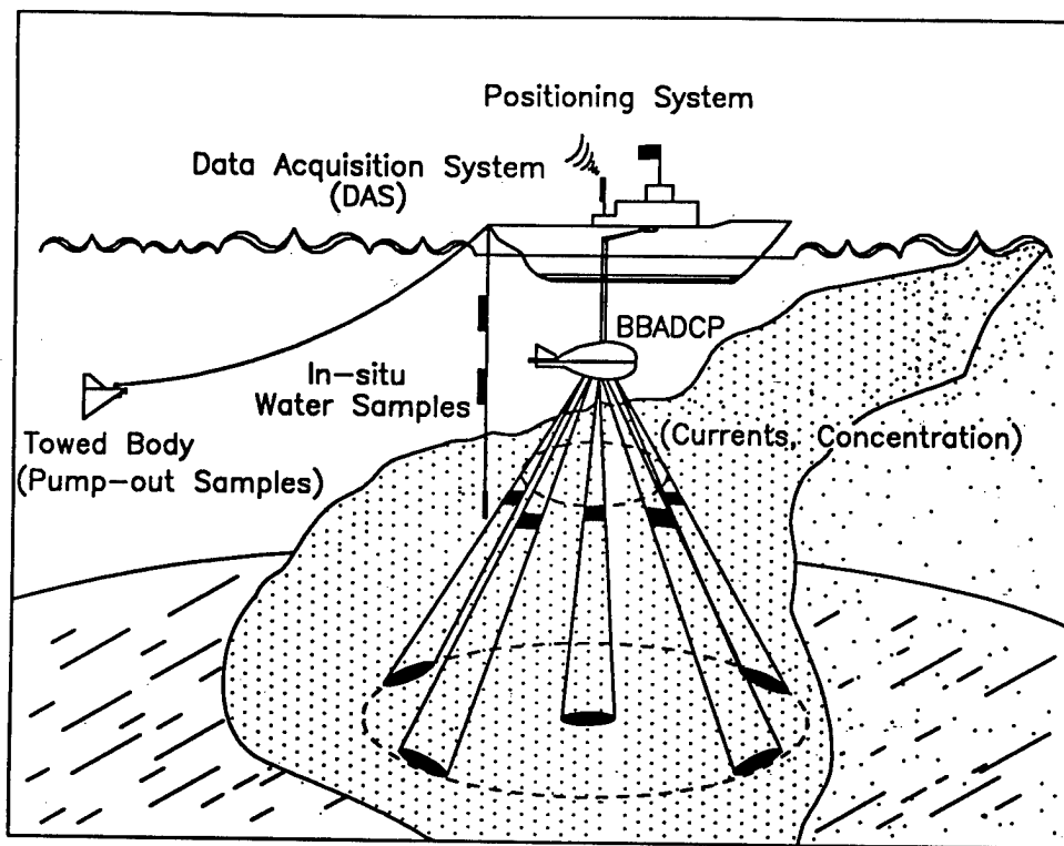
Figure 13. Plume measurement system
