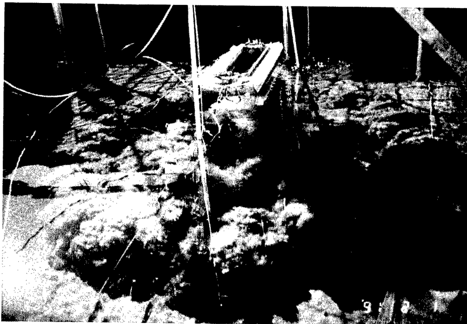
Figure 16. Model tests of open-water disposal from a stationary barge
