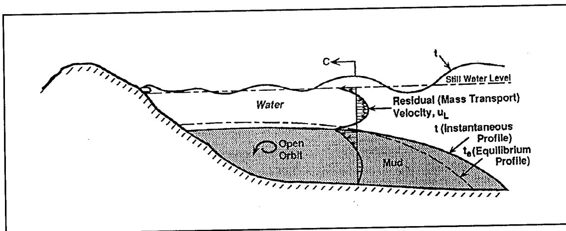
Figure 11. Shoreward migration of mudbank due to Stokes' drift
