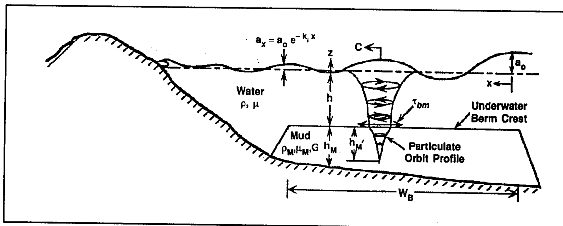
Figure 10. Schematic of wave propagating over an underwater mud berm
