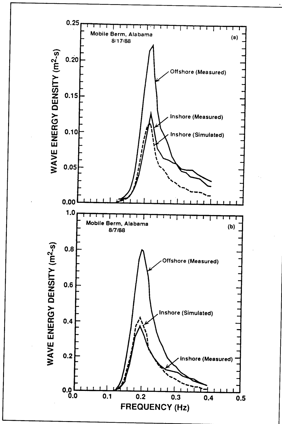
Figure 12. Comparison between measured and model-simulated inshore wave spectra at Mobile nearshore berm site for two offshore wave conditions: (a) H_{max} = 0.9 m and (b) H_{max} = 1.5 m
