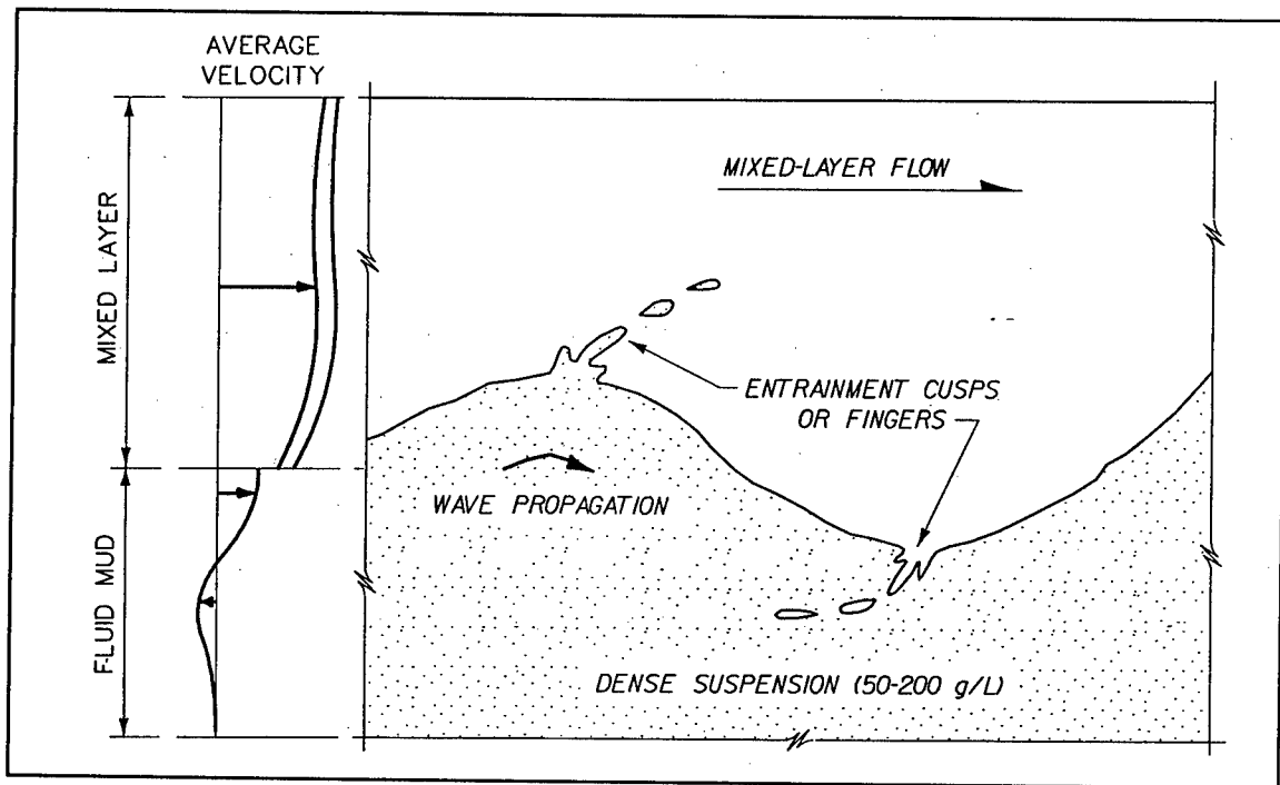
Figure 8. Entrainment of fluid mud into a mixed layer by internal instabilities generated by unidirectional flow
