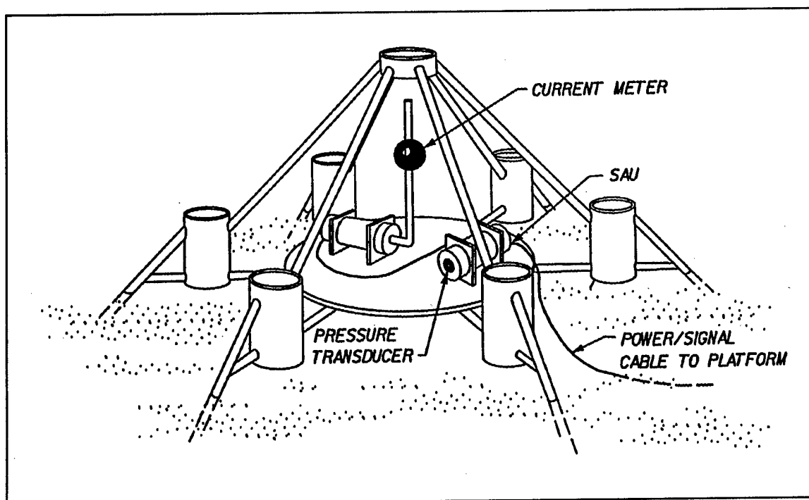
Figure 21. WES-developed PUV gauge used for monitoring waves and currents
