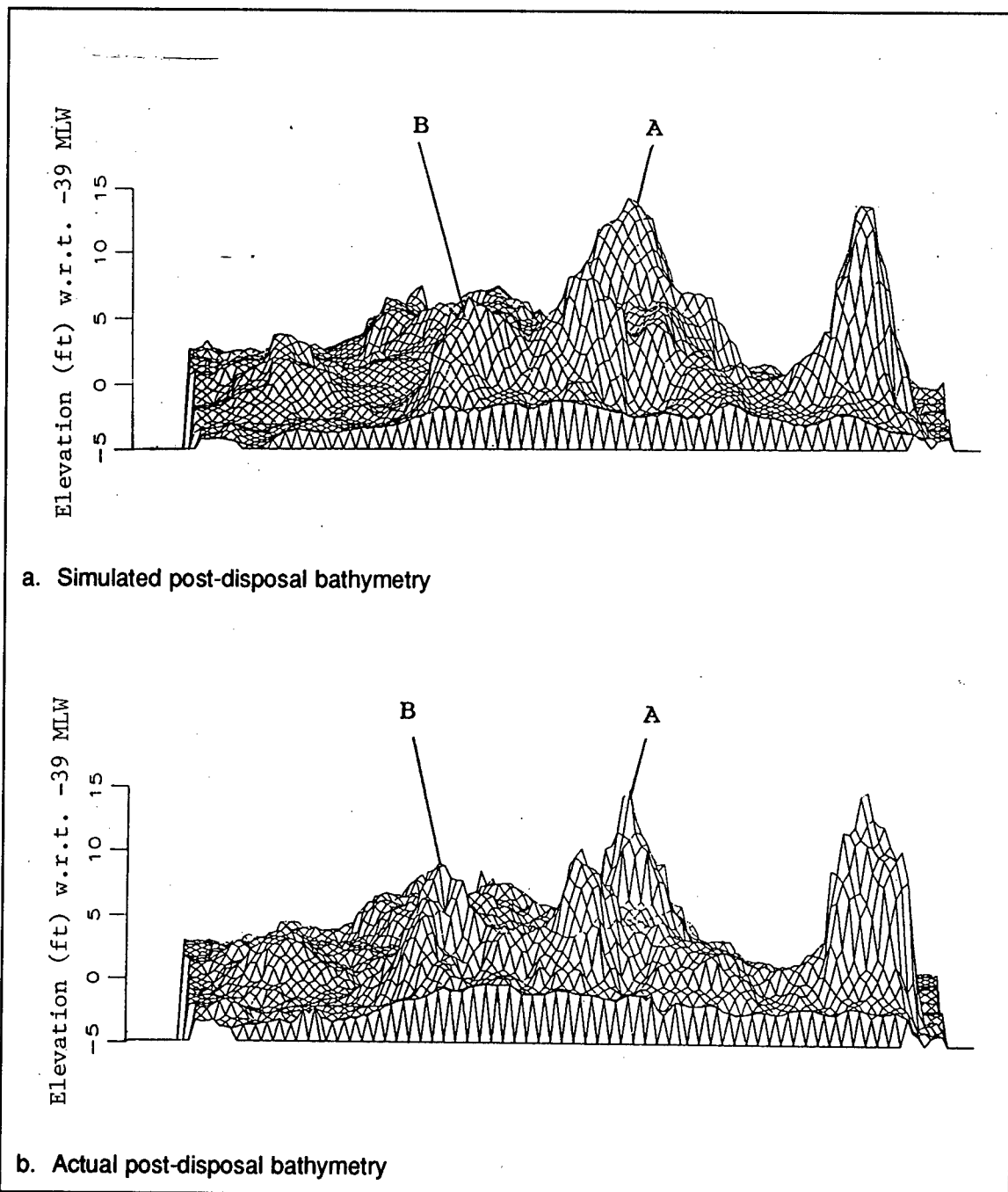
Figure 18. Cross sections of post-disposal survey for Wilmington, NC, offshore dredged material disposal site, April 1991 (after Moritz, unpublished manuscript)
