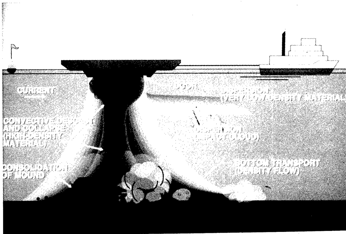
Figure 15. Schematic of barge disposal of dredged material in open water
