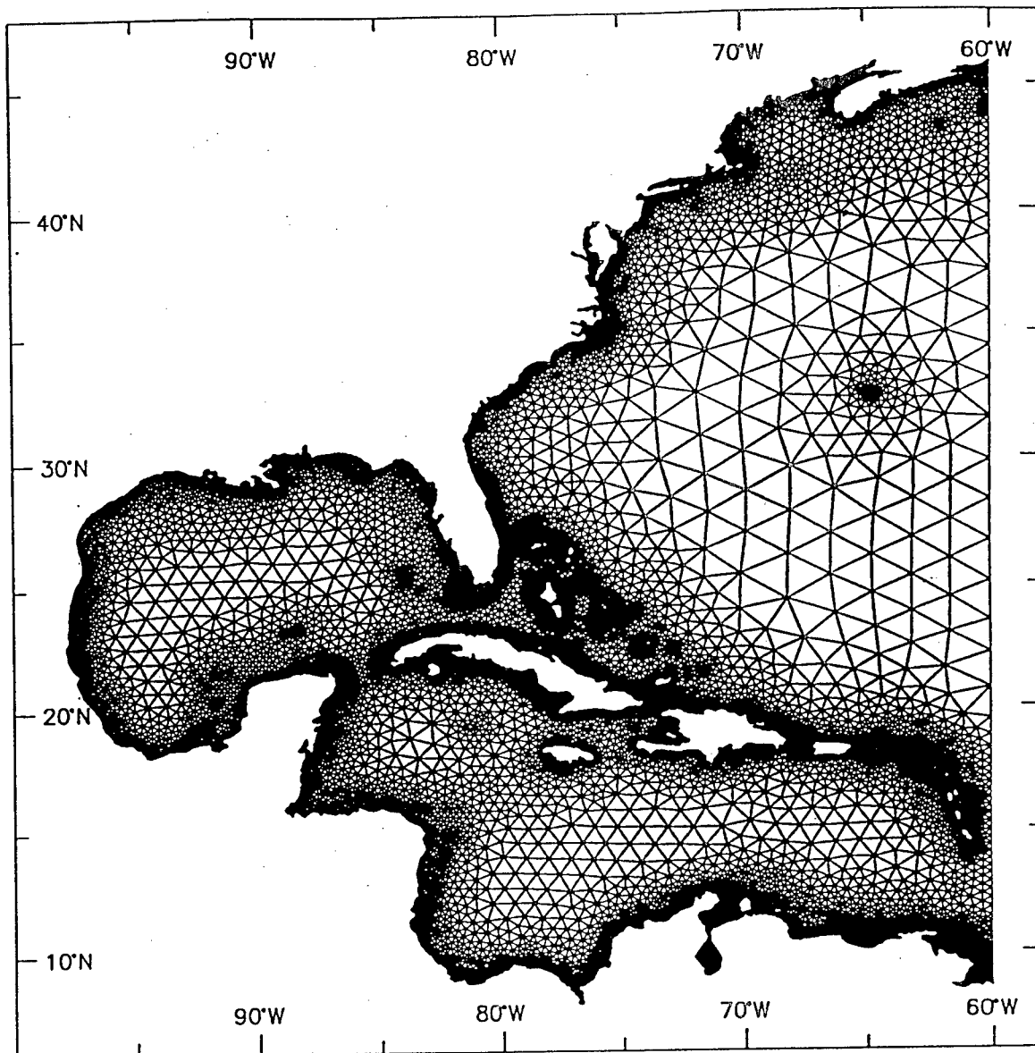
Figure 17. Example of domain size and grid spacing for ADCIRC (after Westerink, Luetlich, and Scheffner (1993))
