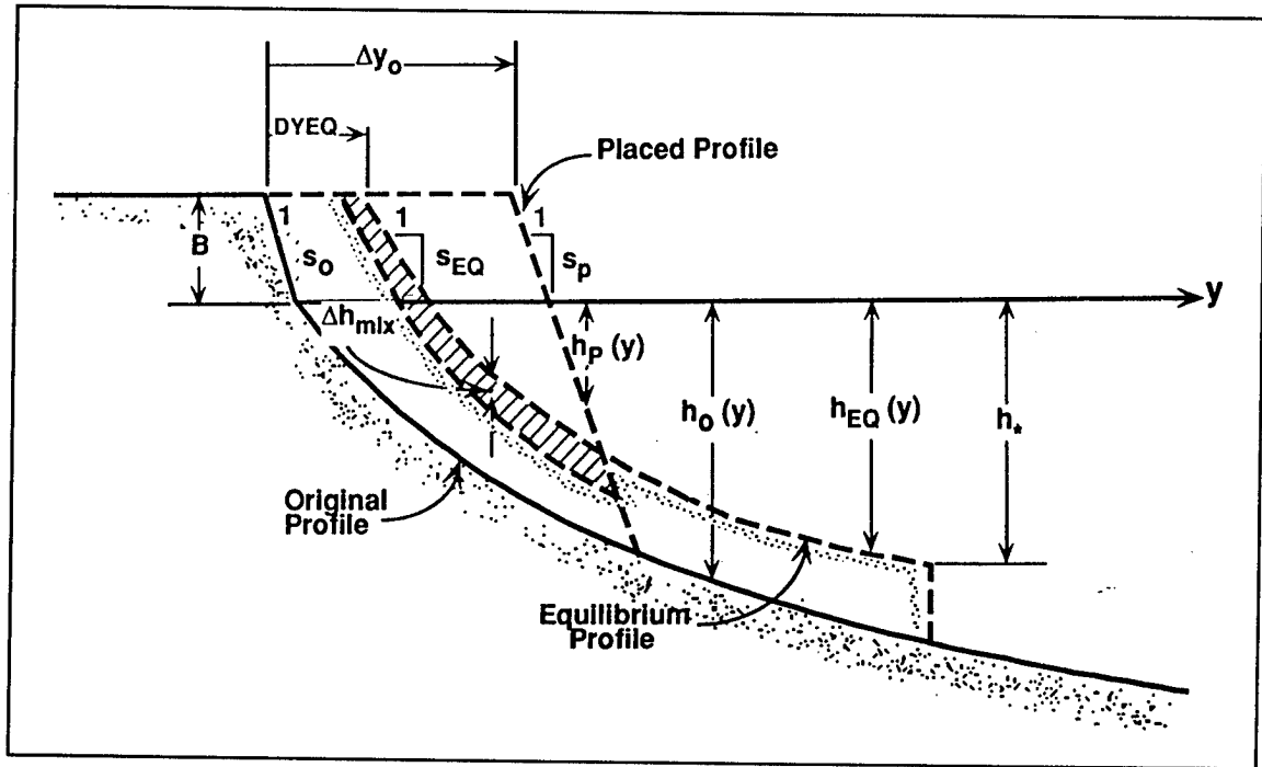
Figure 1. Definition sketch for equilibrium beach profile
