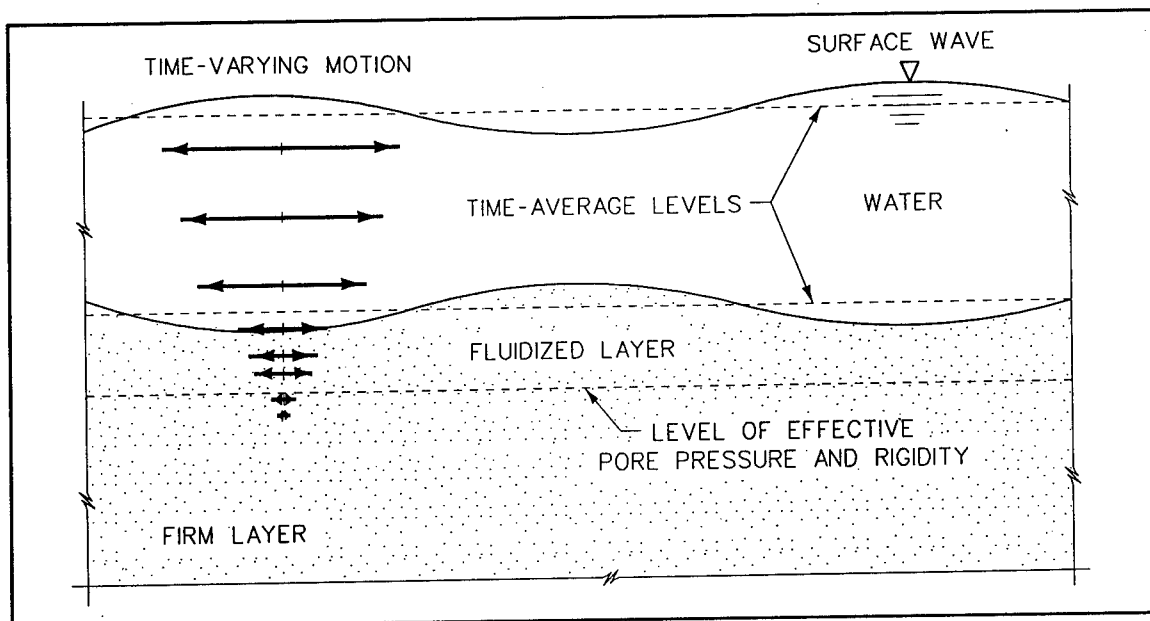
Figure 9. Mud layer fluidized by surface gravity waves
