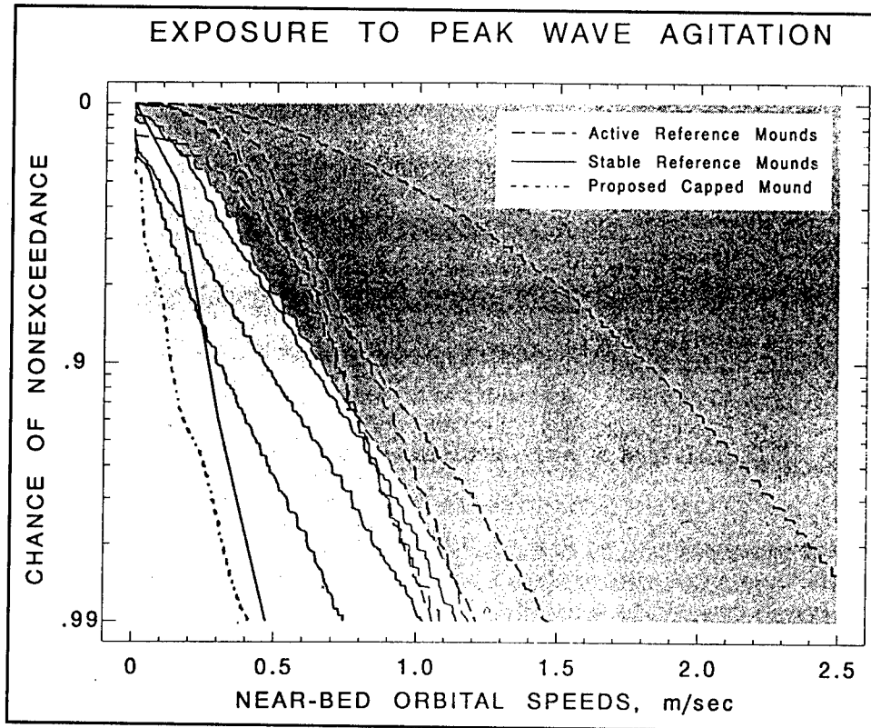
Figure 24. Frequency of near-bed oscillatory peak speeds (NOPS)
