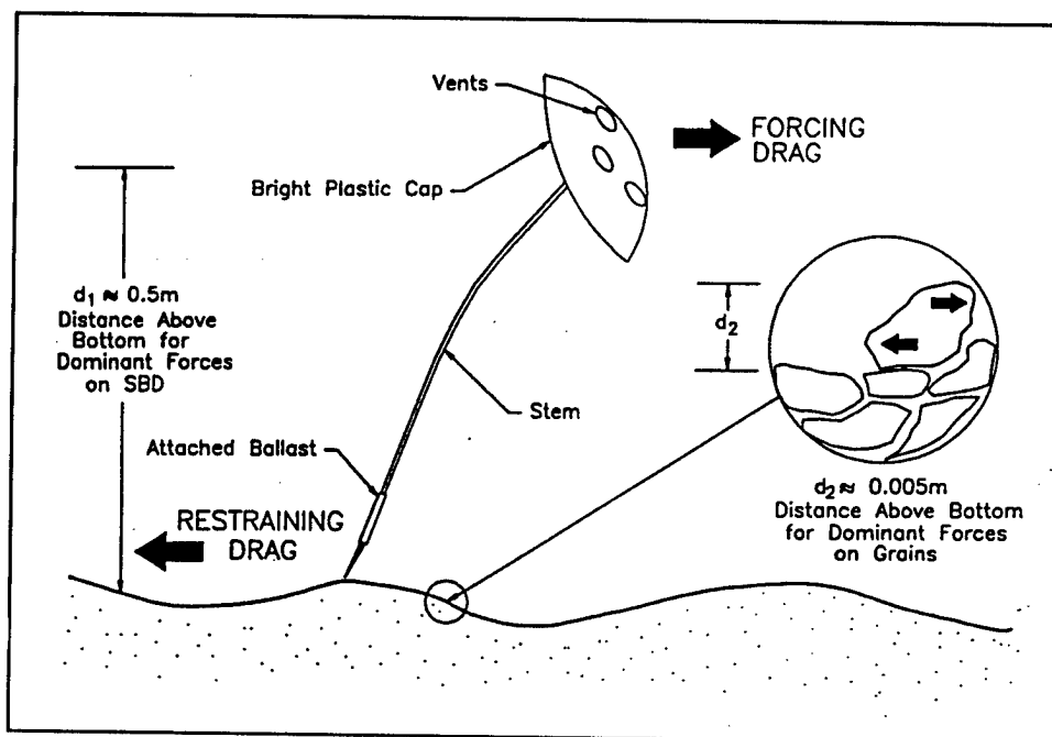
Figure 23. Differences in forces and scales on a seabed drifter and a sand grain
