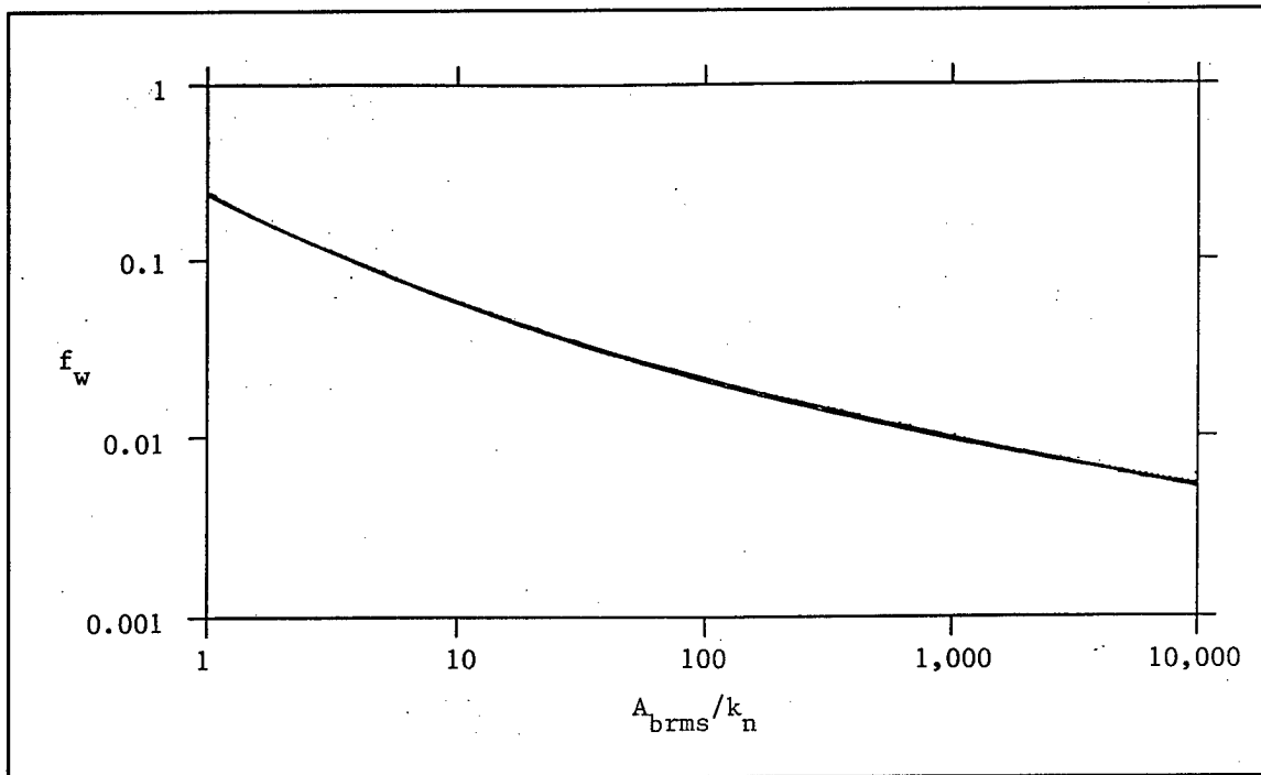
Figure 6. Movable-bed wave-friction factors for fully rough turbulent flow
