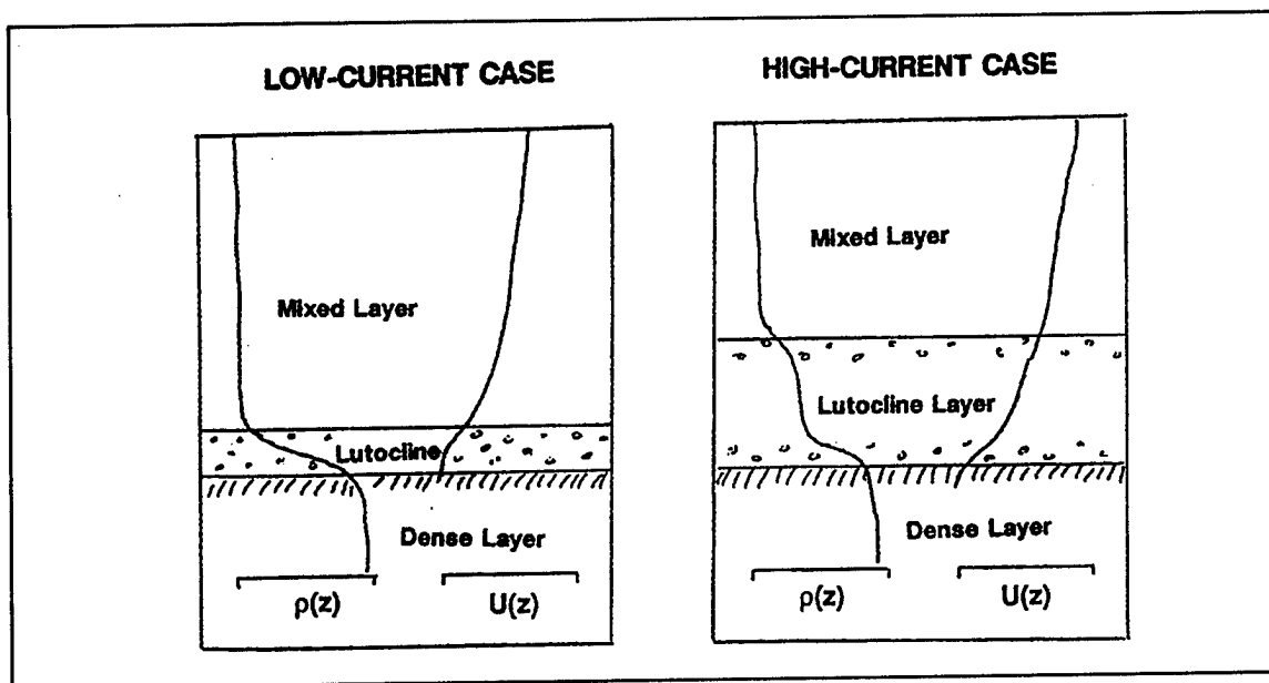
Figure 7. Vertical structure above a fluid-mud layer for low- and high-current conditions
