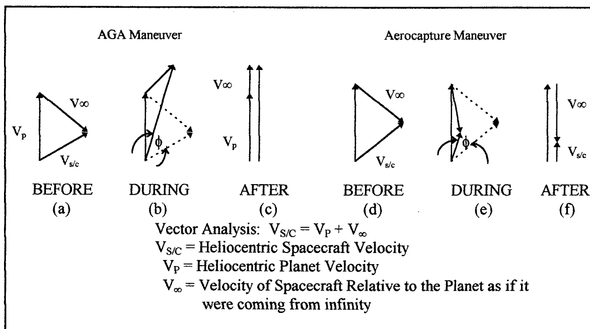
Figure 1.1 Aero-Gravity-Assist Maneuver
