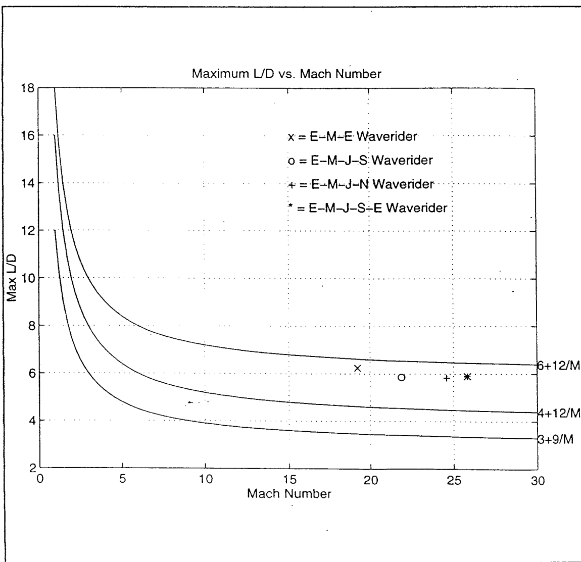
Figure 5.5 Kuchemann's Curve
