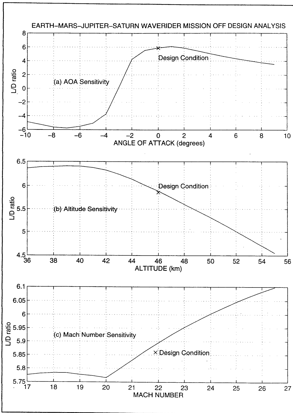
Figure 5.2 Off-Design Analysis for the Earth-Mars-Jupiter-Saturn Wayerider Mission
