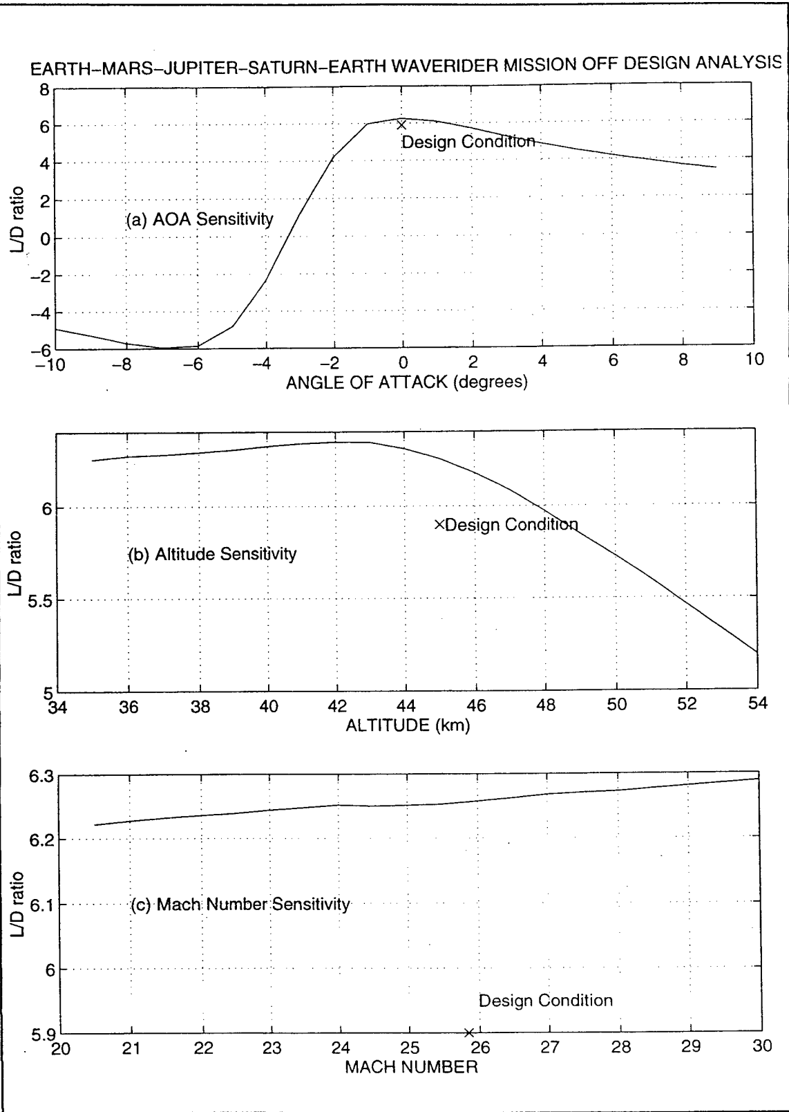
Figure 5.4 Off-Design Analysis for the Earth-Mars-Jupiter-Saturn-Earth Waverider Mission
