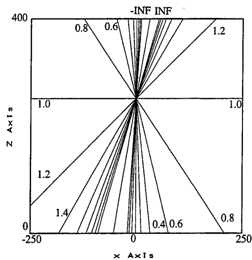
(b) x_0 = -50, x_{0e} = -50, \beta_f = 0.2
