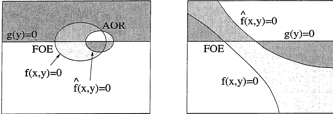
Figure 14: The geometry of the negative upper bound areas on the image plane represented by all the shaded areas in the figures. These are also the areas where the motion fields arising from the erroneous motion estimates must differ from the true motion fields or, equivalently, there exists some gradient direction along which the normal flows must be different.
