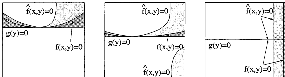
Figure 15: Diagram illustrating the areas where the the motion fields arising from the erroneous motion estimates must differ from the true motion field, for the case where W(x0_e, y0_e) = -\lambda(\beta_e, -\alpha_e) for some positive \lambda . The diagrams from left to right illustrate the change in these areas for increasingly small y0 . As can be seen, as y0 tends to zero, both f(x, y) = 0 and \hat{f}(x, y) = 0 degenerate into two pairs of intersecting lines.
