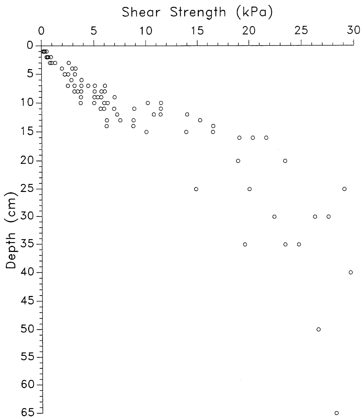
Figure 3.1.8 Depth profile of in-situ sediment shear strength.
