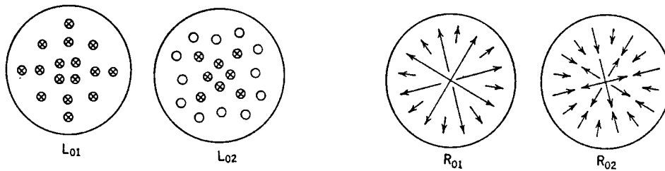
Schematic particle displacement patterns for the lowest order dilational modes of a circular rod at \beta = 0 .
