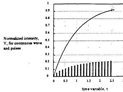
Graph of pulsed normalized intensities where pulse widths are 9.1% and 23% of the period
