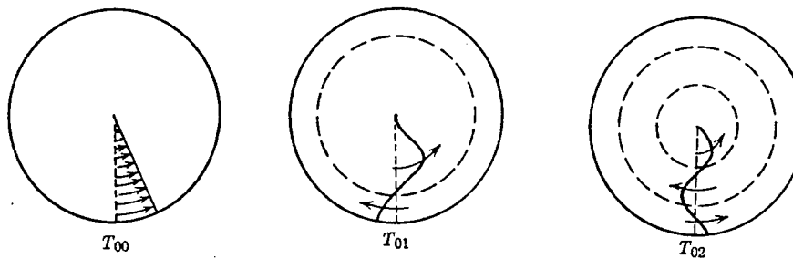
Particle velocity distributions for the three lowest order members of the torsional mode family T_{0q} .
