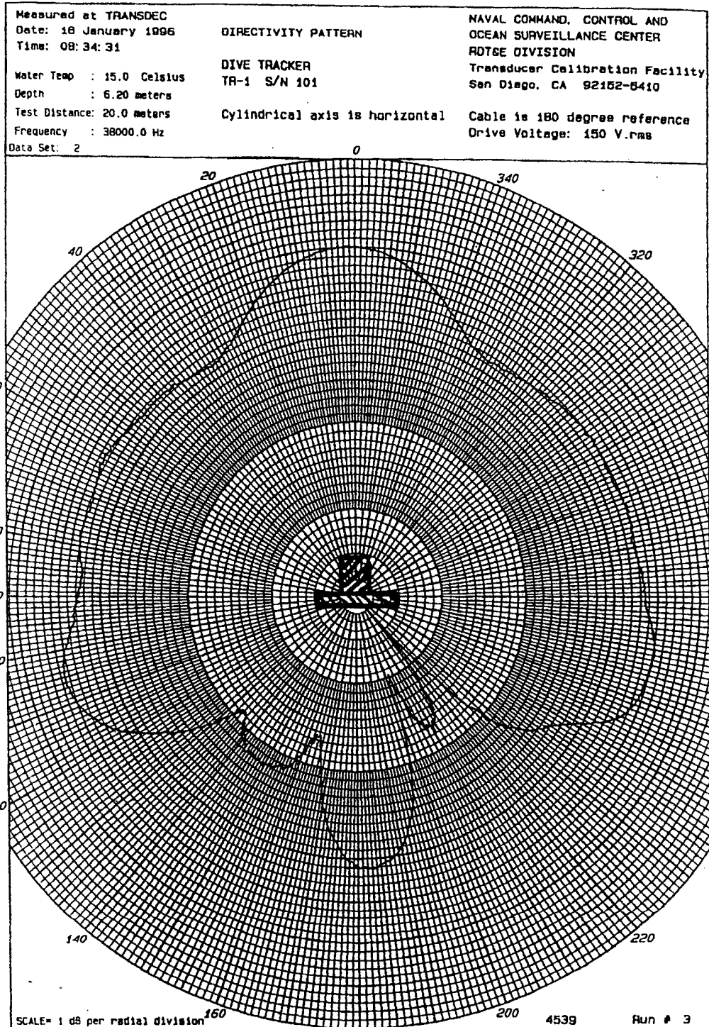
Figure 4. Transducer Beam Pattern.
