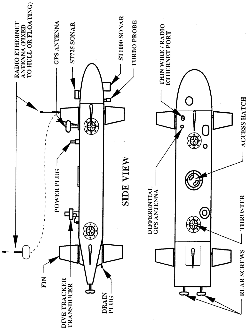
Figure 1. External Views of Phoenix AUV. DiveTracker transducer is mounted on the top. From [Marco].
