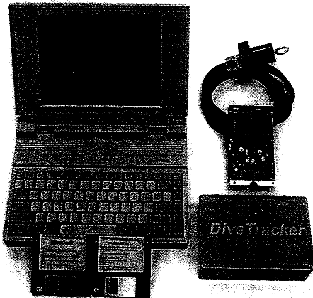
Figure 7. Surface Station computer with software, DT1-DRY electronics module, bare module for mounting in an AUV, and 40 kHz sonar transducer. From [Desert Star Systems].
