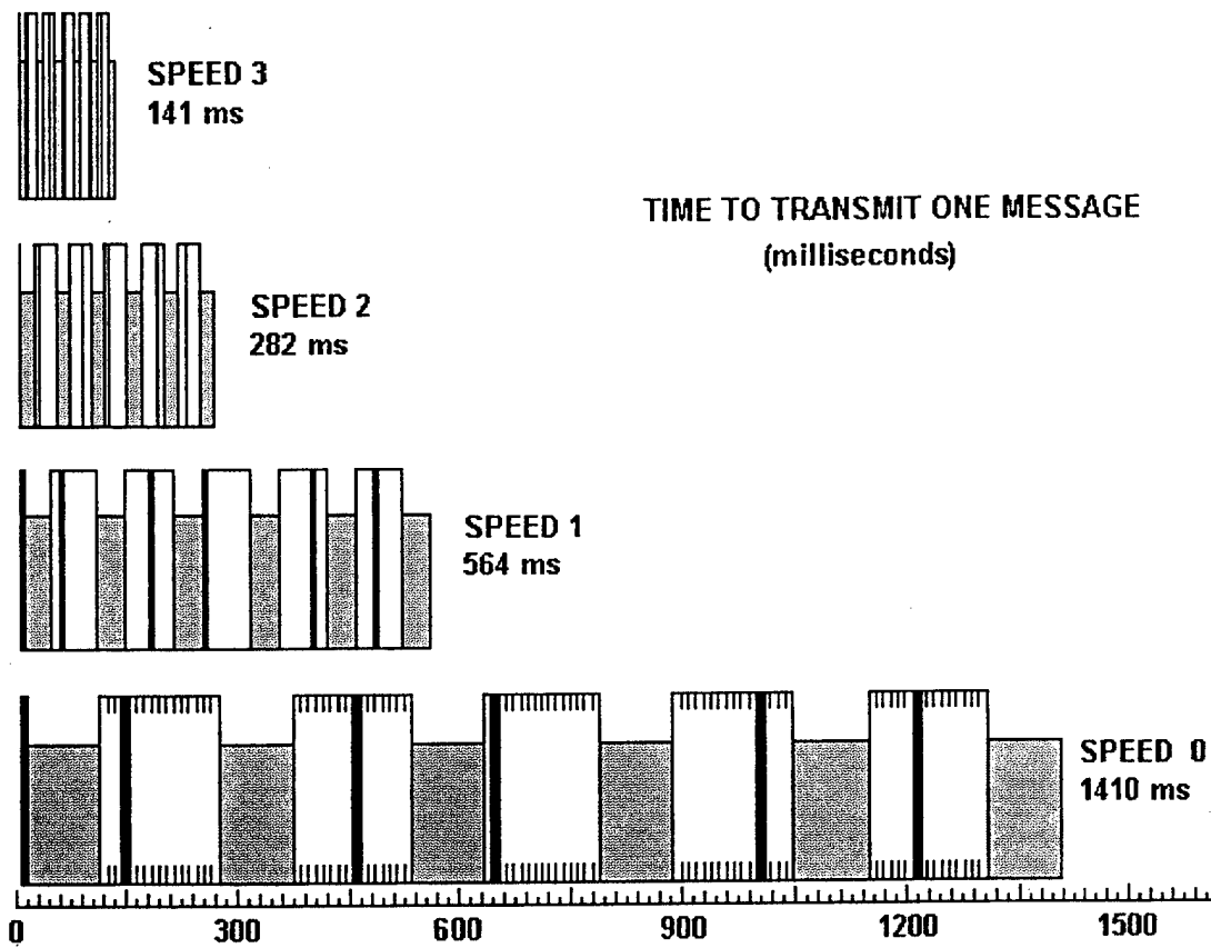
Figure 9. Communication Speed Comparison.
