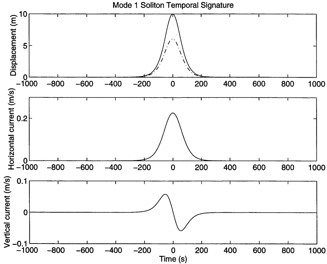
Figure 11. The evolution of modal displacement (top), horizontal current (middle) and vertical current (bottom) associated with a single soliton. The soliton temporal structure (solid lines) was calculated based on weakly non-linear theory. The dot-dashed line in the top panel represents the result of linearization, showing large error.
