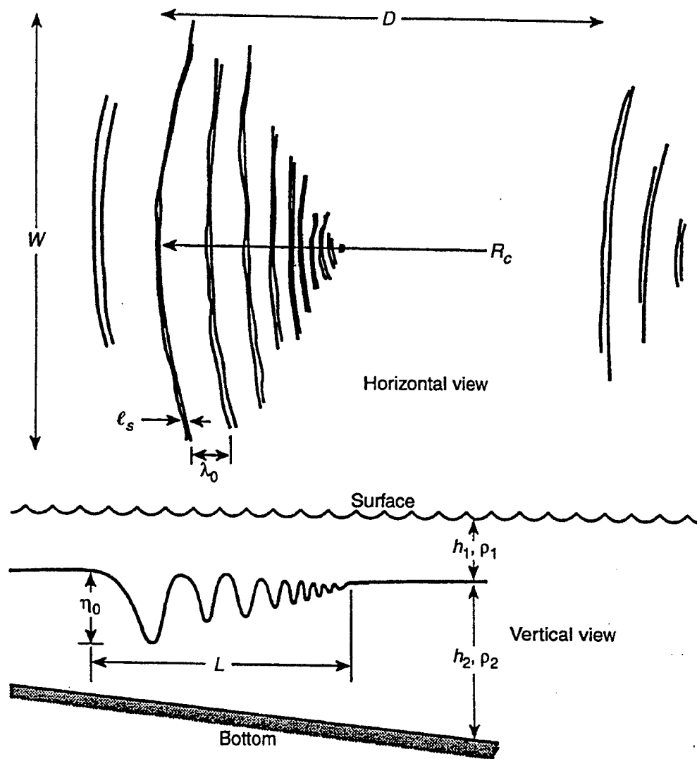
Figure 3 Schematic plan view and profile of soliton waves (from Apel 1995).
