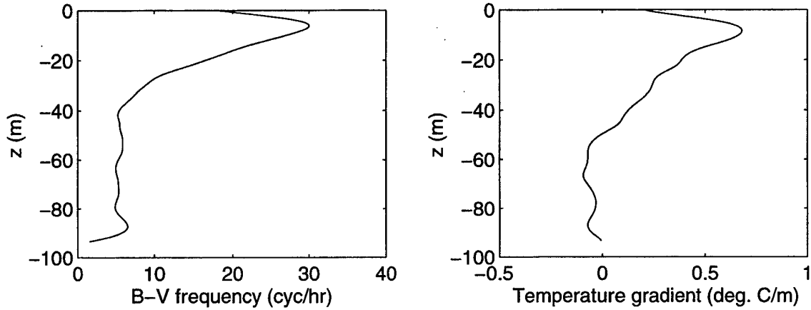
Figure 6. A Brunt-Vaisala frequency profile (left) and a temperature gradient profile (right). Both profiles are derived from a CTD cast taken between the two ADCP sites with some smoothing.
