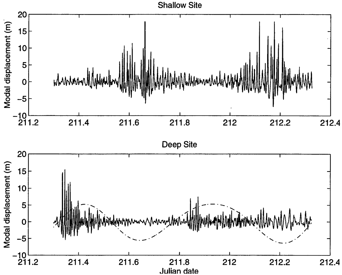
Figure 14. A segment of highpass time-series of modal displacements, at the Shallow (top) and Deep (bottom) Sites. The upslope barotropic tidal current (dot-dashed line in units of cm/s) is superimposed to show that this segment encompasses two tidal cycles with strong soliton packets generated near the Deep Site during the tidal flood.
