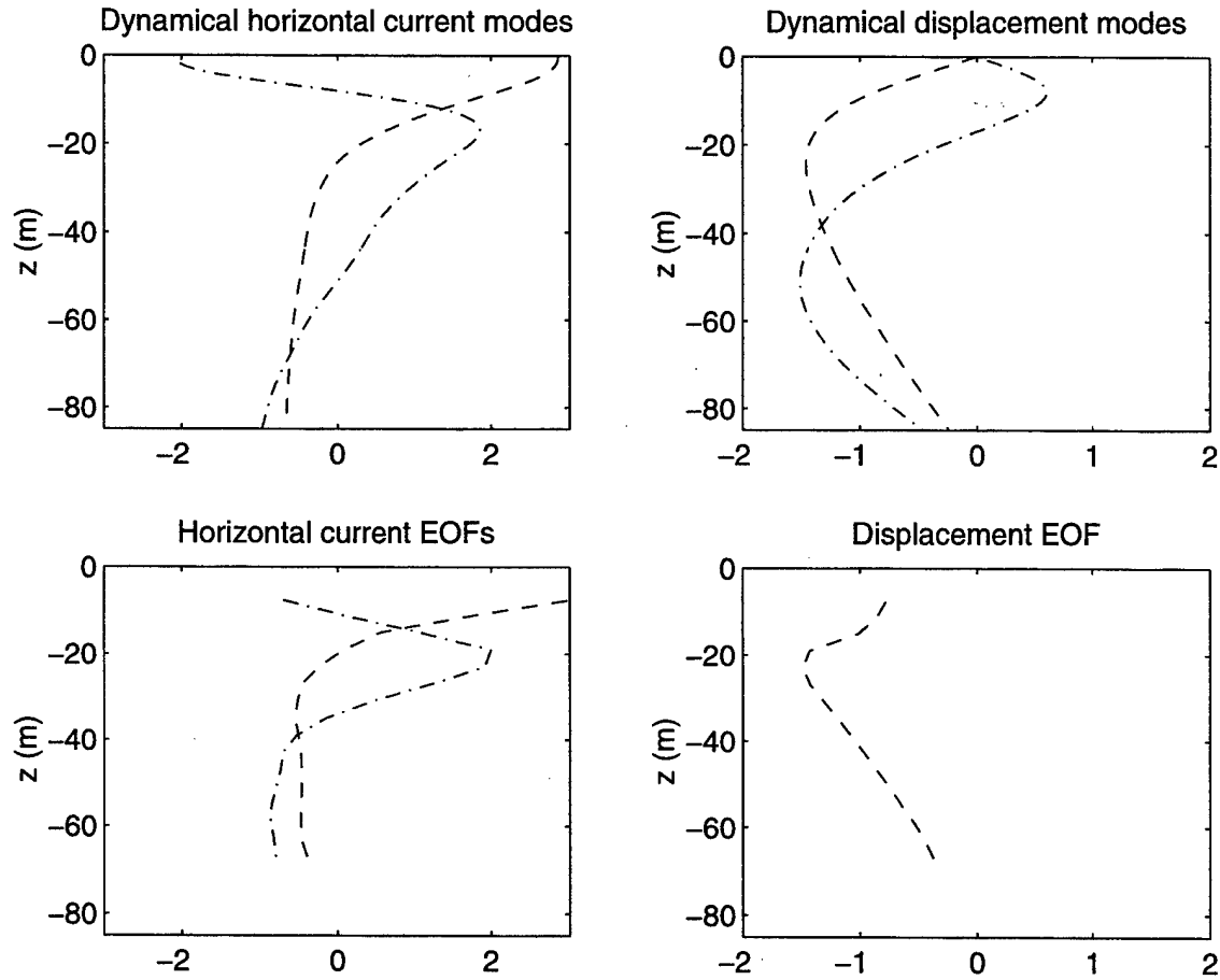
Figure 5. Vertical structure of currents (left panels) and displacements (right panels). Dynamical modes calculated based on an observed buoyancy profile are shown on the top panels whereas the vertical empirical orthogonal functions derived from the ADCP data are shown on the bottom panels for comparison. First baroclinic mode is denoted by dashed lines and second mode by dot-dashed lines. The zeroth barotropic mode is not shown.
