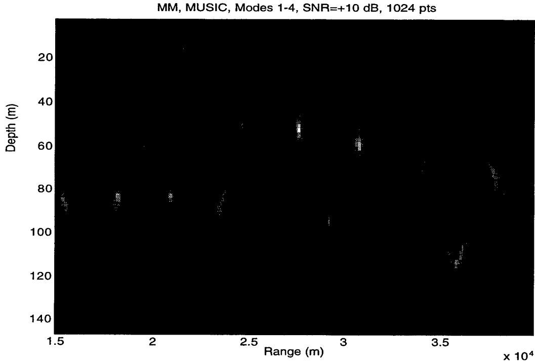
Figure 26: Data from 1st transmission ( M1=0.46 ; M2=0.015 ; M3=0.026 )
