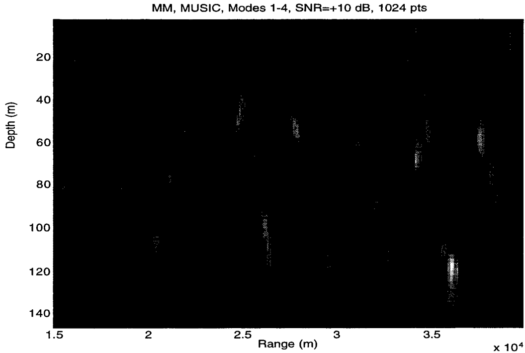
Figure 24: Pseudo-inverse mode filter ( M1=1.7 ; M2=0.013 ; M3=0.020 )
