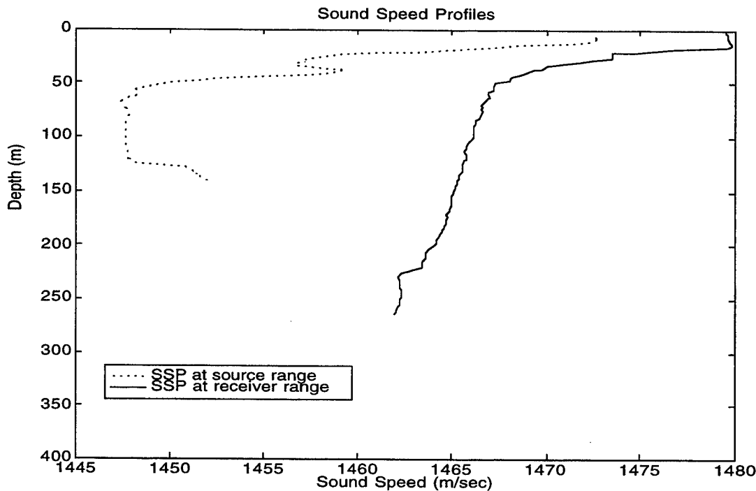
Figure 8: Sound Speed Profiles
