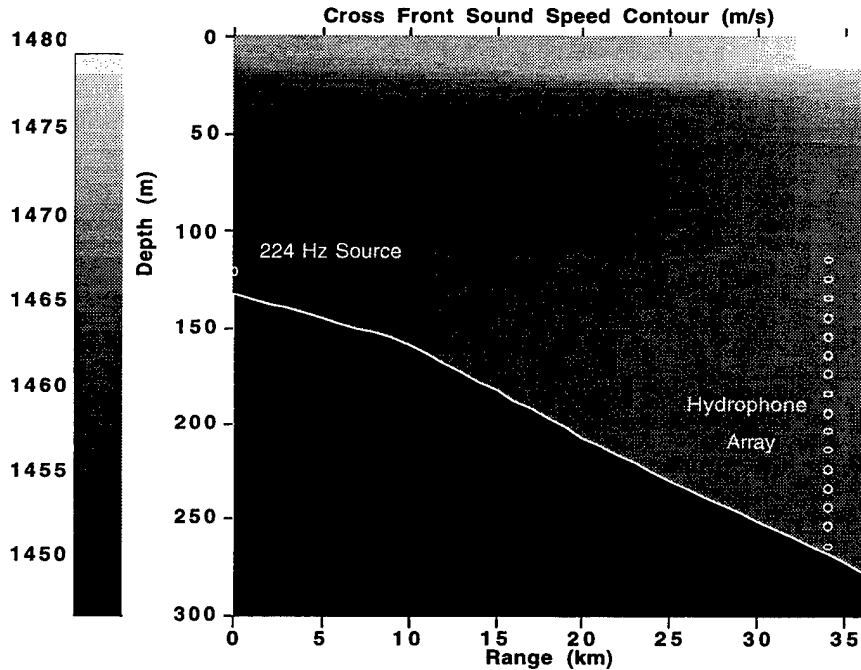
Figure 7: Sound speed field and bathymetry
