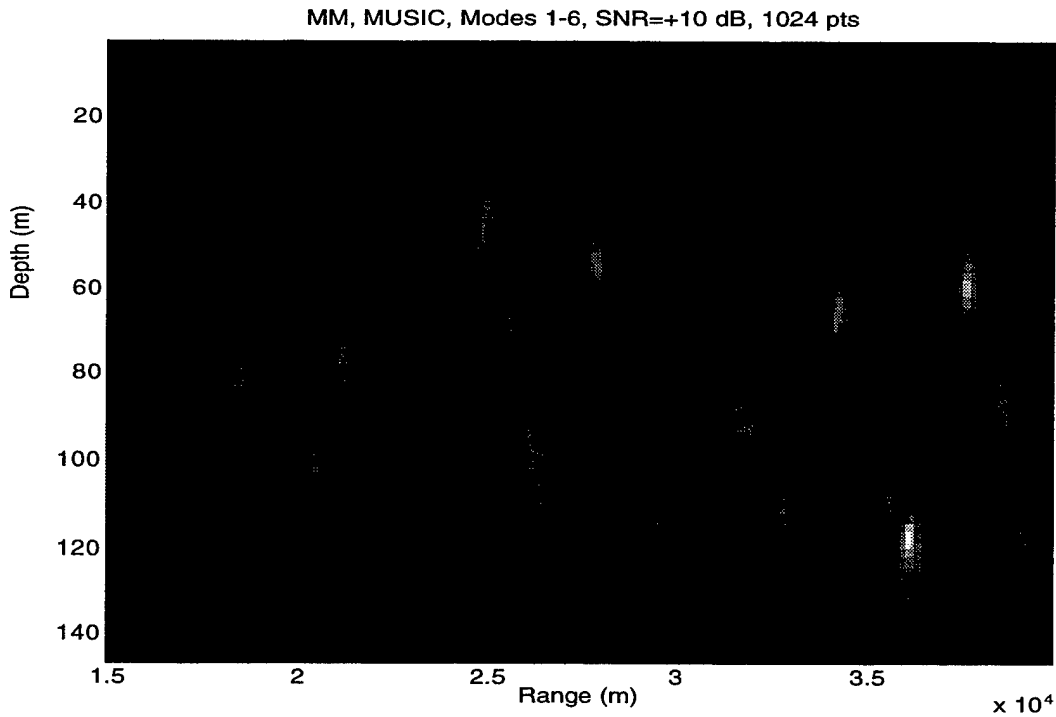
Figure 29: Modes 1-6 (M1=1.3; M2=0.011; M3=0.018)
