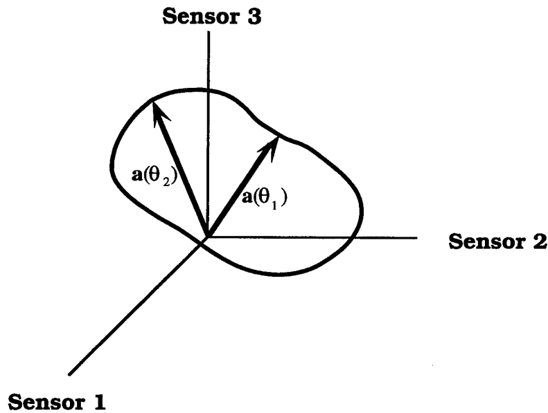
Figure 4: Array manifold
