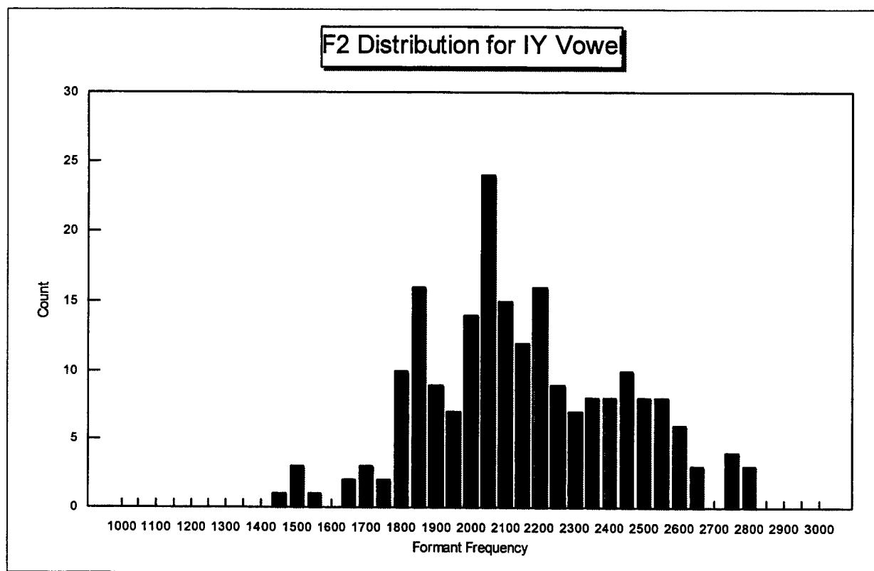
Figure 4.4. Distribution of F2 frequencies (IY vowel) before normalization.
