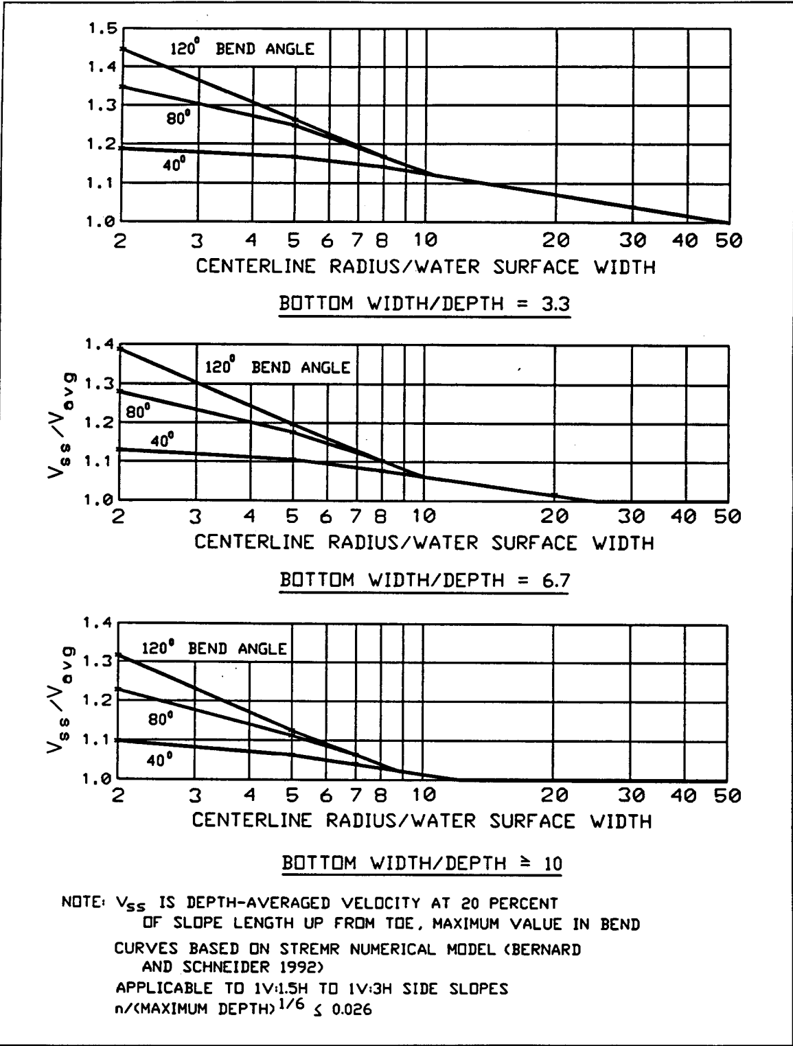
Figure 18. Riprap design velocities, trapezoidal channel
